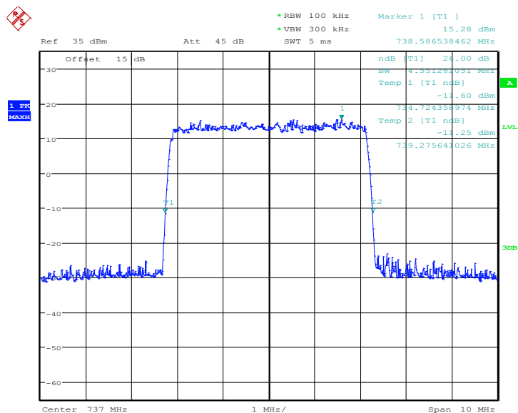
Output DL 1S M AWGN AGC+3dB 26dB Bandwidth
