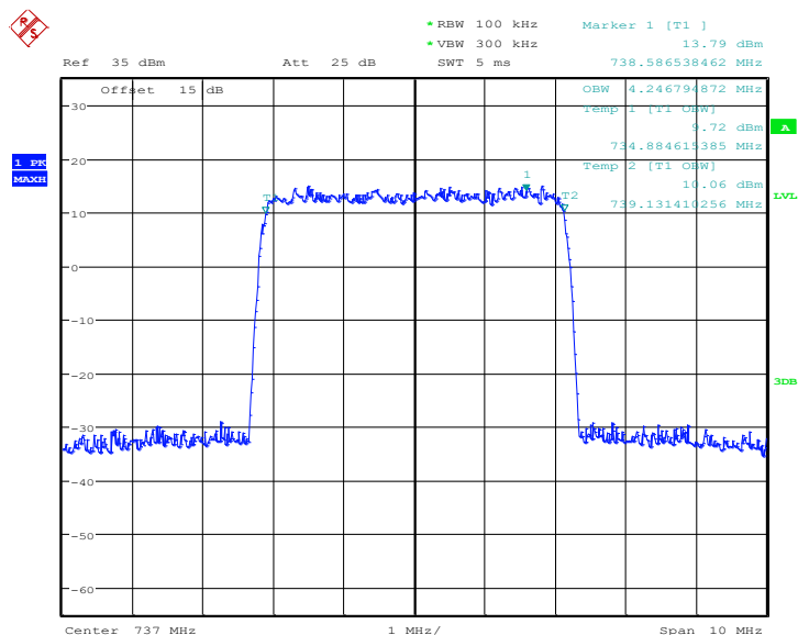
Output DL 1S M AWGN AGC+3dB 99% OBW
