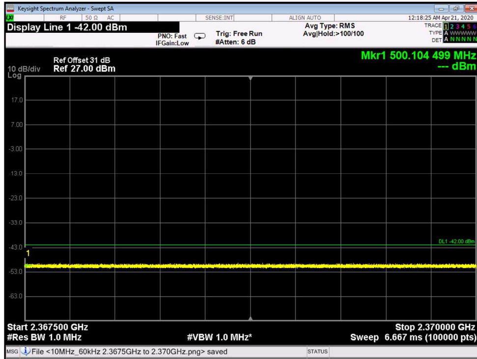
Figure 91: Spurious Emissions at Antenna Terminal 256QAM, 2355.0MHz, B.W. 10MHz, Sub Carrier 15kHz
