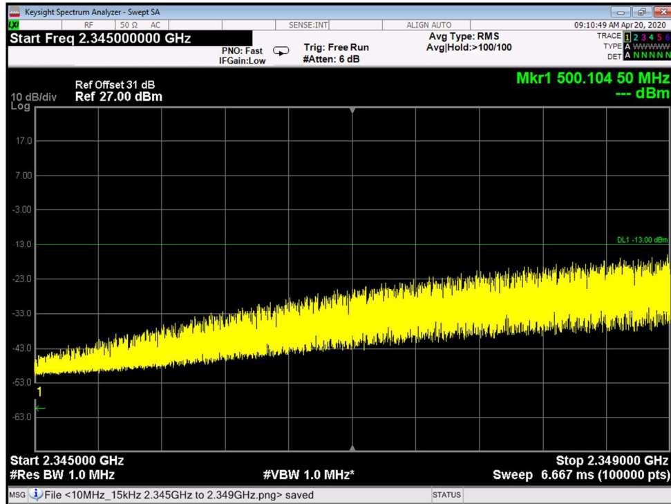
Figure 95: Spurious Emissions at Antenna Terminal 256QAM, 2355.0MHz, B.W. 10MHz, Sub Carrier 30kHz
