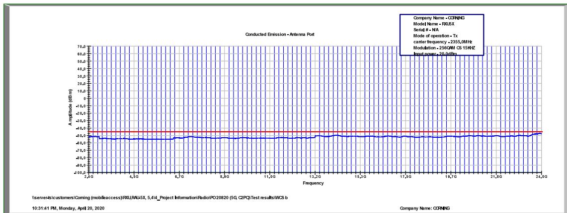
Figure 92: Spurious Emissions at Antenna Terminal 256QAM, 2355.0MHz, B.W. 10MHz, Sub Carrier 15kHz
