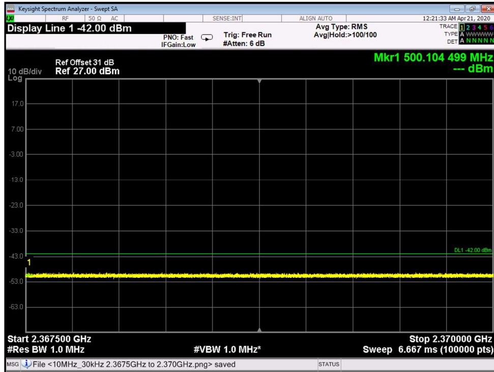
Figure 107: Spurious Emissions at Antenna Terminal 256QAM, 2355.0MHz, B.W. 10MHz, Sub Carrier 60kHz
