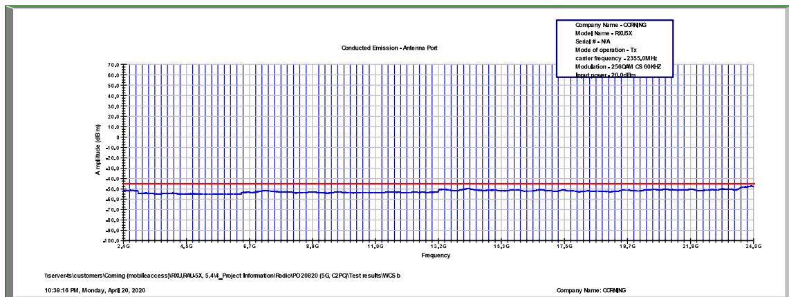
Figure 108: Spurious Emissions at Antenna Terminal 256QAM, 2355.0MHz, B.W. 10MHz, Sub Carrier 60kHz
