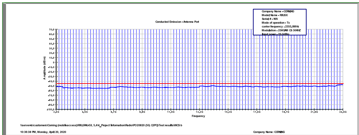
Figure 100: Spurious Emissions at Antenna Terminal 256QAM, 2355.0MHz, B.W. 10MHz, Sub Carrier 30kHz
