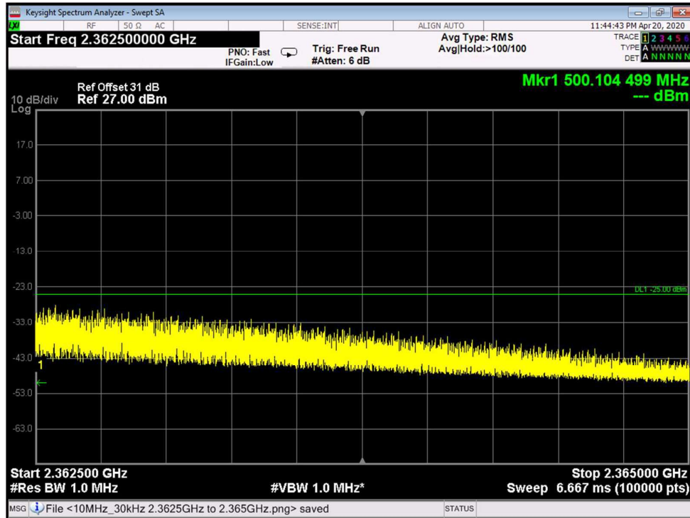
Figure 105: Spurious Emissions at Antenna Terminal 256QAM, 2355.0MHz, B.W. 10MHz, Sub Carrier 60kHz
