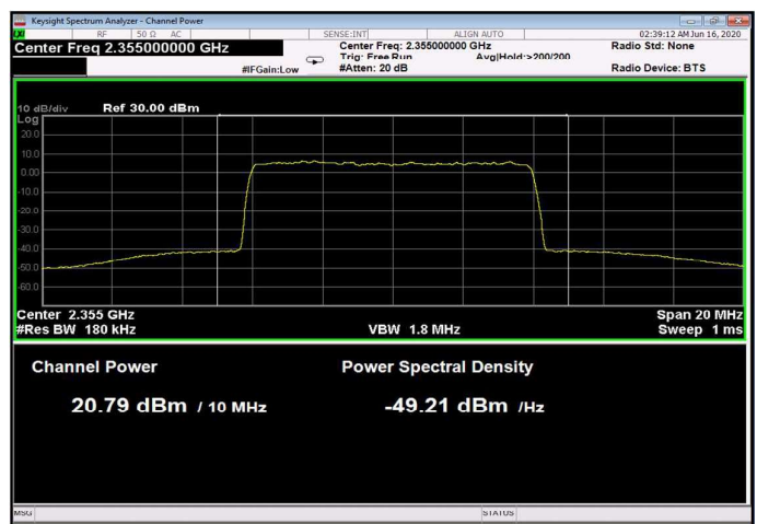
Figure 14: 64QAM 10MHz C.S.; 2355.0MHz, 60kHz
