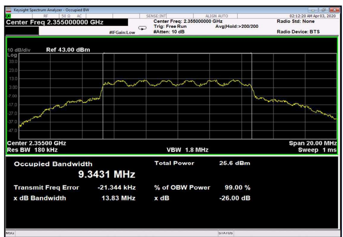
Figure 27: 16QAM 10MHz B.W.; 2355.0MHz, 15kHz Output
