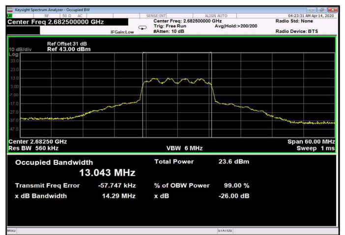
Figure 320: 16QAM 15MHz B.W.; 2682.5MHz, 60kHz Output
