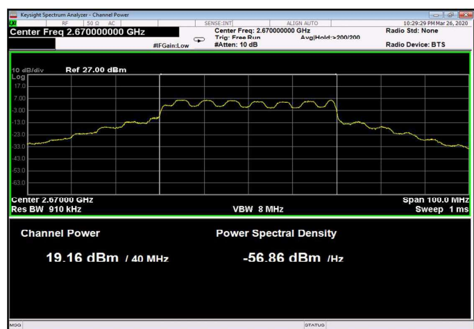
Figure 48: 16QAM 40MHz B.W.; 2670.0MHz, 15kHz
