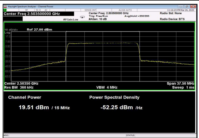
Figure 72: 64QAM 15MHz B.W.; 2503.5MHz, 15kHz
