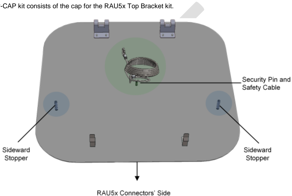
Figure 4-14. BR-TOP-CAP
