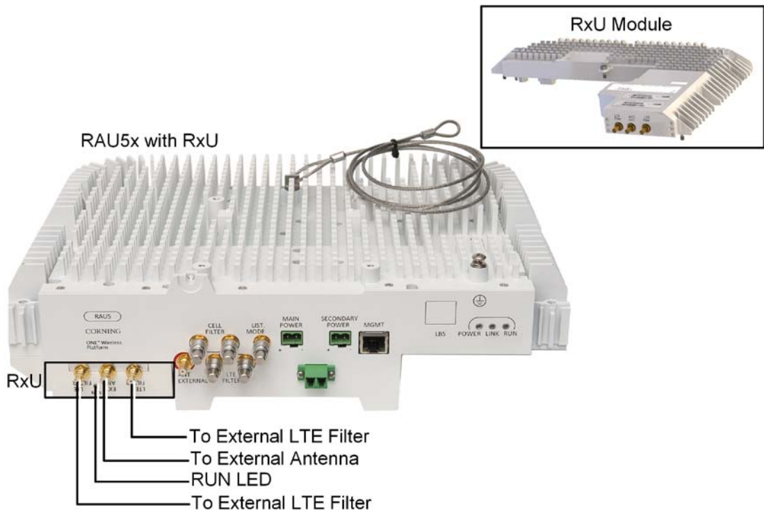
Figure 2-2. RxU Interfaces
