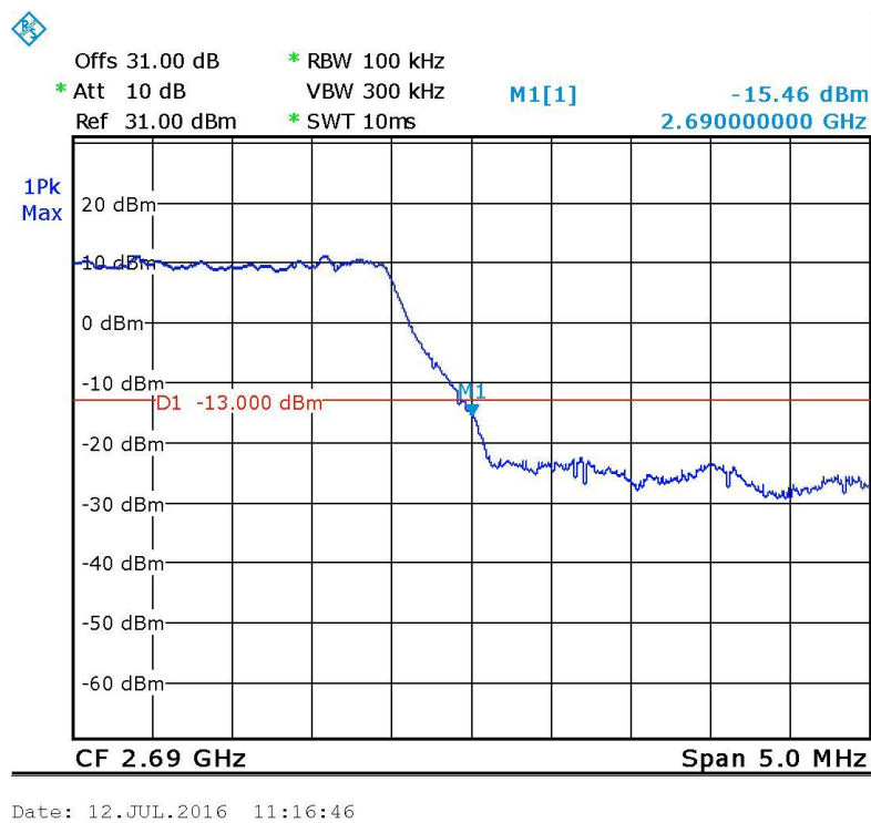
Figure 68. — Band Edge – High, QPSK
