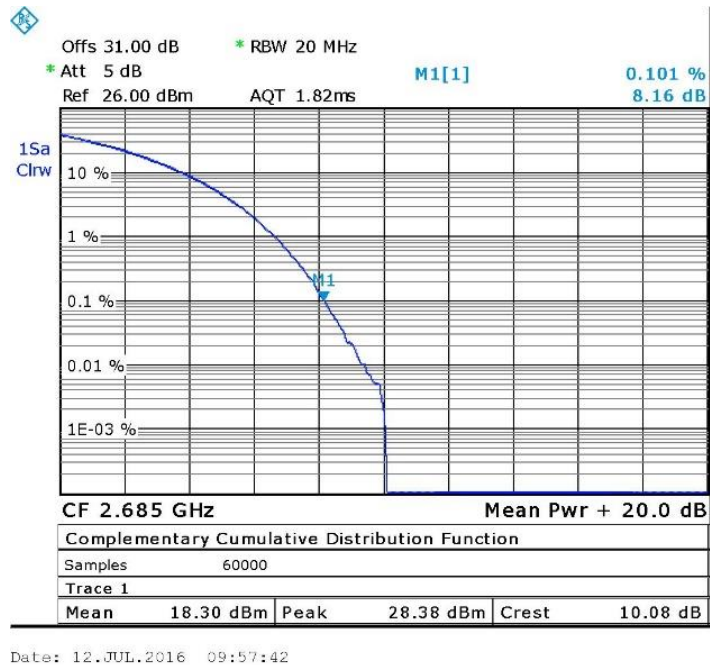
Figure 27. — 16QAM, 2685.0 MHz
