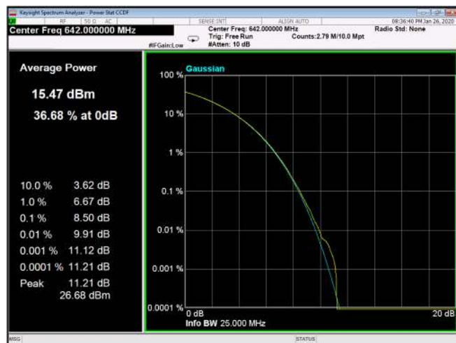
Figure 250: 16QAM 15MHz B.W; 642.0MHz, 60kHz
