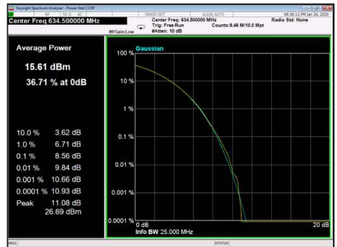
Figure 252: 16QAM 20MHz B.W; 634.5MHz, 15kHz
