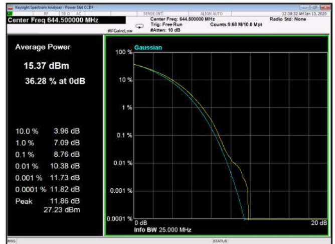
Figure 281: 64QAM 15MHz B.W; 644.5MHz, 15kHz
