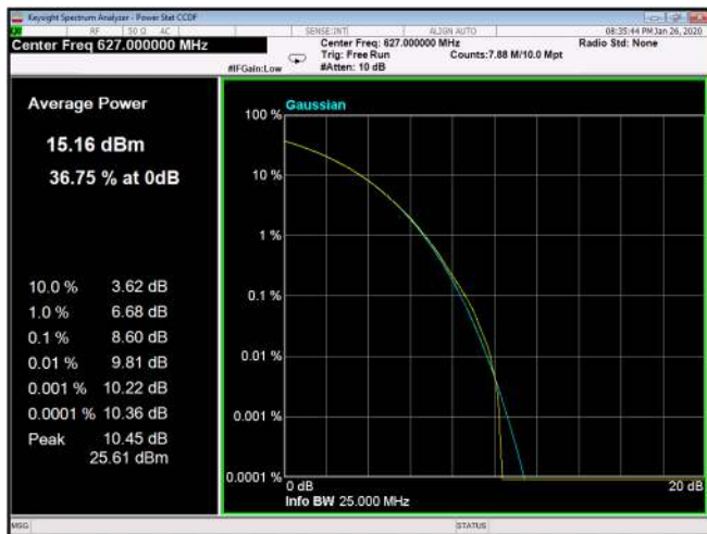
Figure 251: 16QAM 20MHz B.W; 627.0MHz, 15kHz
