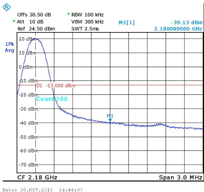
Figure 105. — GSM 2178.8 MHz
