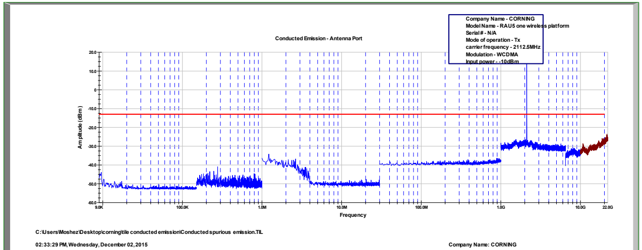
Figure 97 Spurious Emissions at Antenna Terminals WCDMA, 2112.5MHz
