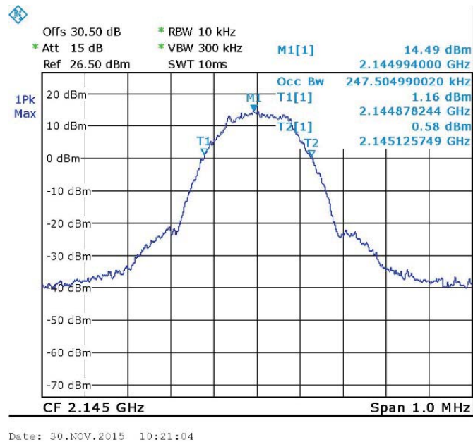
Figure 81. — GSM (2145.0 MHz) OUT
