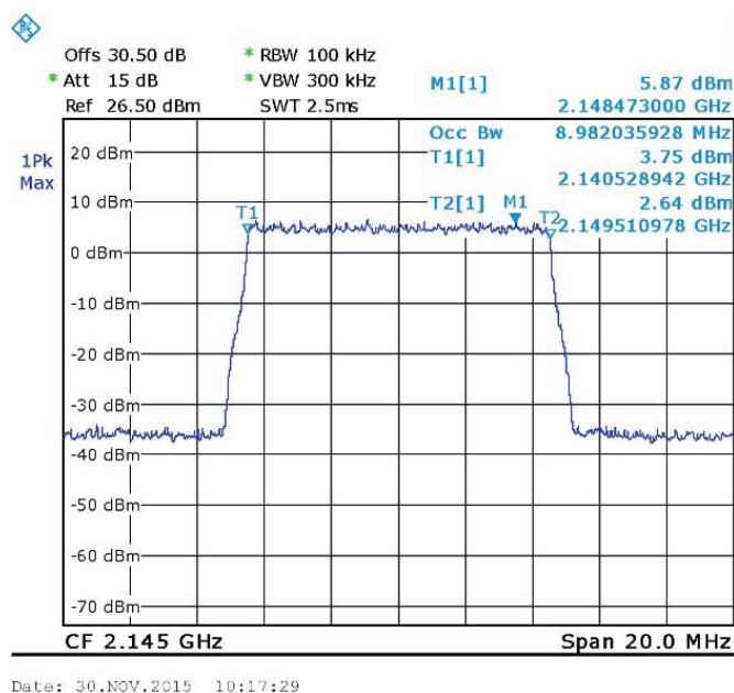
Figure 74. — LTE 64QAM (2145.0 MHz) IN
