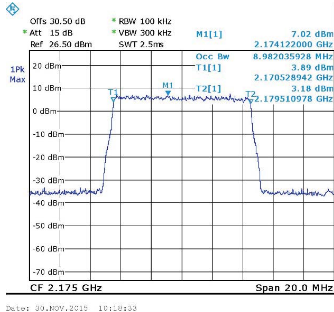
Figure 77. — LTE 64QAM (2175.0 MHz) OUT
