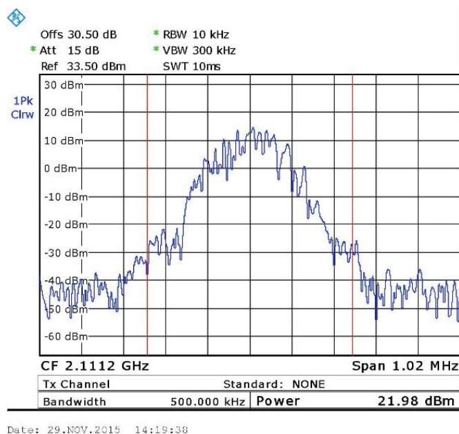
Figure 64. — GSM (2111.2 MHz)
