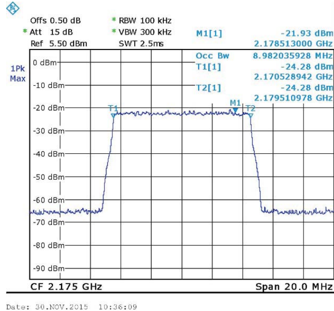
Figure 76. — LTE 64QAM (2175.0 MHz) IN
