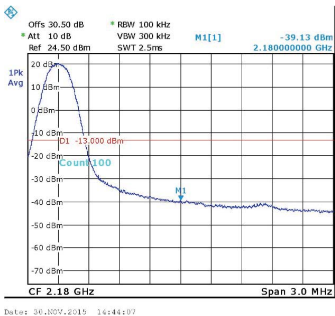
Figure 105. — GSM 2178.8 MHz
