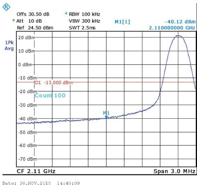
Figure 104. — GSM 2111.2 MHz
