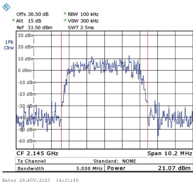
Figure 68. — WCDMA (2145.0 MHz)
