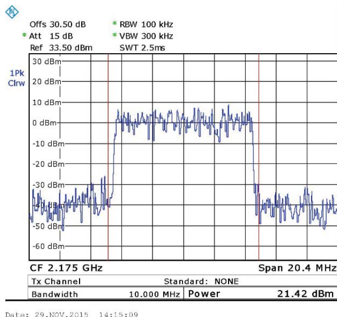
Figure 63. — LTE 64QAM (2175.0 MHz)
