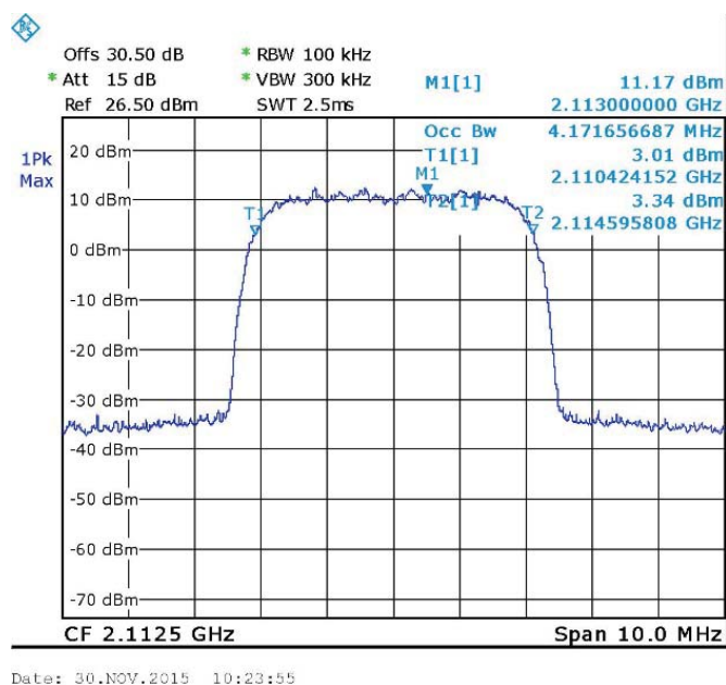
Figure 85. — WCDMA (2112.5 MHz) OUT
