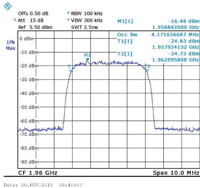
Figure 124. WCDMA- 1960.0 MHz Input
