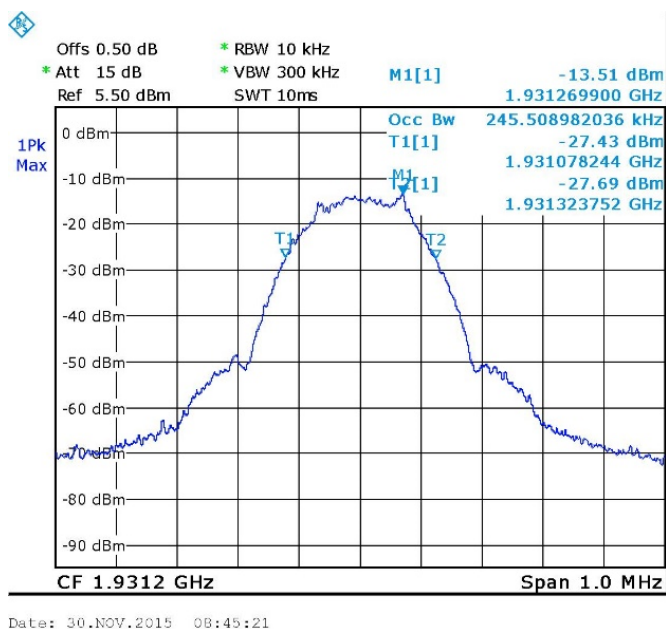
Figure 116. GSM - 1931.2 MHz Input
