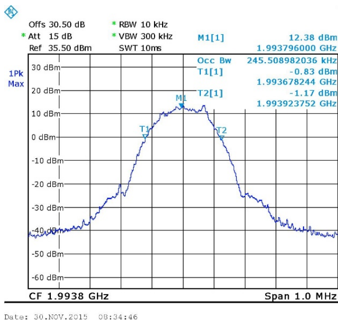
Figure 121. GSM - 1993.8 MHz Output
