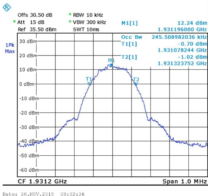
Figure 117. GSM - 1931.2 MHz Output
