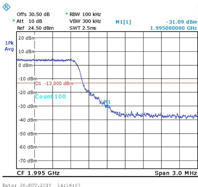
Figure 141— LTE 64QAM - 1990.0 MHz
