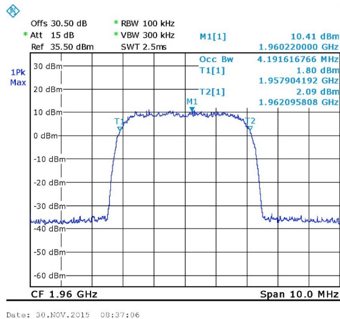
Figure 125. WCDMA - 1960.0 MHz Output
