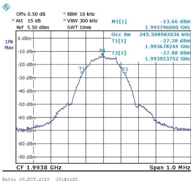
Figure 120. GSM - 1993.8 MHz Input
