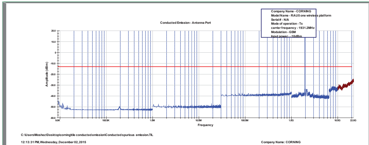
Figure 132 GSM - 1931.2 MHz
