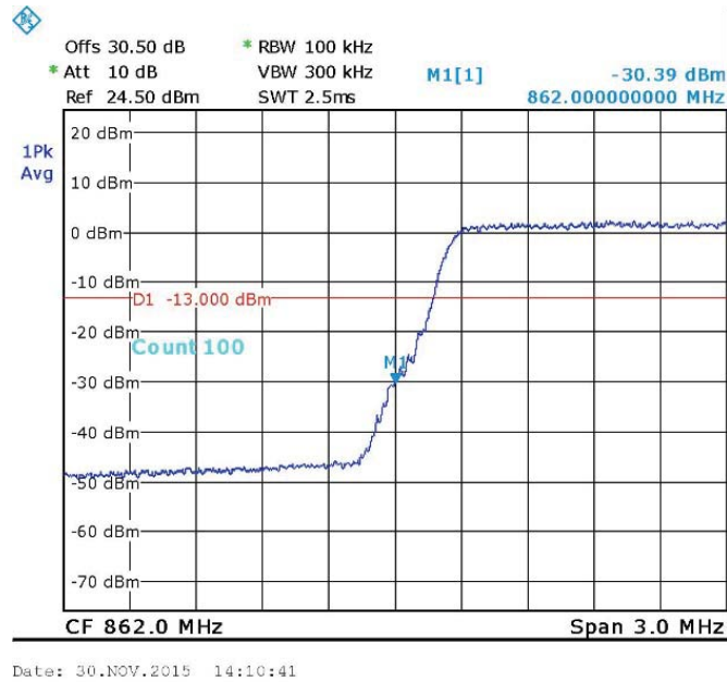
Figure 89— LTE 64QAM - 864.5MHz
