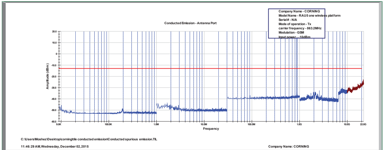
Figure 83. GSM - 863.2 MHz
