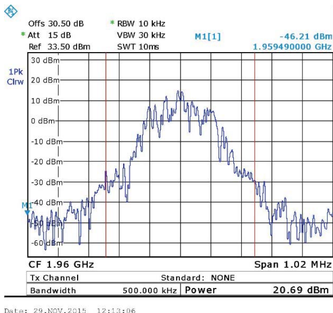
Figure 103. GSM - 1960.0 MHz
