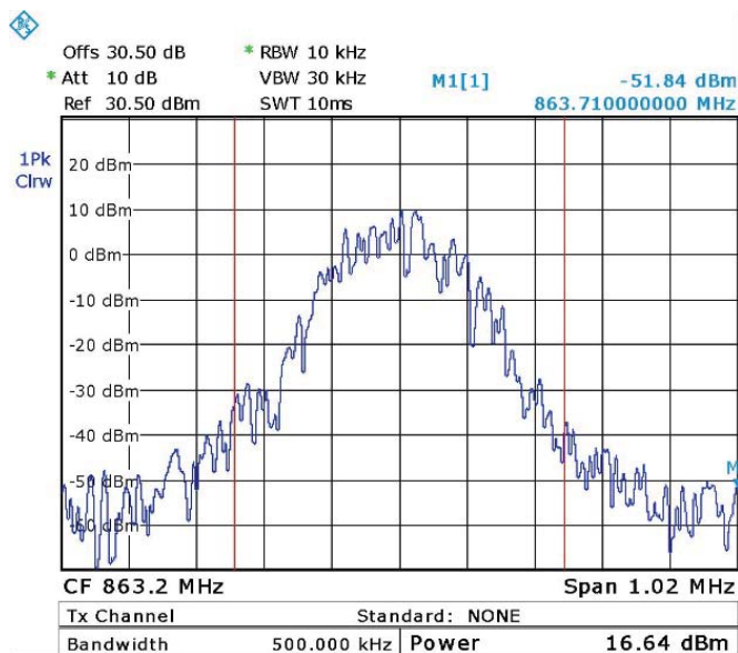
Figure 62. GSM - 863.2 MHz
