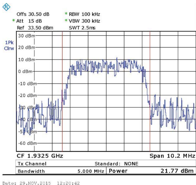
Figure 105.WCDMA - 1932.5 MHz
