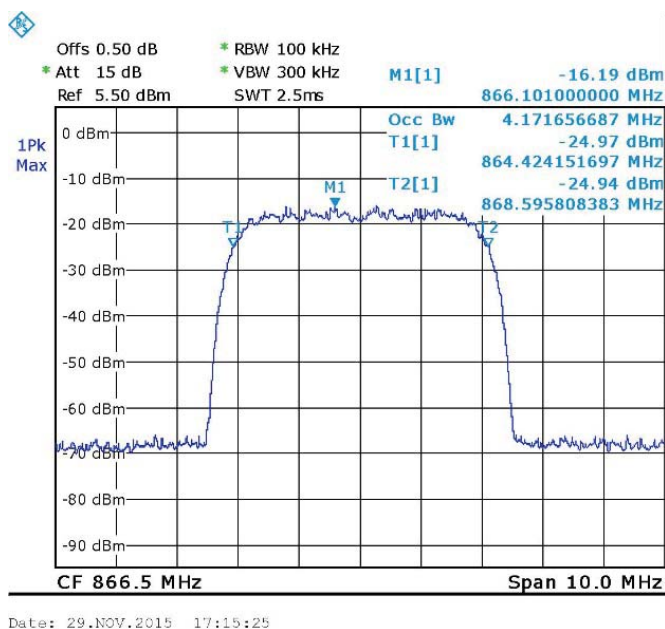
Figure 78. WCDMA - 866.5MHz Input
