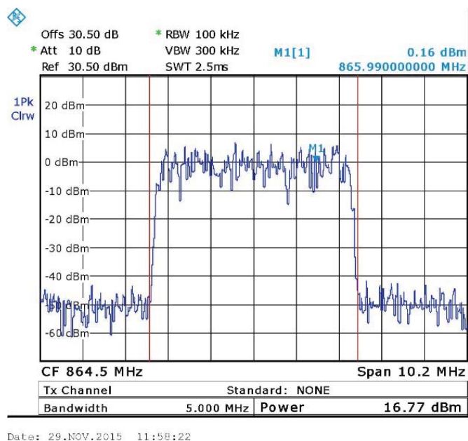
Figure 60. LTE 64QAM - 864.5 MHz
