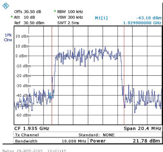
Figure 99. 64QAM - 1935.0 MHz
