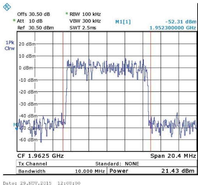
Figure 100. 64QAM - 1962.5 MHz
