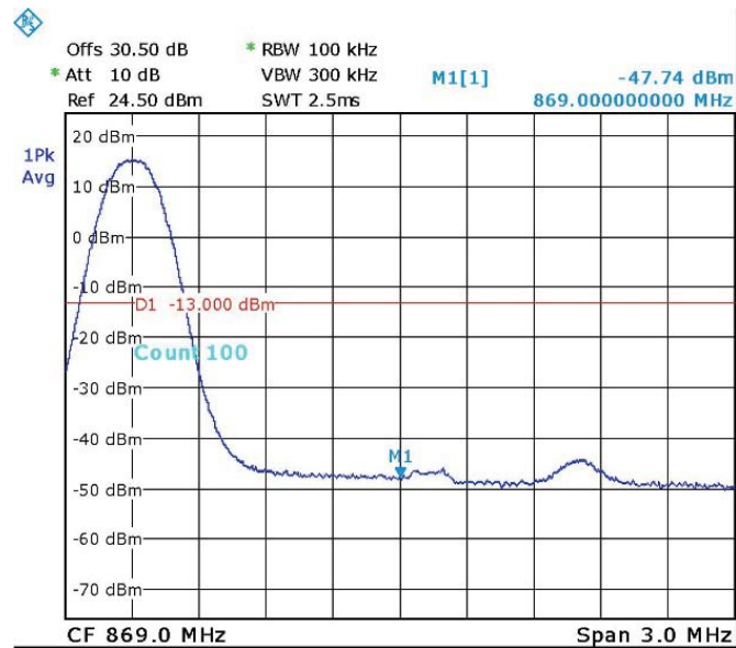
Figure 92—GSM - 867.8 MHz
