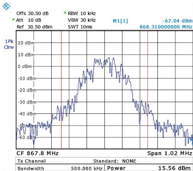
Figure 63. GSM - 867.8 MHz
