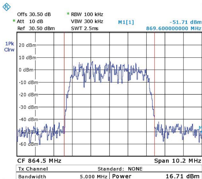
Figure 64. WCDMA - 864.5 MHz
