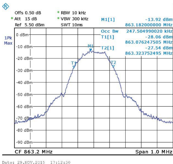
Figure 72. GSM - 863.2MHz Input
