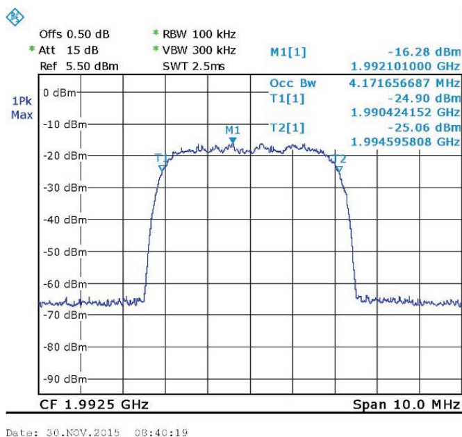
Figure 126. WCDMA - 1992.5 MHz Input
