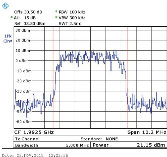
Figure 107. WCDMA - 1992.5 MHz
