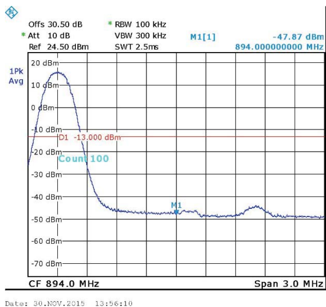
Figure 53. GSM - 892.8 MHz
