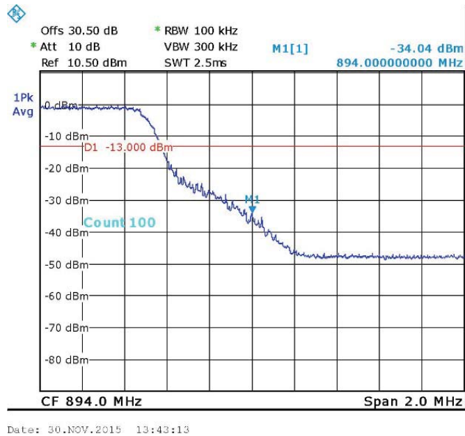
Figure 51. LTE 64QAM - 889.0 MHz
