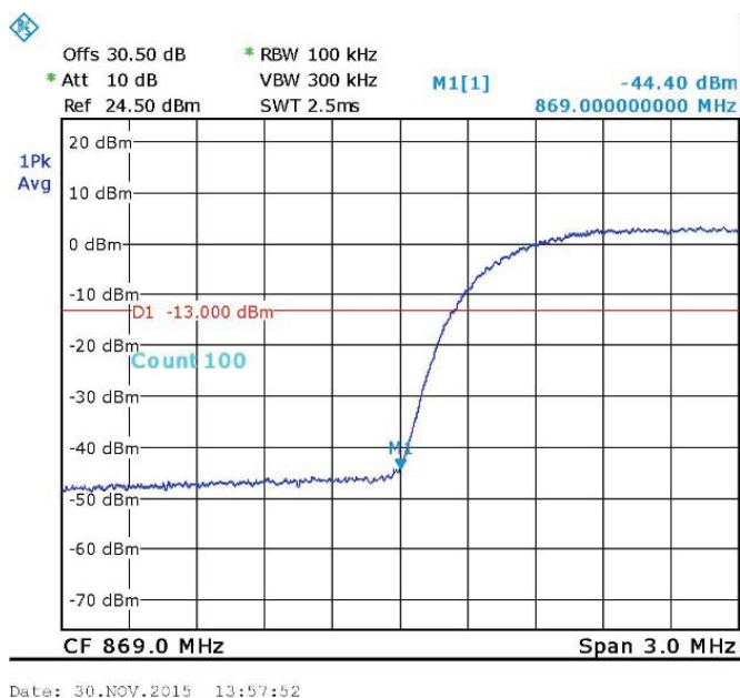
Figure 54. WCDMA - 871.5 MHz
