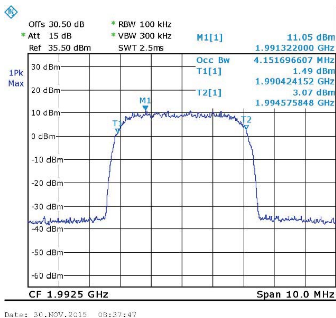
Figure 127. WCDMA - 1992.5 MHz Output
