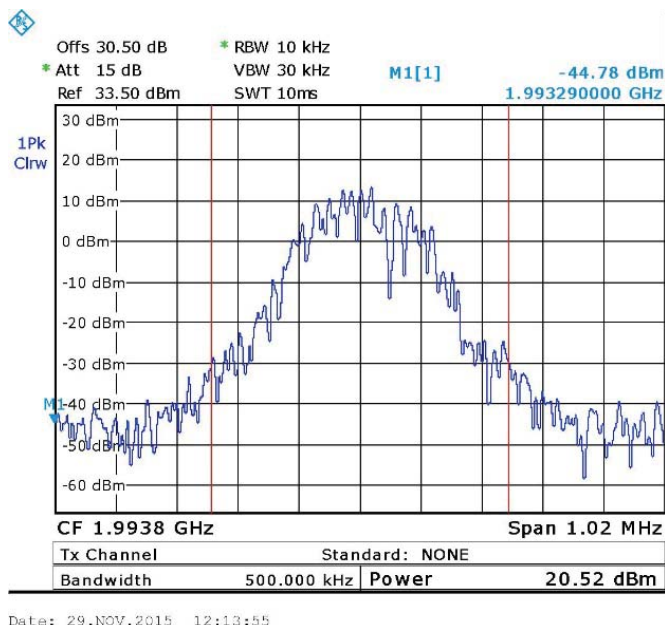
Figure 104. GSM - 1993.8 MHz
