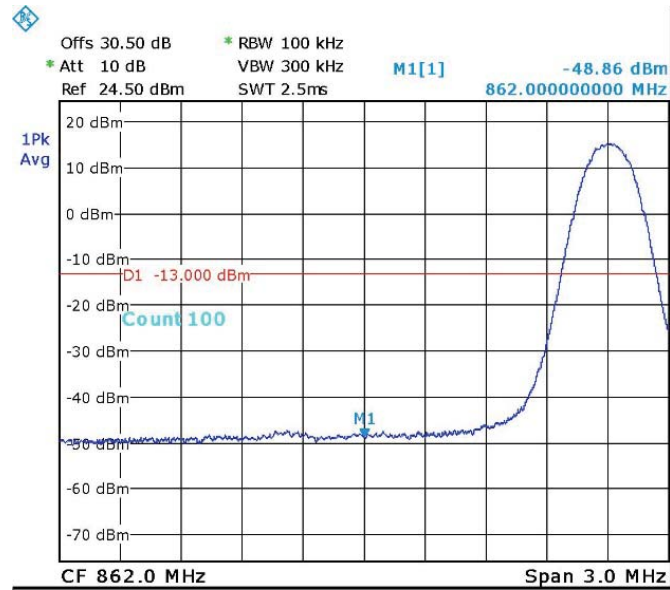
Figure 91—GSM - 863.2MHz
