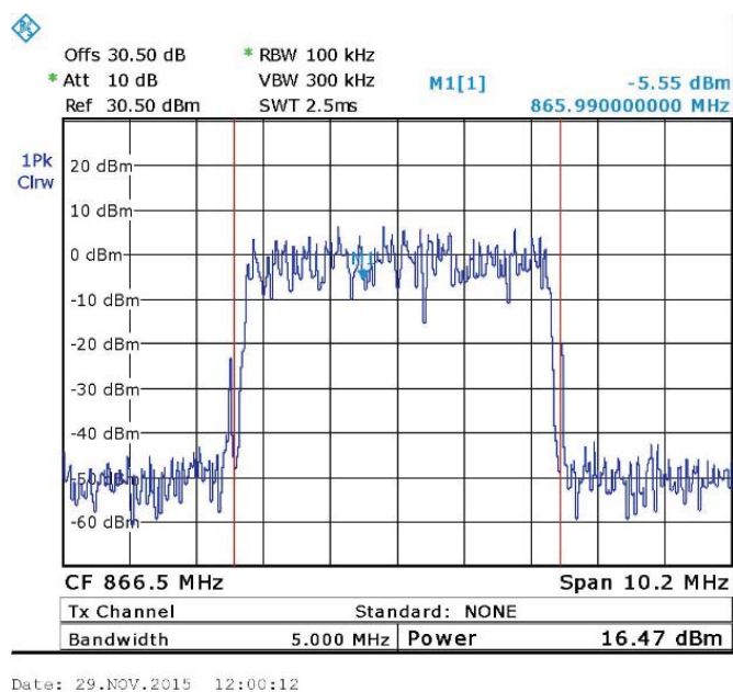
Figure 61. LTE 64QAM - 866.5 MHz
