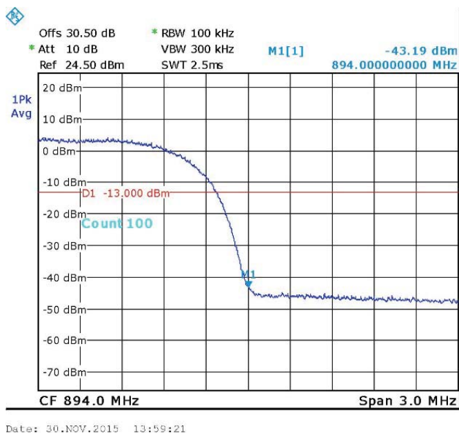
Figure 55. WCDMA - 891.5 MHz
