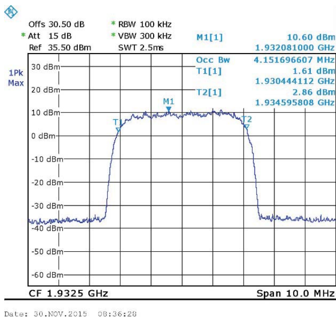
Figure 123. WCDMA - 1932.5 MHz Output
