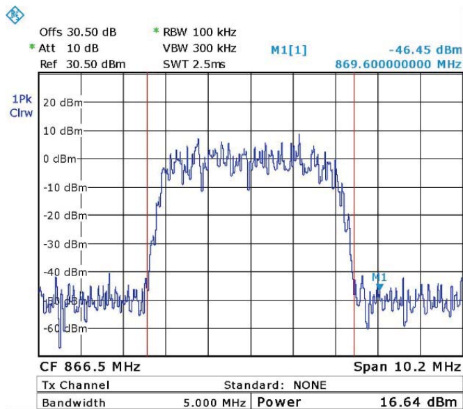
Figure 65. WCDMA - 866.5 MHz
