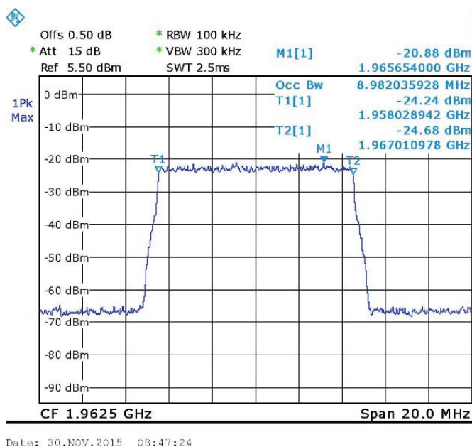
Figure 112.LTE 64QAM - 1962.5 MHz Input
