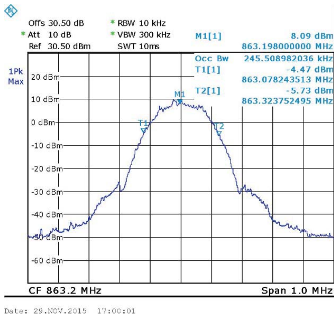
Figure 73. GSM - 863.2MHz Output
