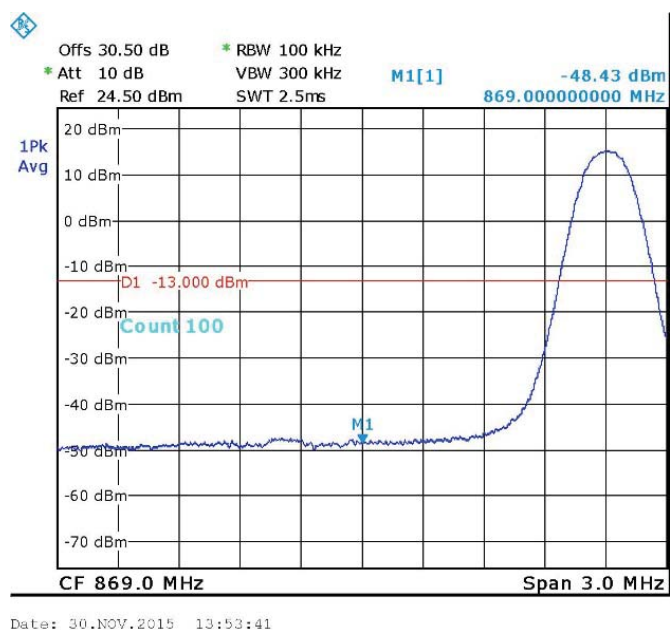
Figure 52. GSM - 870.2 MHz
