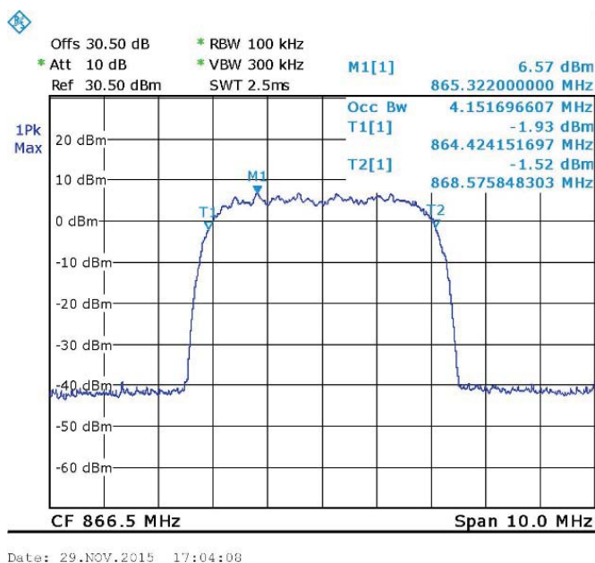
Figure 79. WCDMA - 866.5MHz Output
