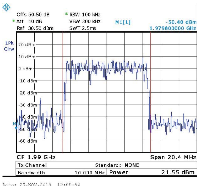
Figure 101. 64QAM - 1990.00 MHz
