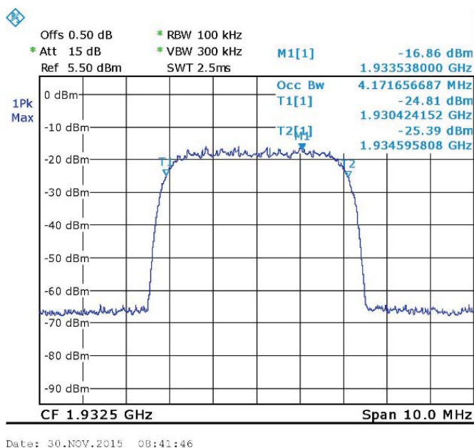
Figure 122.WCDMA - 1932.5 MHz Input
