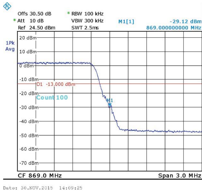
Figure 90— LTE 64QAM - 866.5 MHz
