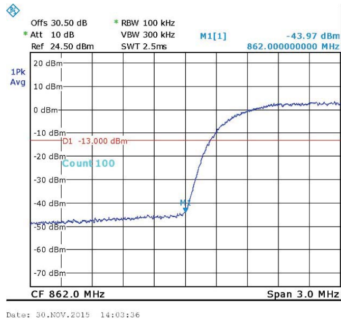
Figure 93—WCDMA - 864.5 MHz
