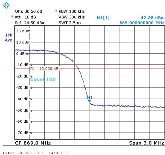
Figure 94—WCDMA - 866.5 MHz
