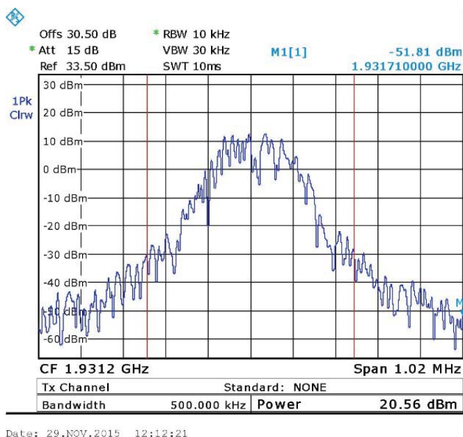
Figure 102. GSM -1931.2 MHz
