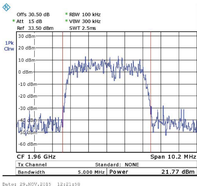
Figure 106. WCDMA- 1960.0 MHz
