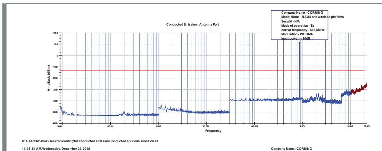
Figure 86. WCDMA - 866.5 MHz
