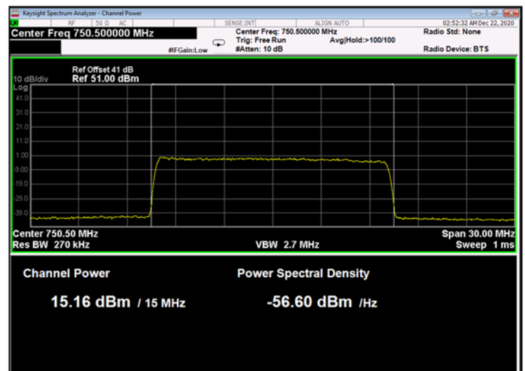
Figure 63: 64QAM 15MHz B.W.; 750.5MHz, 15kHz
