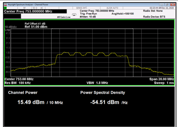
Figure 22: 16QAM 10MHz B.W.; 753.0MHz, 30kHz
