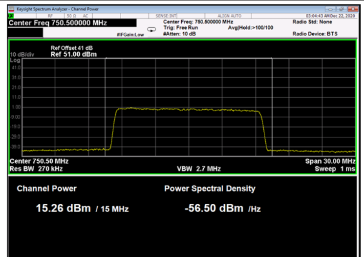
Figure 65: 64QAM 15MHz B.W.; 750.5MHz, 60kHz
