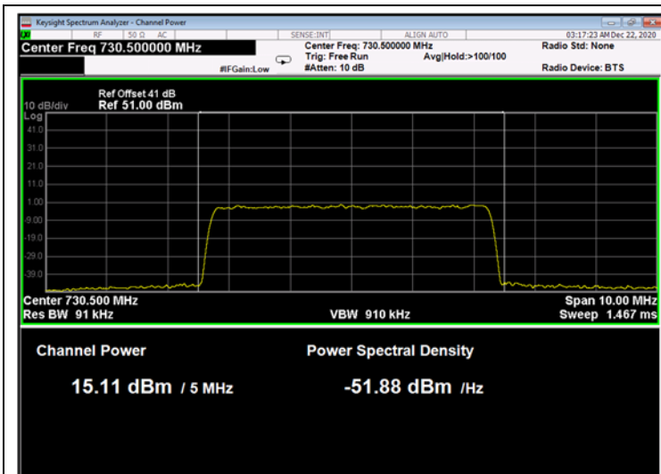
Figure 75: 256QAM 5MHz B.W.; 730.5MHz, 15kHz
