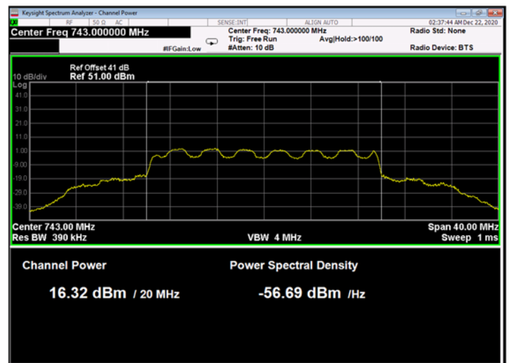
Figure 36: 16QAM 20MHz B.W.; 743.0MHz, 15kHz
