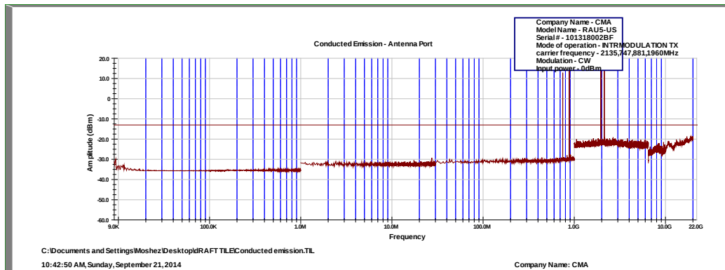
Figure 174 Intermodulation, Port 1
