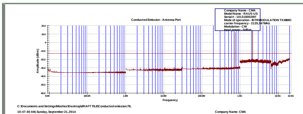
Figure 175 Intermodulation, Port 2
