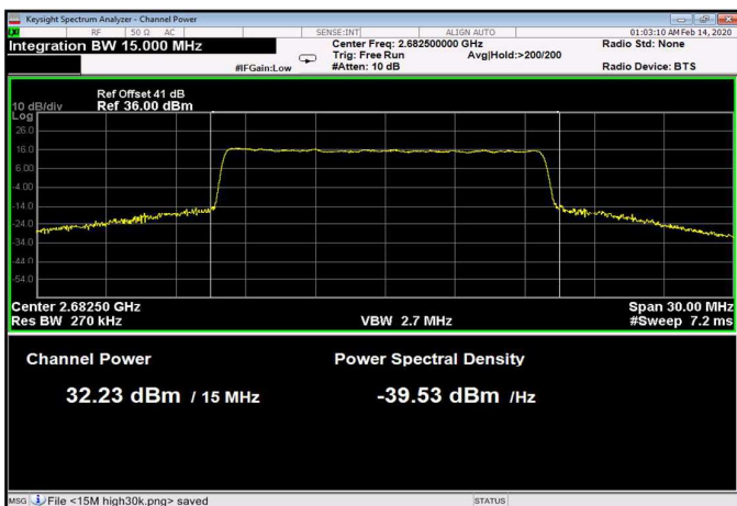
Figure 127: 256QAM 15MHz B.W.; 2682.5MHz, 60kHz
