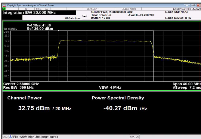
Figure 136: 256QAM 20MHz B.W.; 2680.0MHz, 60kHz
