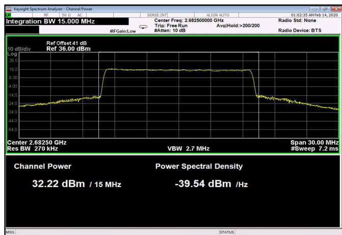
Figure 125: 256QAM 15MHz B.W.; 2682.5MHz, 15kHz
