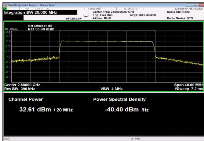
Figure 134: 256QAM 20MHz B.W.; 2680.0MHz, 15kHz
