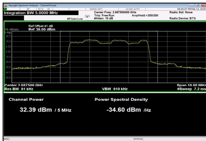
Figure 12: 16QAM 5MHz B.W.; 2687.5MHz, 15kHz
