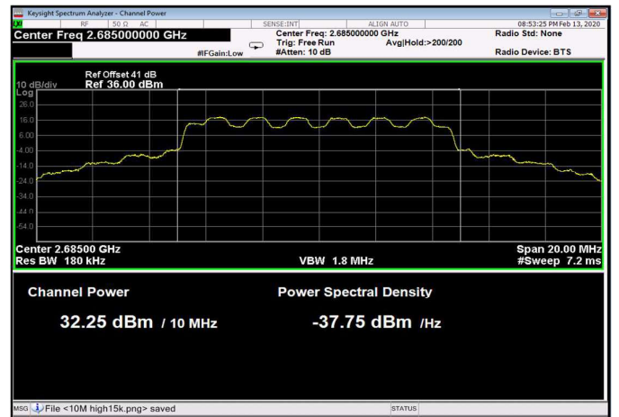
Figure 21: 16QAM 10MHz C.S; 2685.0MHz, 30kHz
