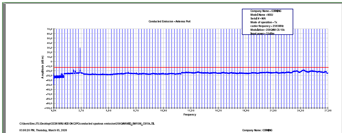
Figure 552: Spurious Emissions at Antenna Terminal 256QAM, 2593.0MHz, B.W. 15MHz, Sub Carrier 15kHz
