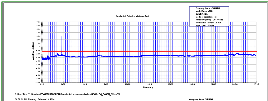
Figure 524: Spurious Emissions at Antenna Terminal 64QAM, 2516.0MHz, B.W. 40MHz, Sub Carrier 30kHz
