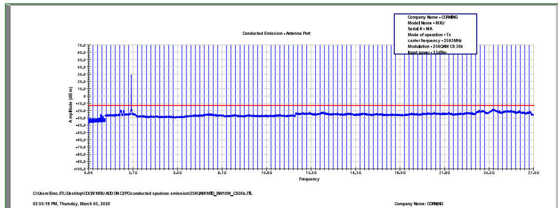
Figure 546: Spurious Emissions at Antenna Terminal 256QAM, 2593.0MHz, B.W. 10MHz, Sub Carrier 30kHz
