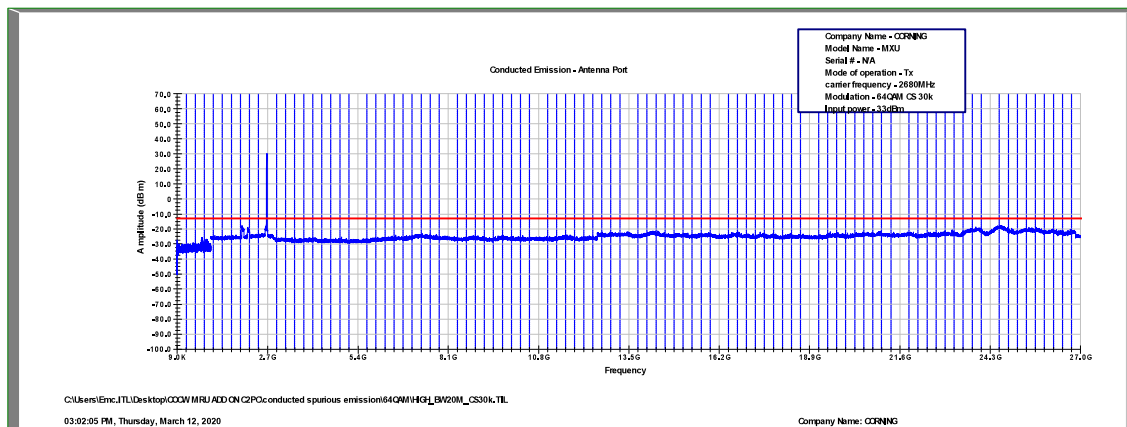
Figure 517: Spurious Emissions at Antenna Terminal 64QAM, 2680.0MHz, B.W. 20MHz, Sub Carrier 30kHz
