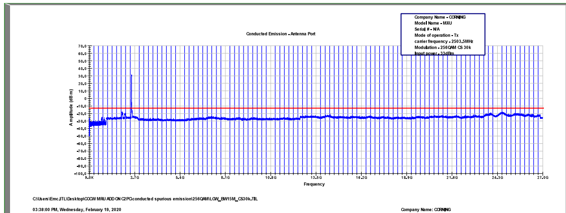
Figure 554: Spurious Emissions at Antenna Terminal 256QAM, 2503.5MHz, B.W. 15MHz, Sub Carrier 30kHz
