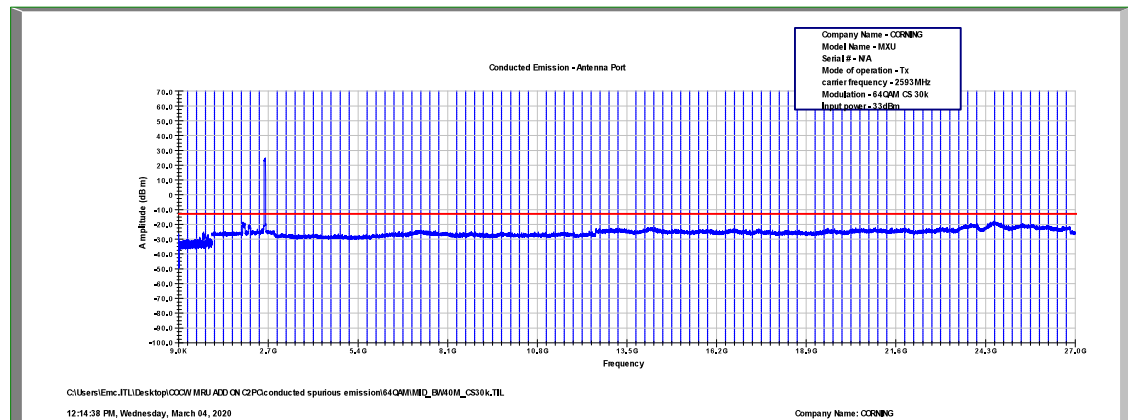
Figure 525: Spurious Emissions at Antenna Terminal 64QAM, 2593.0MHz, B.W. 40MHz, Sub Carrier 30kHz
