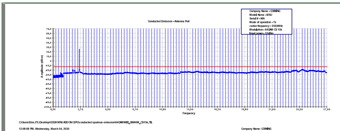
Figure 522: Spurious Emissions at Antenna Terminal 64QAM, 2593.0MHz, B.W. 40MHz, Sub Carrier 15kHz
