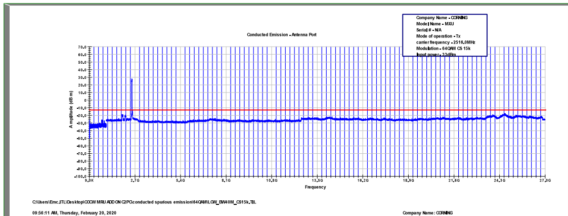
Figure 521: Spurious Emissions at Antenna Terminal 64QAM, 2516.0MHz, B.W. 40MHz, Sub Carrier 15kHz
