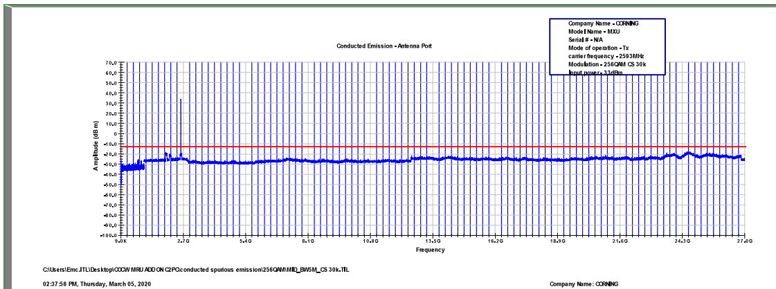
Figure 540: Spurious Emissions at Antenna Terminal 256QAM, 2593.0MHz, B.W. 5MHz, Sub Carrier 30kHz
