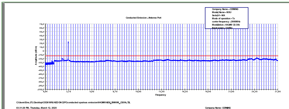
Figure 532: Spurious Emissions at Antenna Terminal 64QAM, 2660.0MHz, B.W. 60MHz, Sub Carrier 30kHz
