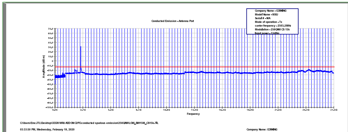
Figure 551: Spurious Emissions at Antenna Terminal 256QAM, 2503.5MHz, B.W. 15MHz, Sub Carrier 15kHz
