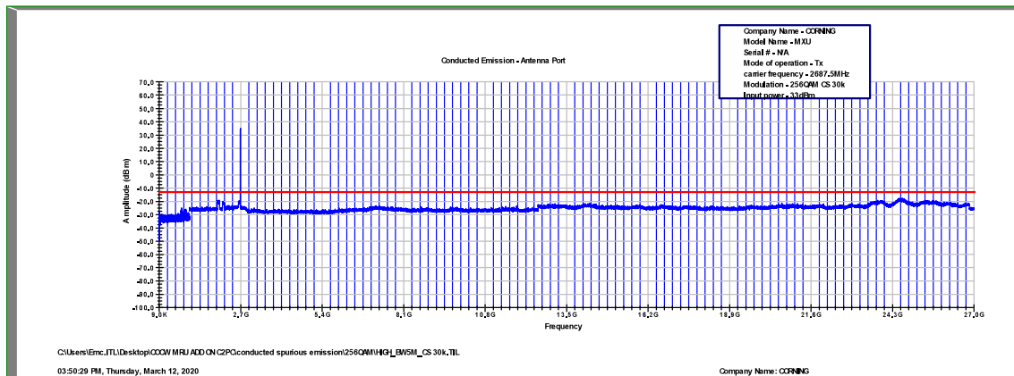
Figure 541: Spurious Emissions at Antenna Terminal 256QAM, 2687.5MHz, B.W. 5MHz, Sub Carrier 30kHz
