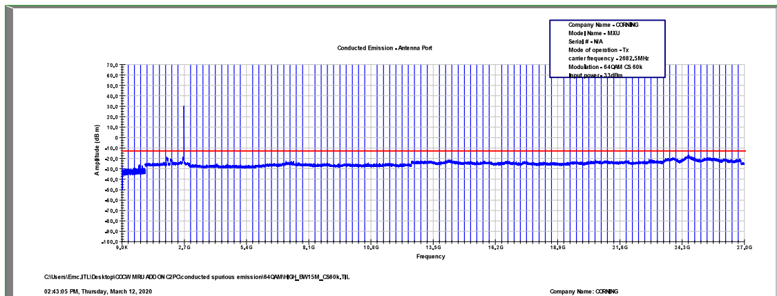
Figure 511: Spurious Emissions at Antenna Terminal 64QAM, 2682.5MHz, B.W. 15MHz, Sub Carrier 60kHz
