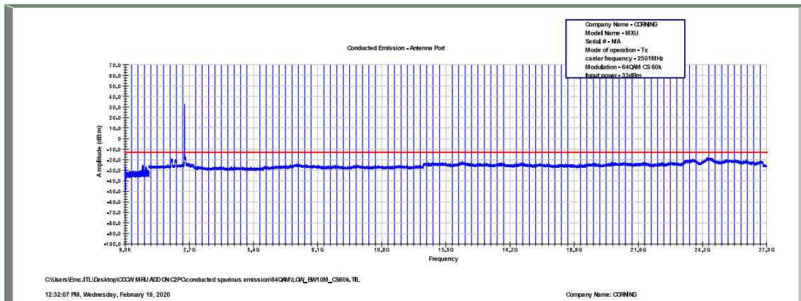
Figure 500: Spurious Emissions at Antenna Terminal 64QAM, 2501.0MHz, B.W. 10MHz, Sub Carrier 60kHz
