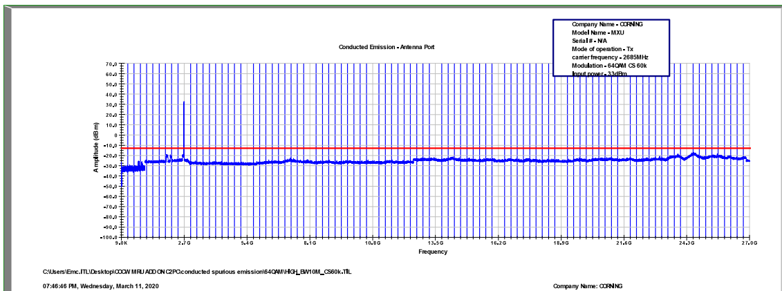
Figure 502: Spurious Emissions at Antenna Terminal 64QAM, 2685.0MHz, B.W. 10MHz, Sub Carrier 60kHz
