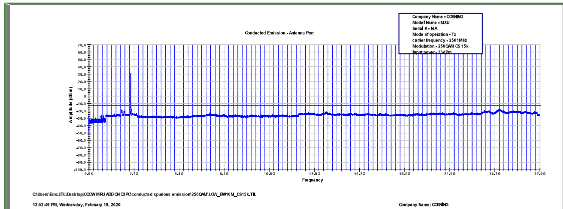
Figure 542: Spurious Emissions at Antenna Terminal 256QAM, 2501.0MHz, B.W. 10MHz, Sub Carrier 15kHz
