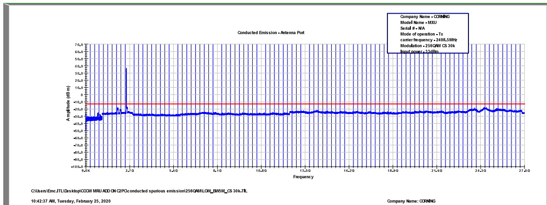
Figure 539: Spurious Emissions at Antenna Terminal 256QAM, 2498.5MHz, B.W. 5MHz, Sub Carrier 30kHz
