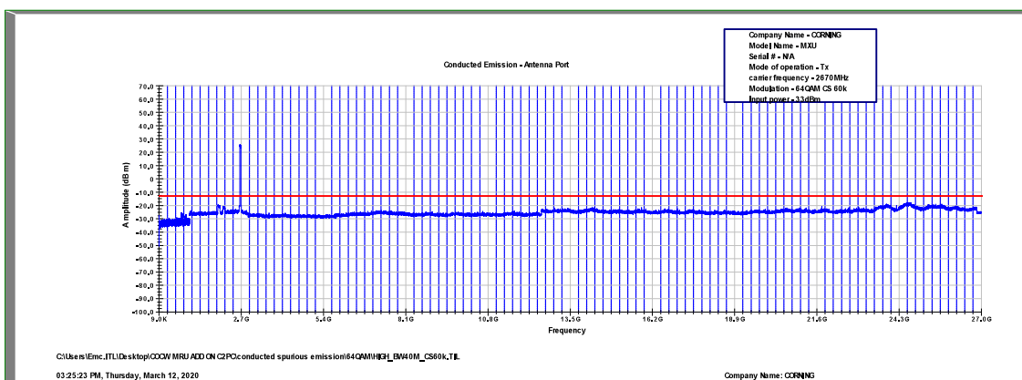
Figure 529: Spurious Emissions at Antenna Terminal 64QAM, 2670.0MHz, B.W. 40MHz, Sub Carrier 60kHz
