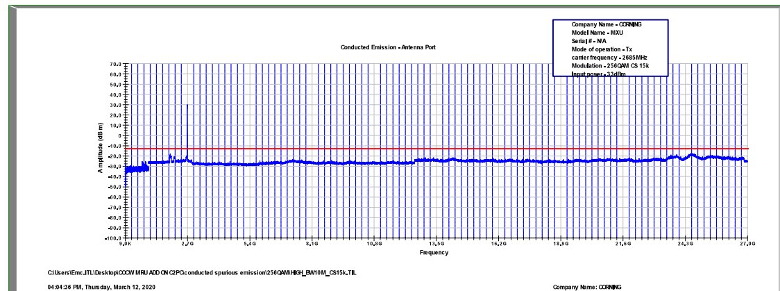
Figure 544: Spurious Emissions at Antenna Terminal 256QAM, 2685.0MHz, B.W. 10MHz, Sub Carrier 15kHz
