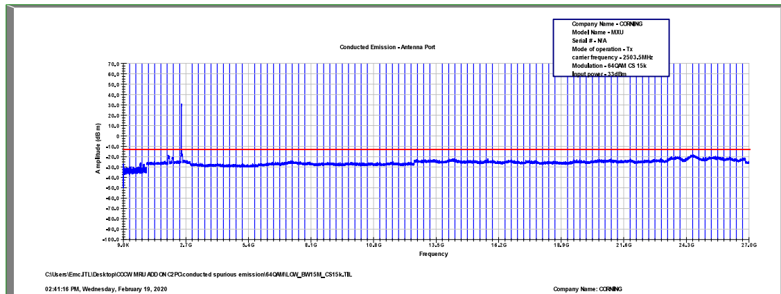
Figure 503: Spurious Emissions at Antenna Terminal 64QAM, 2503.5MHz, B.W. 15MHz, Sub Carrier 15kHz
