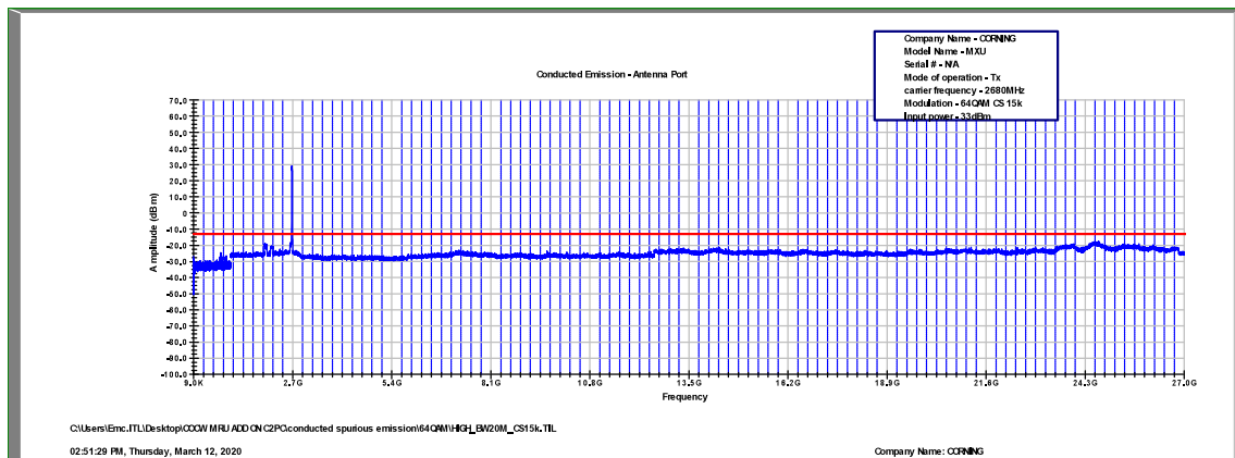
Figure 514: Spurious Emissions at Antenna Terminal 64QAM, 2680.0MHz, B.W. 20MHz, Sub Carrier 15kHz
