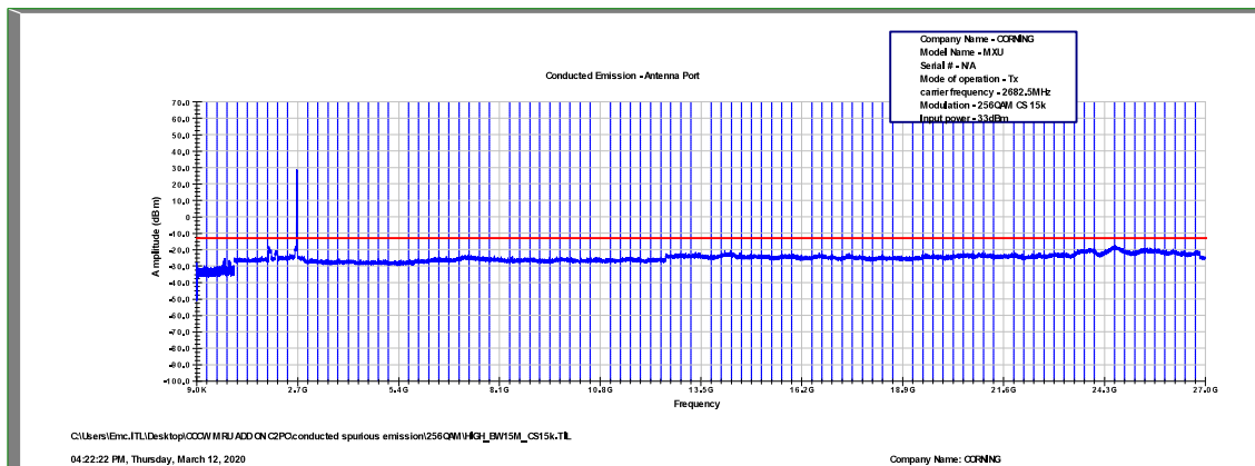
Figure 553: Spurious Emissions at Antenna Terminal 256QAM, 2682.5MHz, B.W. 15MHz, Sub Carrier 15kHz
