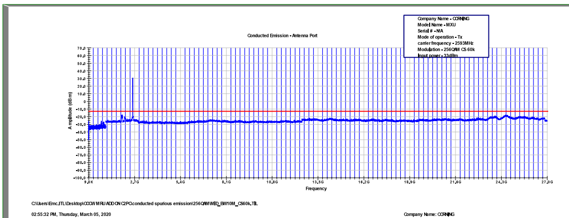
Figure 549: Spurious Emissions at Antenna Terminal 256QAM, 2593.0MHz, B.W. 10MHz, Sub Carrier 60kHz
