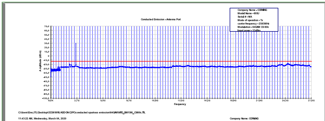
Figure 510: Spurious Emissions at Antenna Terminal 64QAM, 2593.0MHz, B.W. 15MHz, Sub Carrier 60kHz
