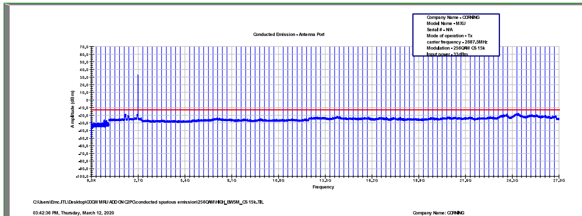
Figure 538: Spurious Emissions at Antenna Terminal 256QAM, 2687.5MHz, B.W. 5MHz, Sub Carrier 15kHz
