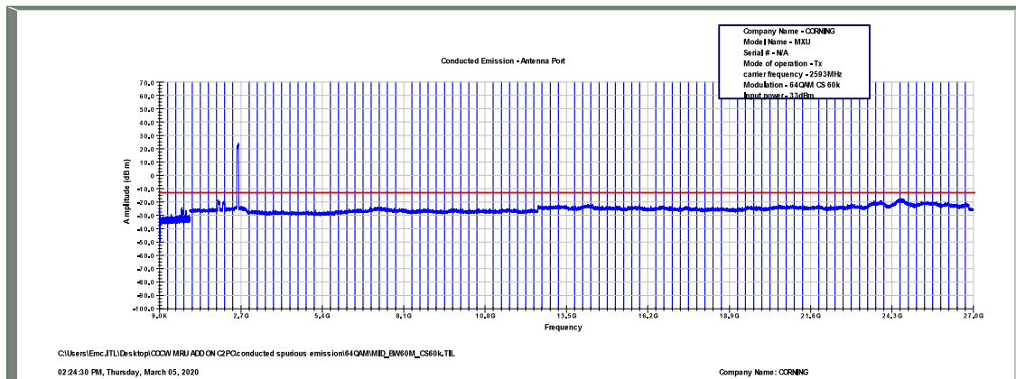
Figure 534: Spurious Emissions at Antenna Terminal 64QAM, 2593.0MHz, B.W. 60MHz, Sub Carrier 60kHz
