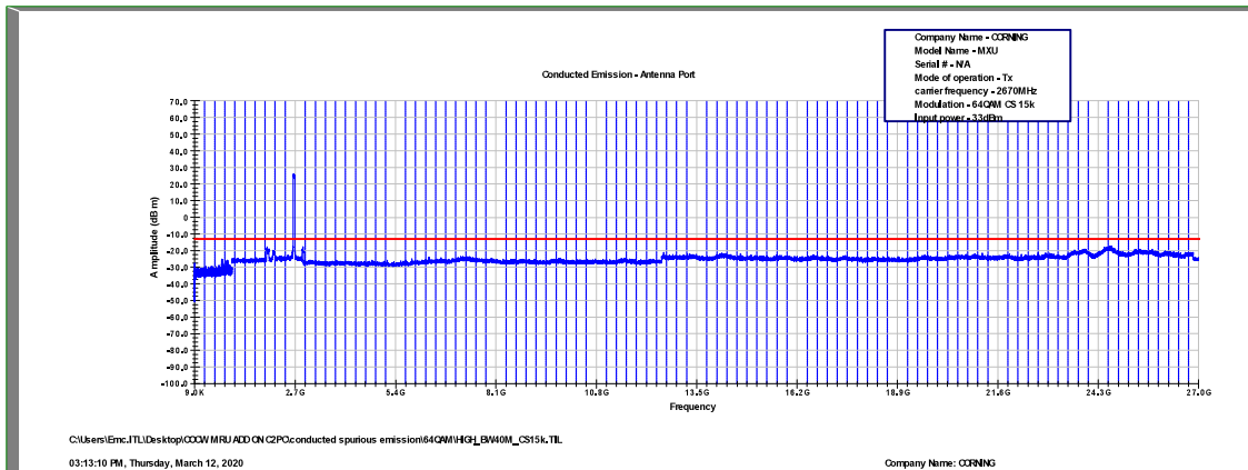
Figure 523: Spurious Emissions at Antenna Terminal 64QAM, 2670.0MHz, B.W. 40MHz, Sub Carrier 15kHz
