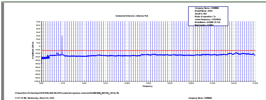
Figure 504: Spurious Emissions at Antenna Terminal 64QAM, 2593.0MHz, B.W. 15MHz, Sub Carrier 15kHz
