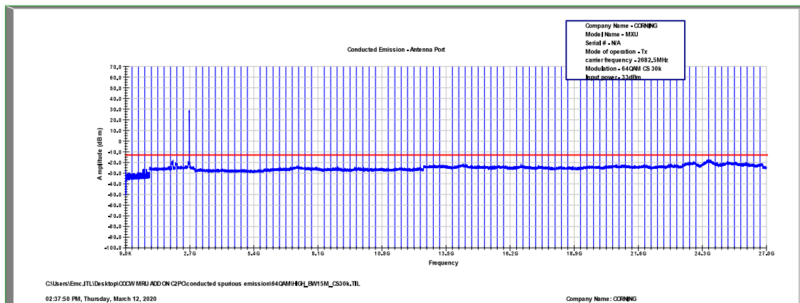
Figure 508: Spurious Emissions at Antenna Terminal 64QAM, 2682.5MHz, B.W. 15MHz, Sub Carrier 30kHz
