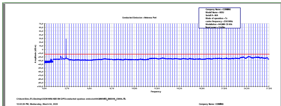
Figure 519: Spurious Emissions at Antenna Terminal 64QAM, 2593.0MHz, B.W. 20MHz, Sub Carrier 60kHz
