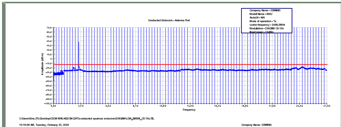
Figure 536: Spurious Emissions at Antenna Terminal 256QAM, 2498.5MHz, B.W. 5MHz, Sub Carrier 15kHz
