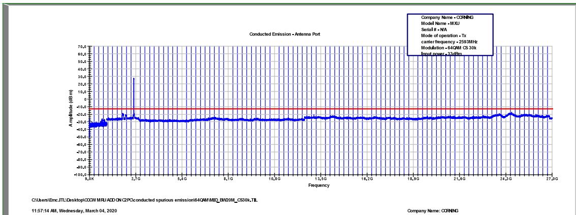
Figure 516: Spurious Emissions at Antenna Terminal 64QAM, 2593.0MHz, B.W. 20MHz, Sub Carrier 30kHz
