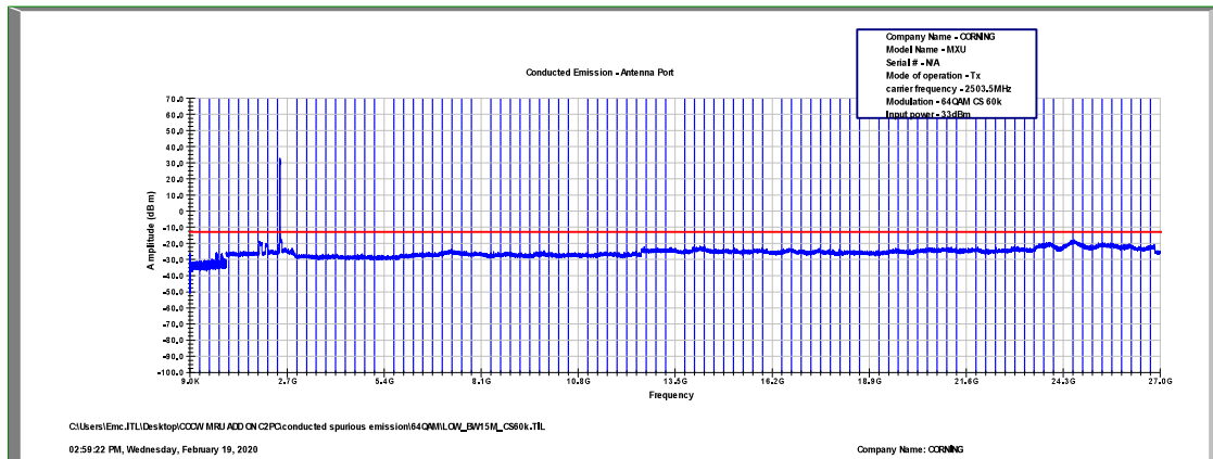
Figure 509: Spurious Emissions at Antenna Terminal 64QAM, 2503.5MHz, B.W. 15MHz, Sub Carrier 60kHz
