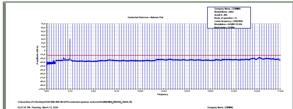
Figure 520: Spurious Emissions at Antenna Terminal 64QAM, 2680.0MHz, B.W. 20MHz, Sub Carrier 60kHz
