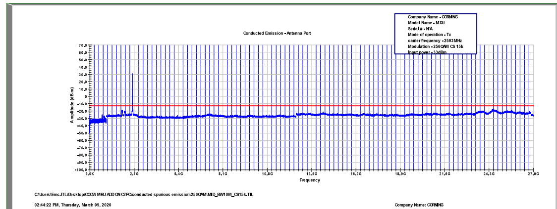
Figure 543: Spurious Emissions at Antenna Terminal 256QAM, 2593.0MHz, B.W. 10MHz, Sub Carrier 15kHz
