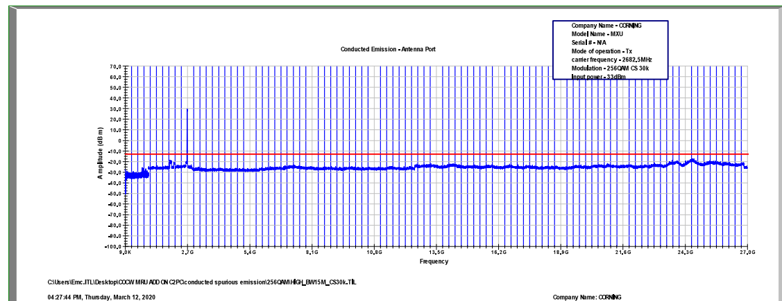
Figure 556: Spurious Emissions at Antenna Terminal 256QAM, 2682.5MHz, B.W. 15MHz, Sub Carrier 30kHz
