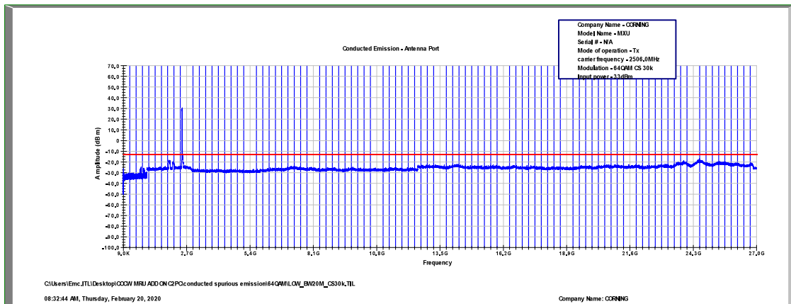
Figure 515: Spurious Emissions at Antenna Terminal 64QAM, 2506.0MHz, B.W. 20MHz, Sub Carrier 30kHz
