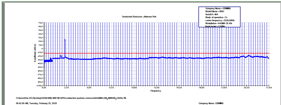
Figure 530: Spurious Emissions at Antenna Terminal 64QAM, 2526.0MHz, B.W. 60MHz, Sub Carrier 30kHz
