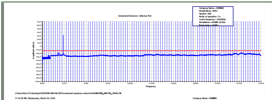
Figure 501: Spurious Emissions at Antenna Terminal 64QAM, 2593.0MHz, B.W. 10MHz, Sub Carrier 60kHz
