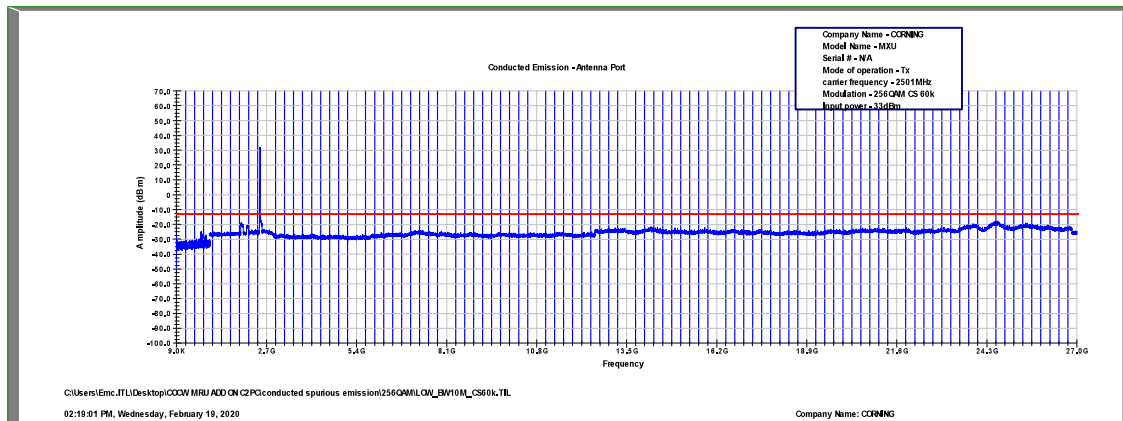
Figure 548: Spurious Emissions at Antenna Terminal 256QAM, 2501.0MHz, B.W. 10MHz, Sub Carrier 60kHz
