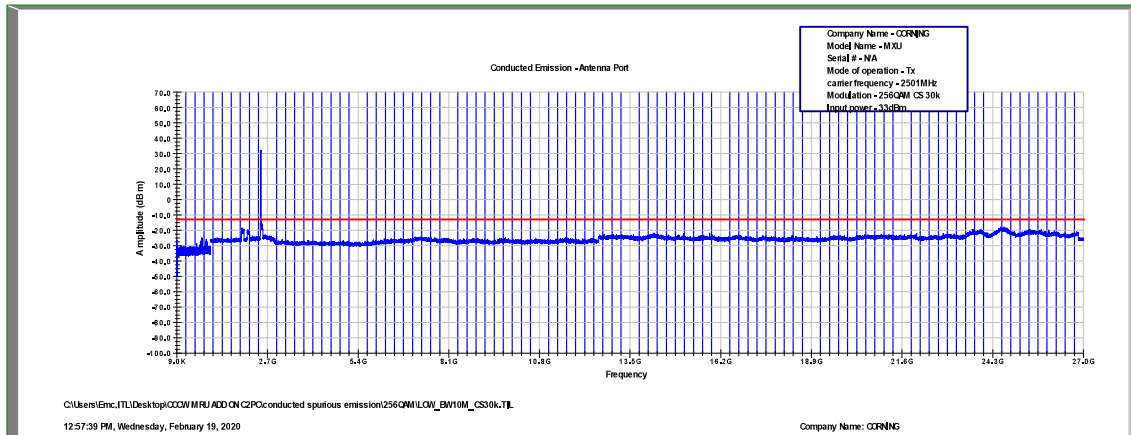
Figure 545: Spurious Emissions at Antenna Terminal 256QAM, 2501.0MHz, B.W. 10MHz, Sub Carrier 30kHz
