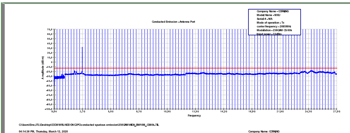
Figure 550: Spurious Emissions at Antenna Terminal 256QAM, 2685.0MHz, B.W. 10MHz, Sub Carrier 60kHz
