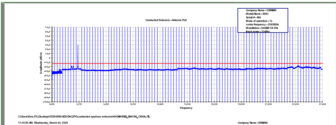
Figure 507: Spurious Emissions at Antenna Terminal 64QAM, 2593.0MHz, B.W. 15MHz, Sub Carrier 30kHz
