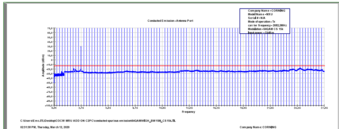
Figure 505: Spurious Emissions at Antenna Terminal 64QAM, 2682.5MHz, B.W. 15MHz, Sub Carrier 15kHz
