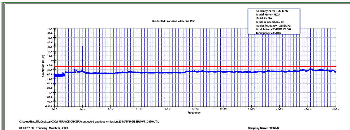
Figure 547: Spurious Emissions at Antenna Terminal 256QAM, 2685.0MHz, B.W. 10MHz, Sub Carrier 30kHz
