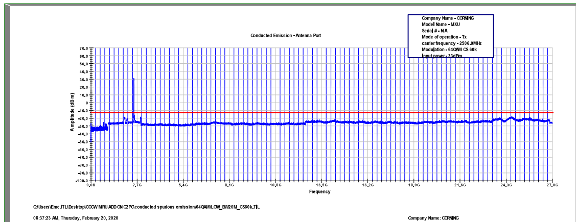
Figure 518: Spurious Emissions at Antenna Terminal 64QAM, 2506.0MHz, B.W. 20MHz, Sub Carrier 60kHz
