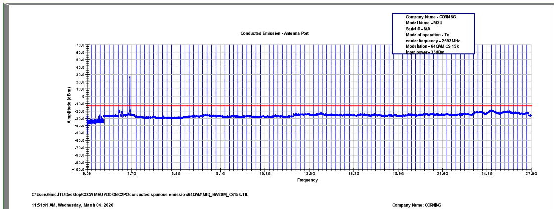
Figure 513: Spurious Emissions at Antenna Terminal 64QAM, 2593.0MHz, B.W. 20MHz, Sub Carrier 15kHz
