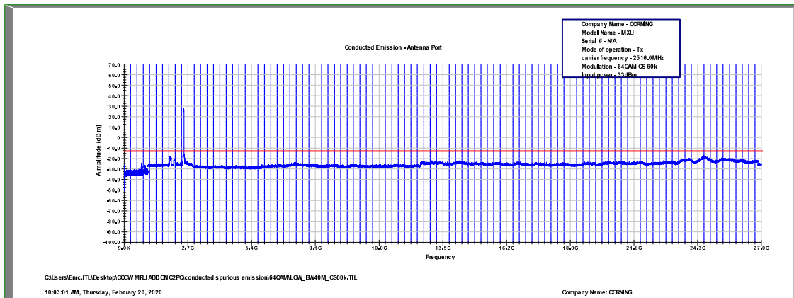
Figure 527: Spurious Emissions at Antenna Terminal 64QAM, 2516.0MHz, B.W. 40MHz, Sub Carrier 60kHz
