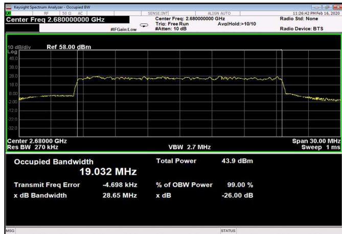
Figure 424: 256QAM 20MHz B.W.; 2680.0MHz, 60kHz Output
