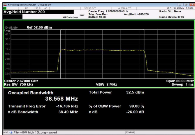
Figure 384: 64QAM 40MHz B.W.; 2670.0MHz, 15kHz Output
