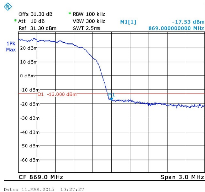
Figure 93. — W-CDMA - 866.5 MHz
