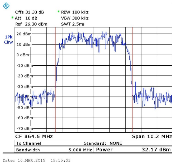
Figure 63.—864.5 MHz – WCDMA
