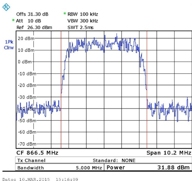
Figure 64. — 866.5 MHz – WCDMA
