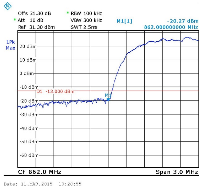
Figure 92. — W-CDMA - 864.5 MHz
