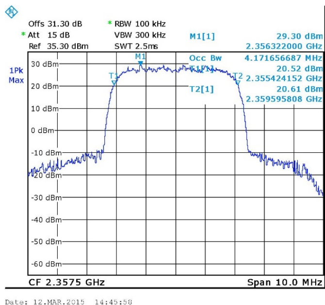
Figure 36 Occupied Bandwidth OUTPUT, WCDMA
