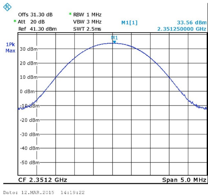
Figure 17 - 2351.2MHz – GSM
