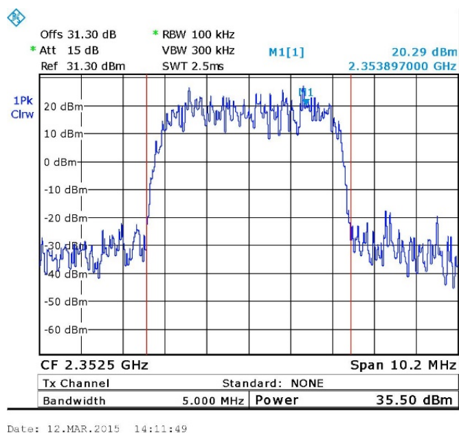
Figure 11. — 2352.5 MHz – W-CDMA
