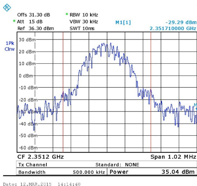
Figure 9. — 2351.2 MHz - GSM
