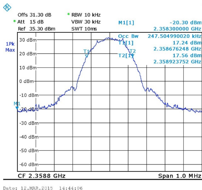
Figure 30 Occupied Bandwidth OUTPUT, GSM
