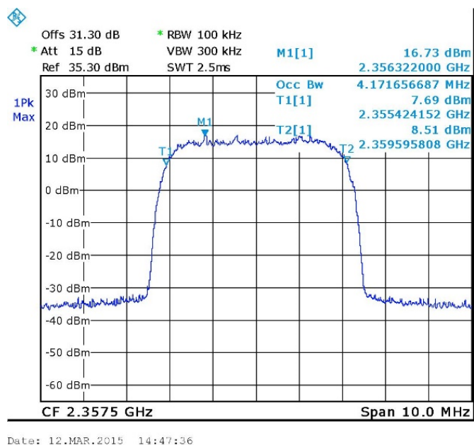
Figure 35 Occupied Bandwidth INPUT, WCDMA
