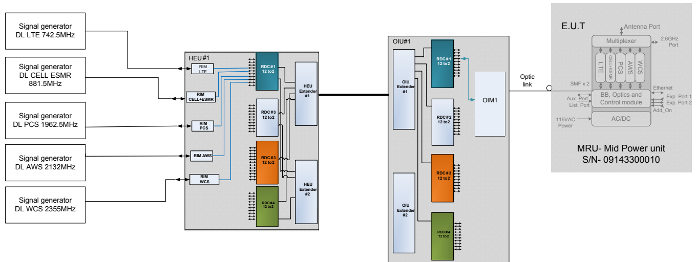
Figure 1. Test Set-up
