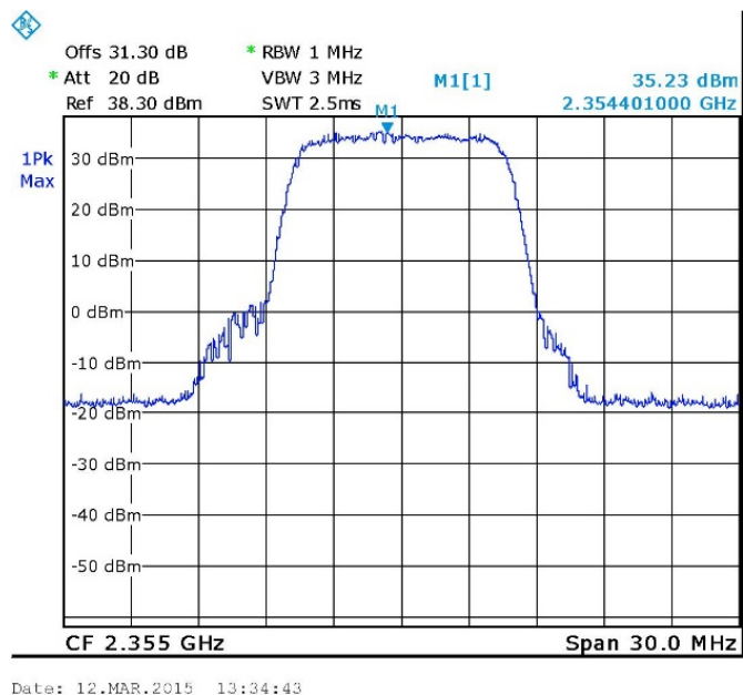
Figure 16. — 2355.0 MHz – LTE 64QAM
