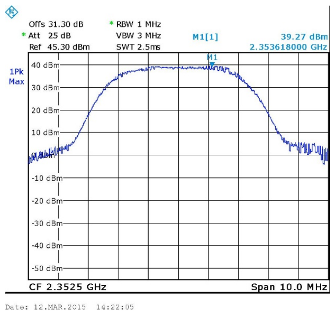
Figure 19. — 2352.5MHz – W-CDMA
