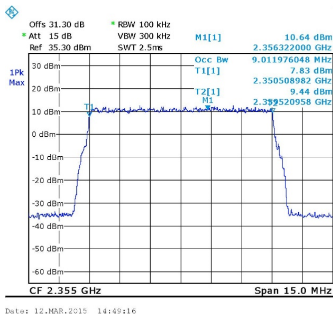
Figure 31 Occupied Bandwidth INPUT, LTE
