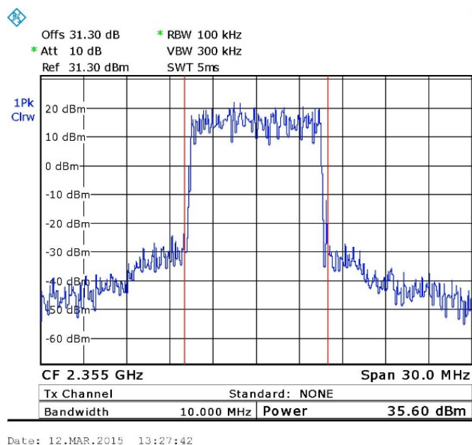
Figure 8. — 2355.0 MHz – LTE 64QAM
