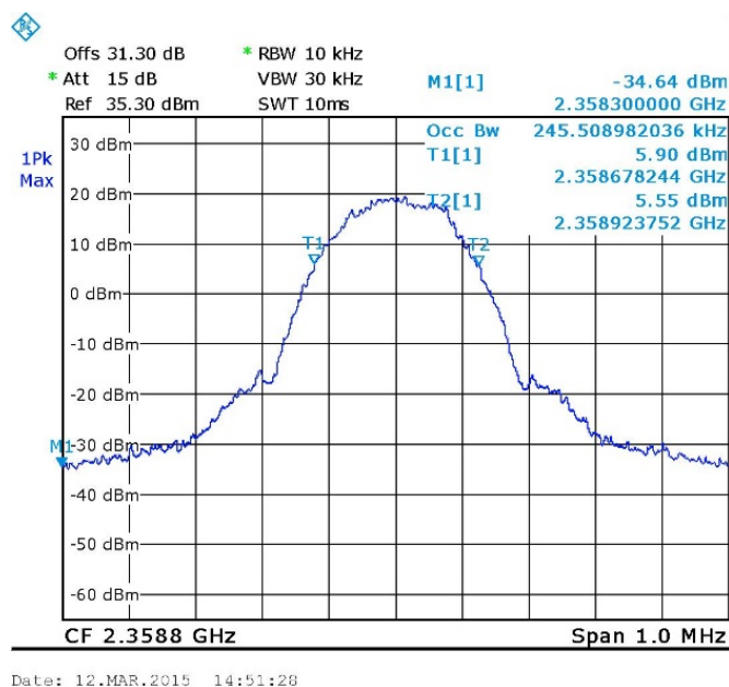
Figure 29 Occupied Bandwidth INPUT, GSM
