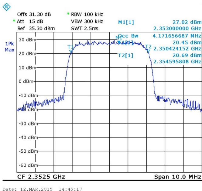
Figure 34 Occupied Bandwidth OUTPUT, WCDMA
