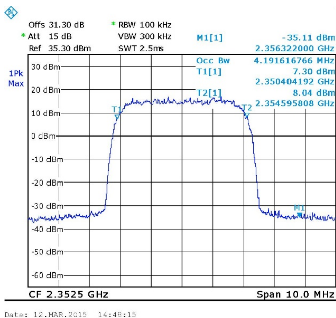
Figure 33 Occupied Bandwidth INPUT, WCDMA
