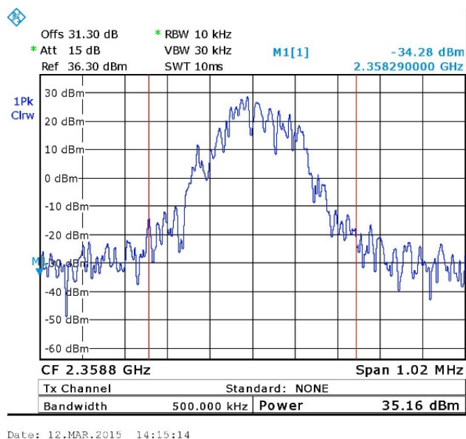
Figure 10. — 2358.8 MHz- GSM
