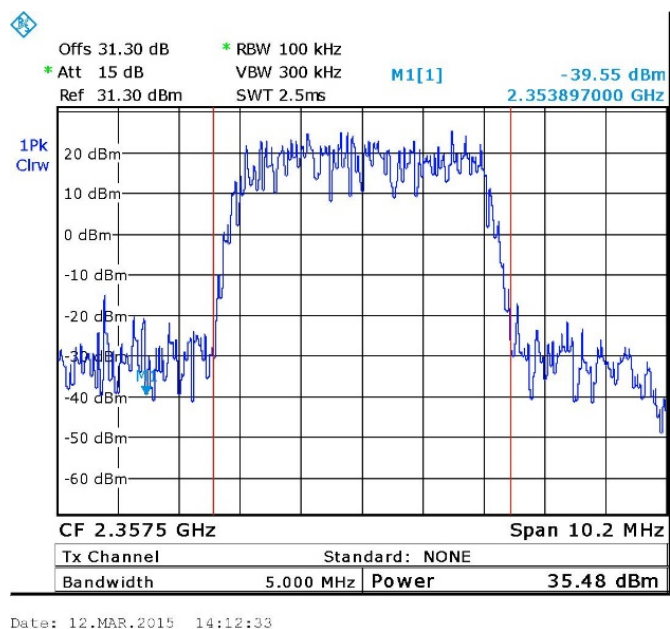
Figure 12. — 2357.5 MHz – W-CDMA
