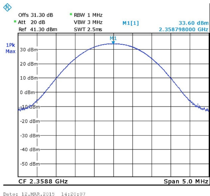
Figure 18.—2358.8 MHz- GSM
