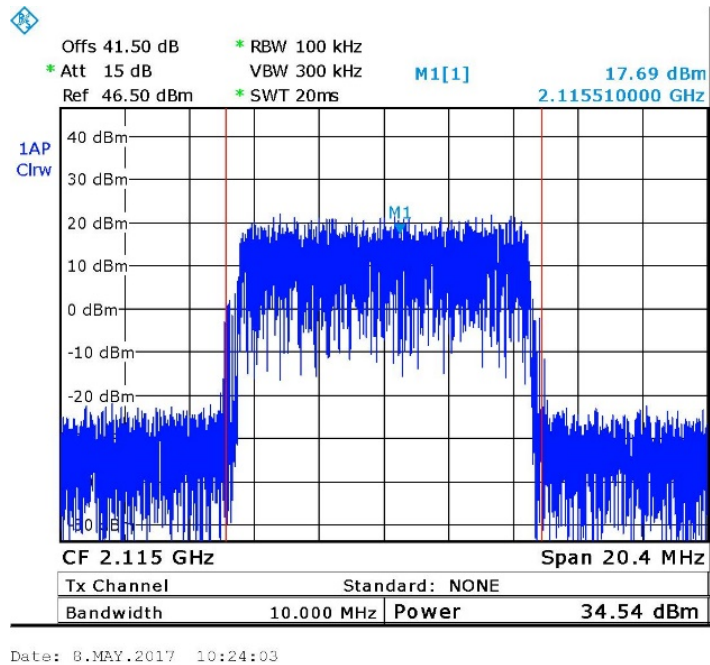
Figure 13. — LTE 64QAM (2115.0 MHz)
