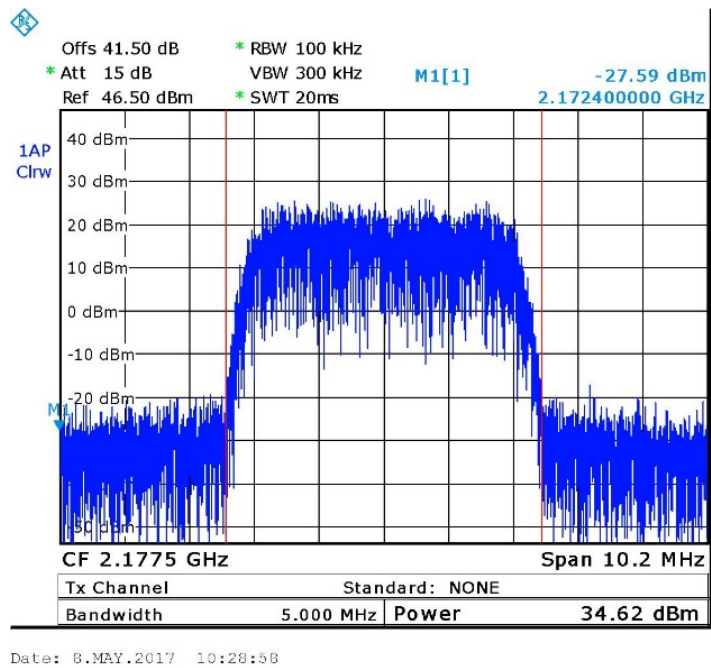
Figure 18. — W-CDMA (2177.5MHz)
