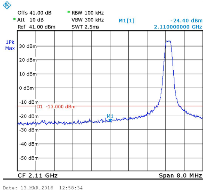
Figure 50. — GSM 2111.2 MHz
