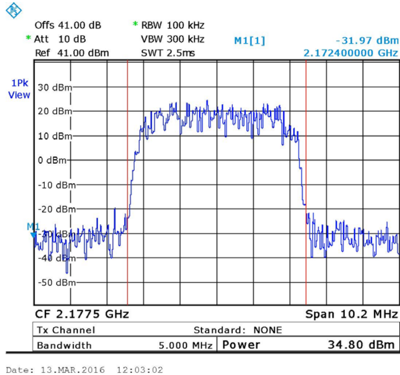
Figure 17. — W-CDMA (2177.5MHz)
