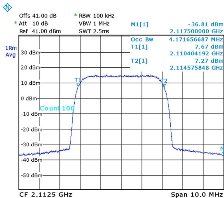
Figure 32. — W-CDMA (2112.5 MHz) IN
