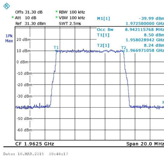
Figure 21. — LTE 64QAM Input 1962.50 MHz
