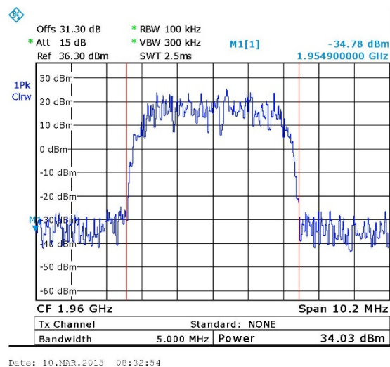
Figure 15. — W-CDMA - 1960.00 MHz
