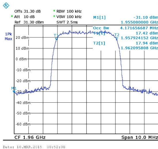
Figure 33. — W-CDMA - Input 1960.00 MHz
