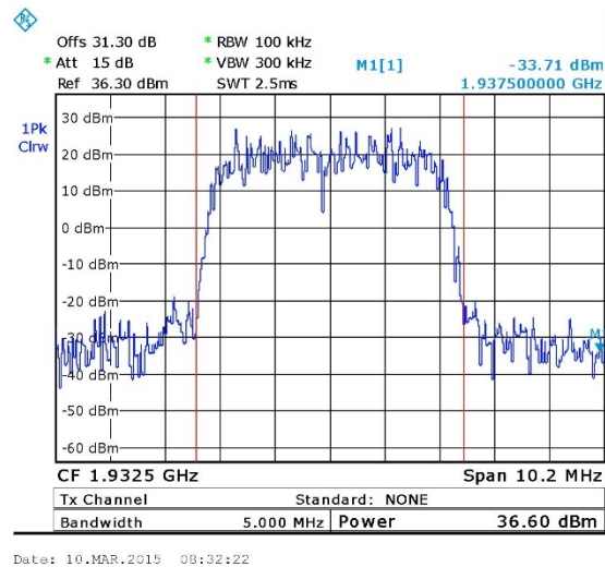
Figure 14. — W-CDMA - 1932.50 MHz
