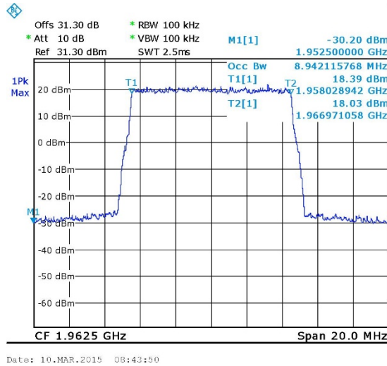
Figure 22. — LTE 64QAM Output 1962.50 MHz
