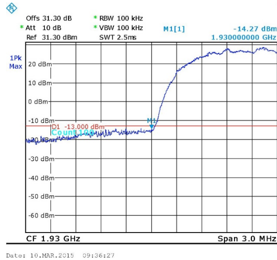
Figure 53. — W-CDMA - 1932.50 MHz
