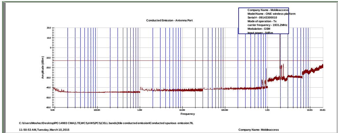
Figure 41. — GSM - 1931.2 MHz
