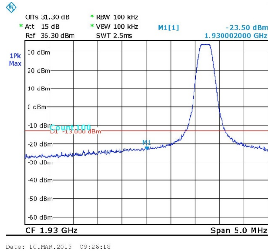
Figure 51. — GSM - 1931.20 MHz
