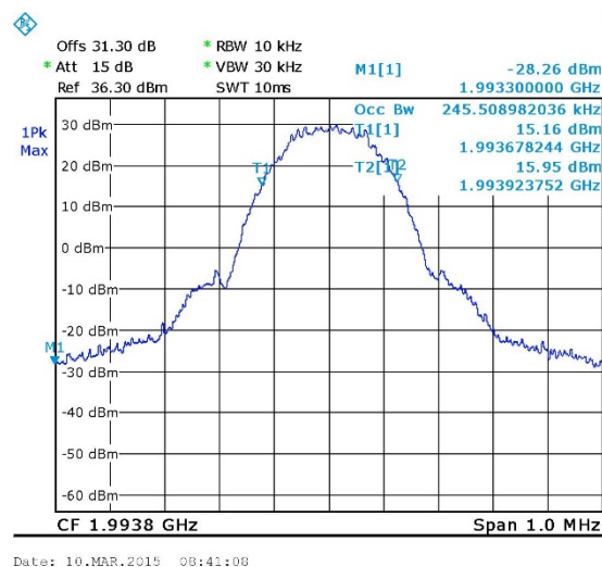
Figure 30. — GSM - Output 1993.80 MHz
