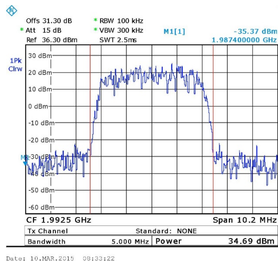
Figure 16. — W-CDMA - 1992.50 MHz
