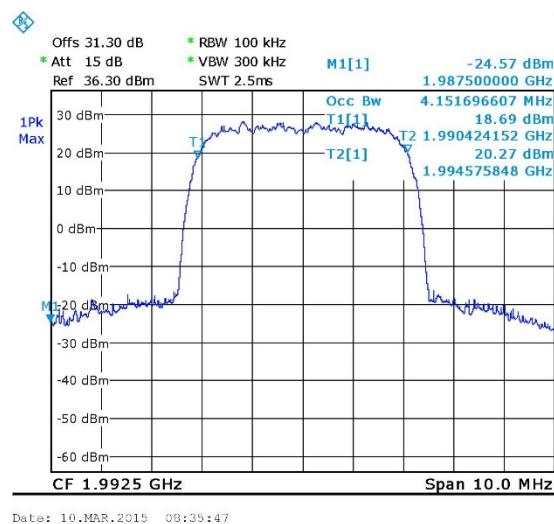
Figure 36. — W-CDMA - Output 1992.50 MHz
