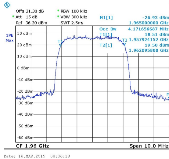
Figure 34. — W-CDMA - Output 1960.00 MHz
