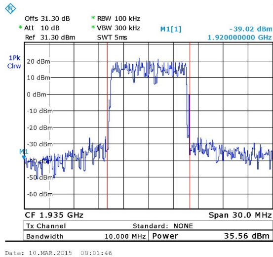
Figure 8. — LTE 64QAM 1935.00 MHz
