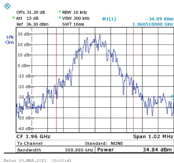
Figure 12. — GSM -1960.00 MHz
