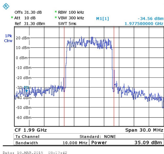
Figure 10. — LTE 64QAM 1990.00 MHz
