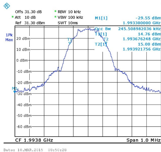
Figure 29. — GSM - Input 1993.80 MHz
