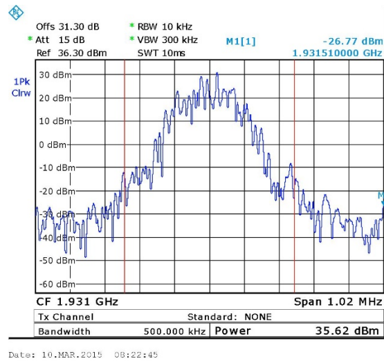
Figure 11. — GSM - 1931.20 MHz
