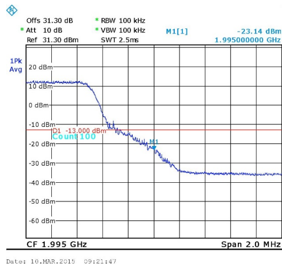
Figure 50. — LTE 64QAM 1990.00 MHz
