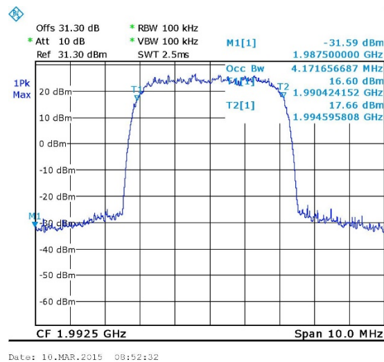
Figure 35. — W-CDMA - Input 1992.50 MHz
