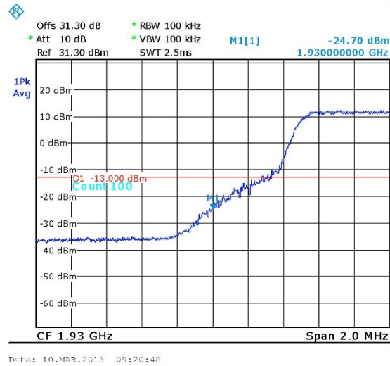
Figure 49. — LTE 64QAM 1935.00 MHz
