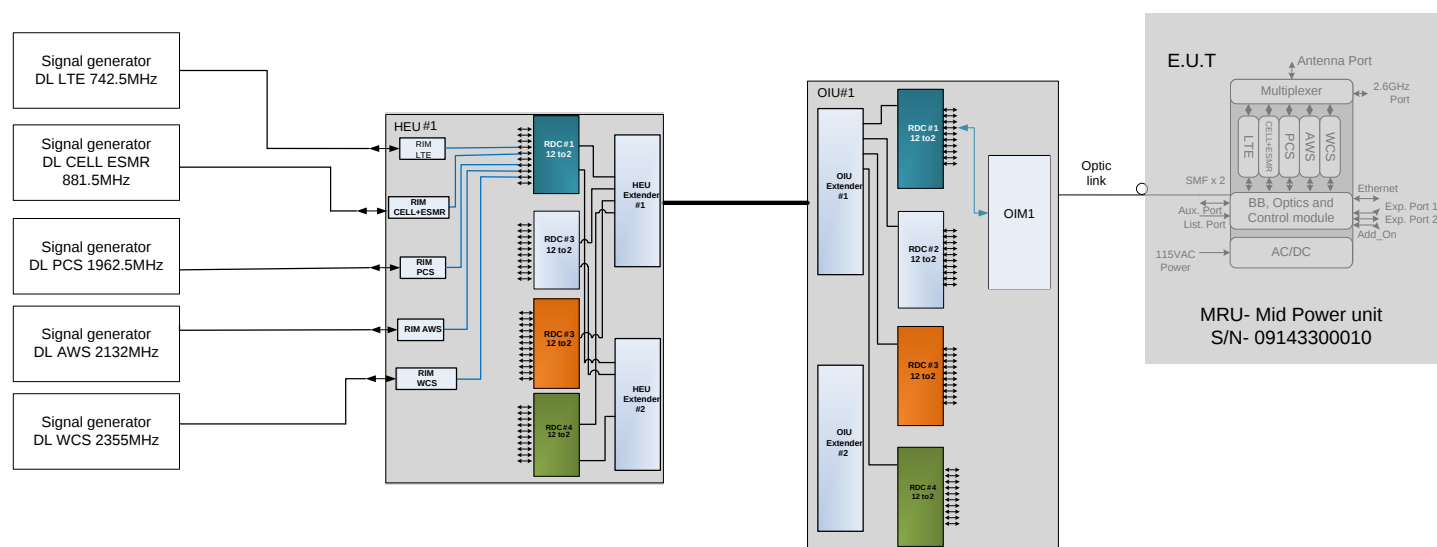
Figure 1. Test Set-up
