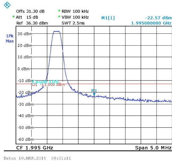
Figure 52. — GSM - 1993.80 MHz
