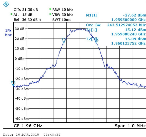
Figure 28. — GSM - Output 1960.00 MHz
