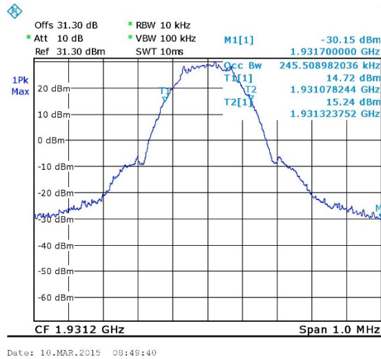
Figure 25. — GSM - Input 1931.20 MHz
