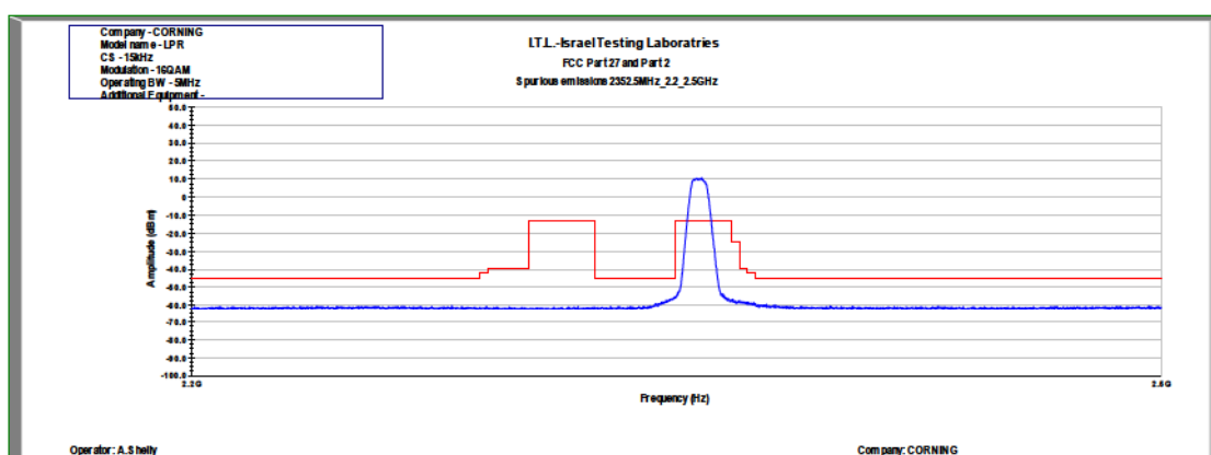
Figure 91: Spurious Emissions at Antenna Terminal 16QAM, 2352.5MHz, B.W. 5MHz, Sub Carrier 15 kHz
