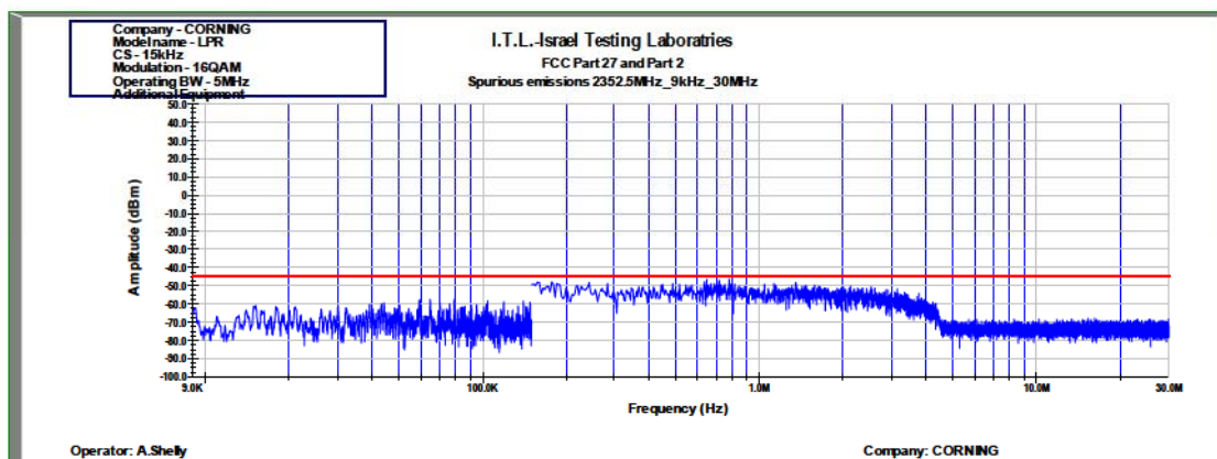
Figure 89: Spurious Emissions at Antenna Terminal 16QAM, 2352.5MHz, B.W. 5MHz, Sub Carrier 15 kHz
