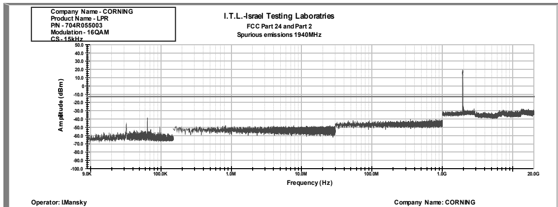
Figure 328: Spurious Emissions at Antenna Terminal 16QAM, 1940.0MHz, B.W. 20MHz, Sub Carrier 15 kHz
