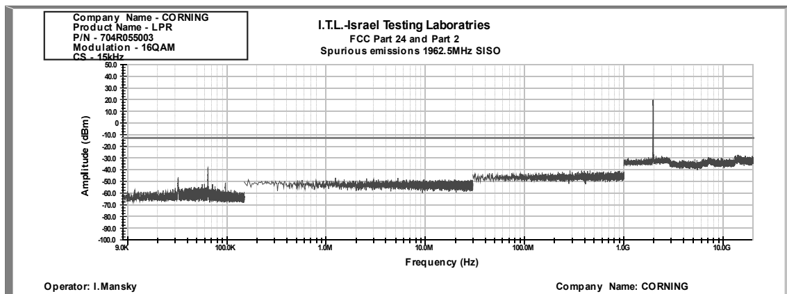
Figure 329: Spurious Emissions at Antenna Terminal 16QAM, 1962.5MHz, B.W. 20MHz, Sub Carrier 15 kHz
