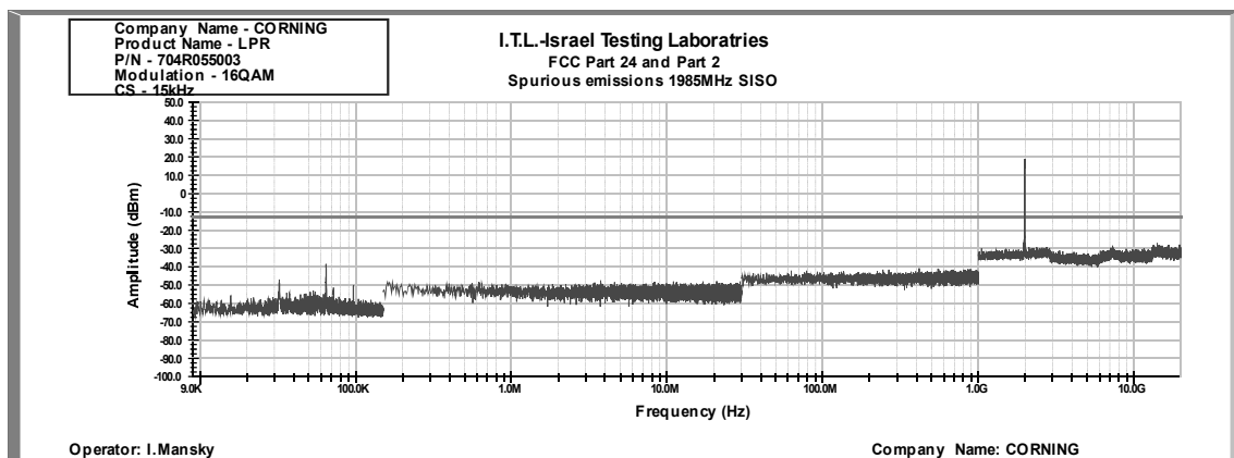
Figure 330: Spurious Emissions at Antenna Terminal 16QAM, 1985.0MHz, B.W. 20MHz, Sub Carrier 15 kHz
