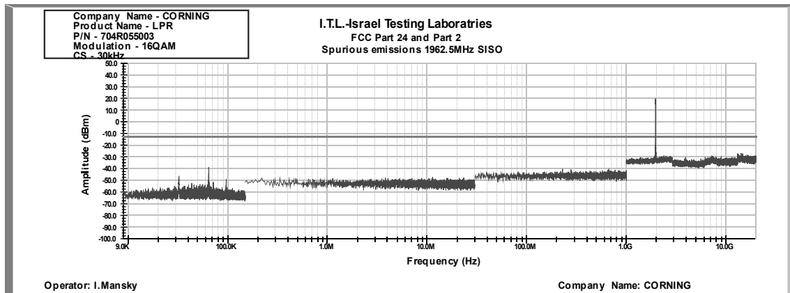
Figure 332: Spurious Emissions at Antenna Terminal 16QAM, 1962.5MHz, B.W. 20MHz, Sub Carrier 30 kHz
