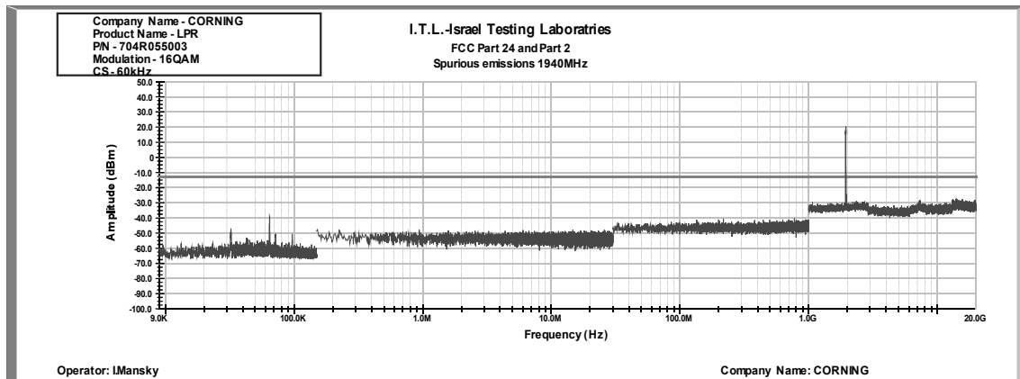
Figure 334: Spurious Emissions at Antenna Terminal 16QAM, 1940.0MHz, B.W. 20MHz, Sub Carrier 60 kHz
