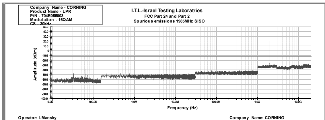
Figure 333: Spurious Emissions at Antenna Terminal 16QAM, 1985.0MHz, B.W. 20MHz, Sub Carrier 30 kHz
