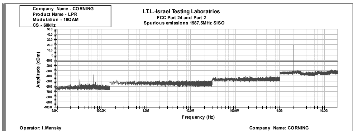
Figure 327: Spurious Emissions at Antenna Terminal 16QAM, 1987.5MHz, B.W. 15MHz, Sub Carrier 60 kHz
