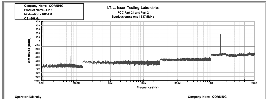
Figure 325: Spurious Emissions at Antenna Terminal 16QAM, 1937.5MHz, B.W. 15MHz, Sub Carrier 60 kHz
