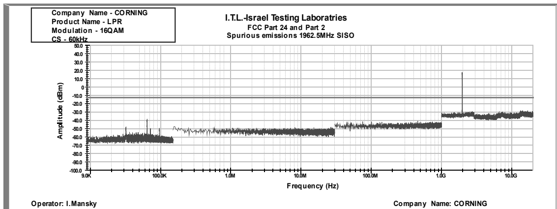
Figure 326: Spurious Emissions at Antenna Terminal 16QAM, 1962.5MHz, B.W. 15MHz, Sub Carrier 60 kHz
