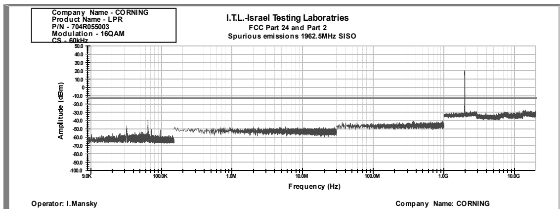
Figure 335: Spurious Emissions at Antenna Terminal 16QAM, 1962.5MHz, B.W. 20MHz, Sub Carrier 60 kHz
