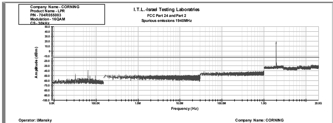
Figure 331: Spurious Emissions at Antenna Terminal 16QAM, 1940.0MHz, B.W. 20MHz, Sub Carrier 30 kHz
