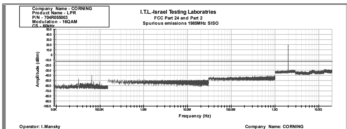
Figure 336: Spurious Emissions at Antenna Terminal 16QAM, 1985.0MHz, B.W. 20MHz, Sub Carrier 60 kHz
