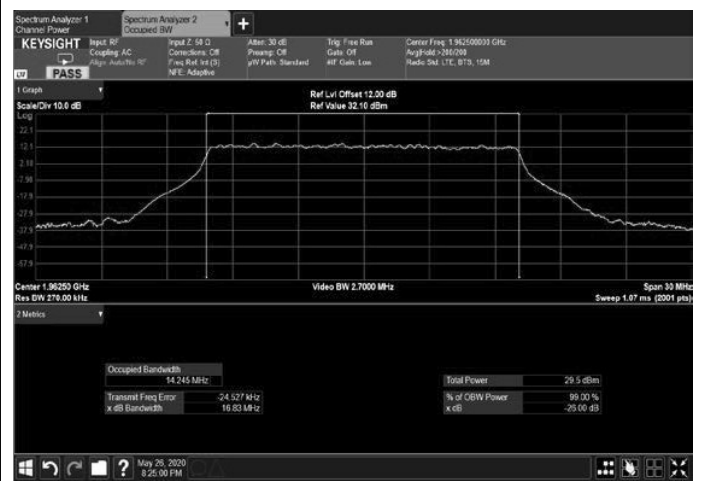
Figure 256: 64QAM 15MHz B.W.; 1962.5MHz, 15kHz Output
