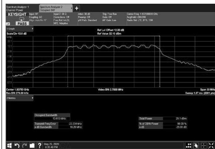
Figure 221: 16QAM 15MHz B.W.; 1937.5MHz, 30kHz Output
