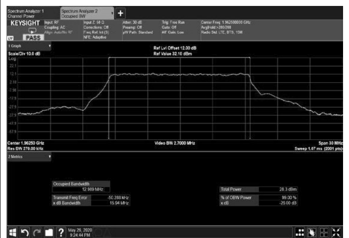
Figure 258: 64QAM 15MHz B.W.; 1962.5MHz, 60kHz Output
