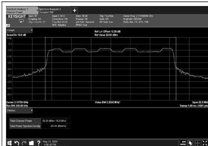
Figure 121: 16QAM 15MHz B.W.; 2117.5MHz, 15kHz
