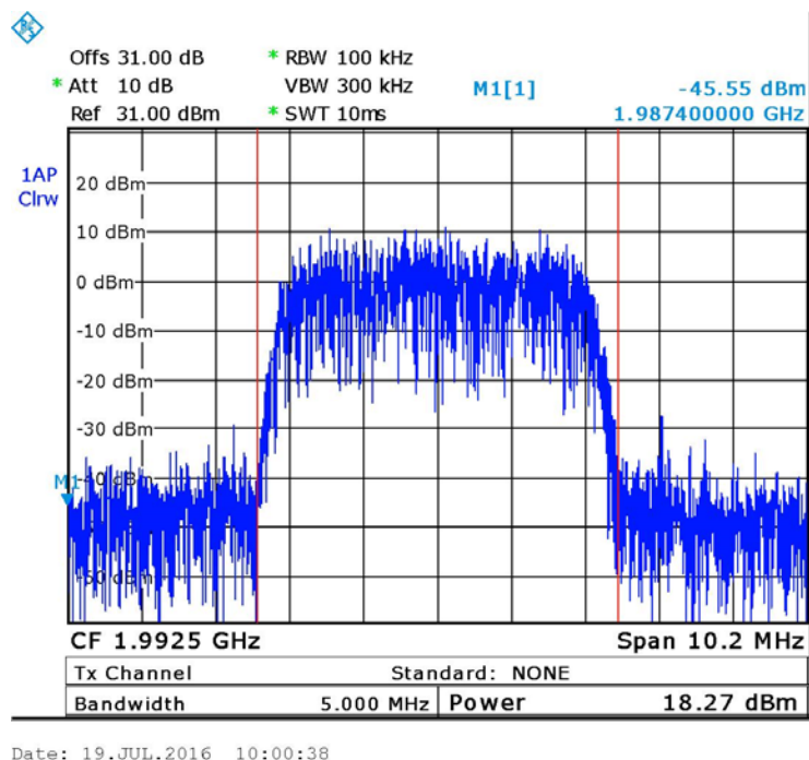
Figure 19. — W-CDMA - 1992.5 MHz
