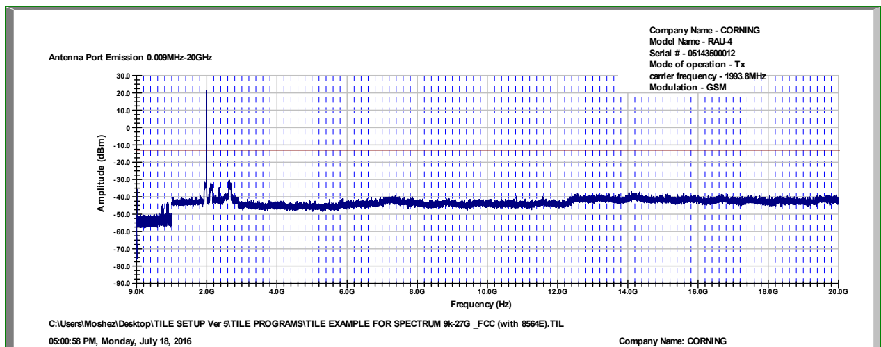
Figure 46. — GSM - 1993.8 MHz
