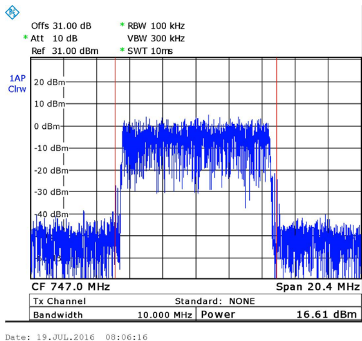
Figure 15. — 16QAM 747 MHz
