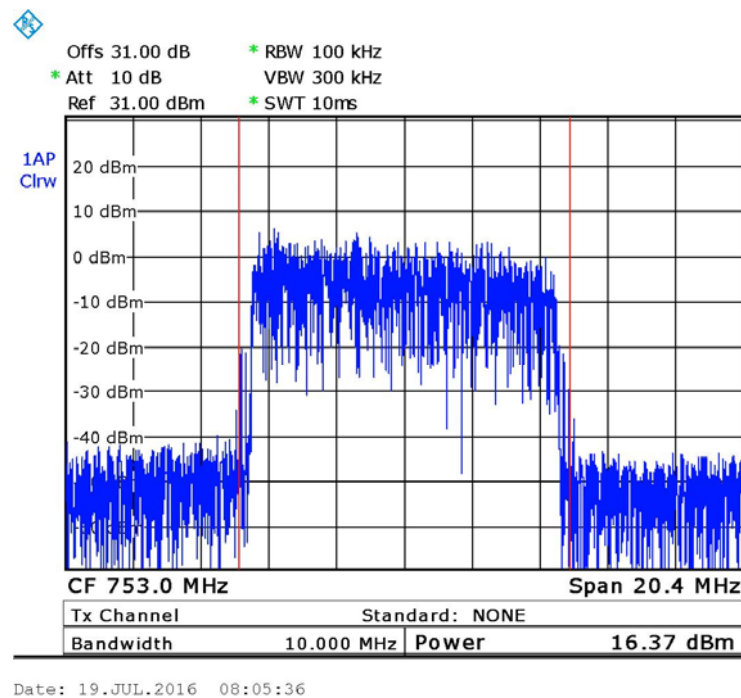
Figure 16. — 16QAM 753 MHz
