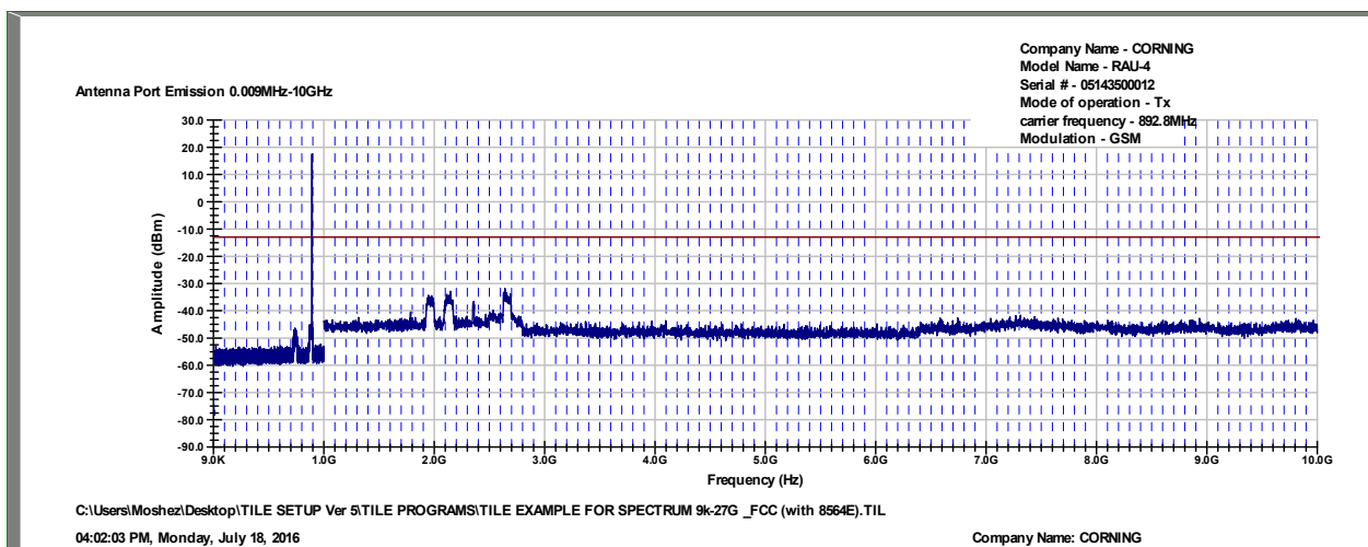
Figure 46. — GSM -892.8 MHz
