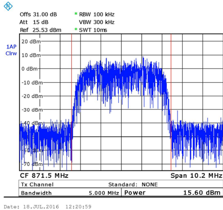
Figure 17. — W-CDMA - 871.5 MHz
