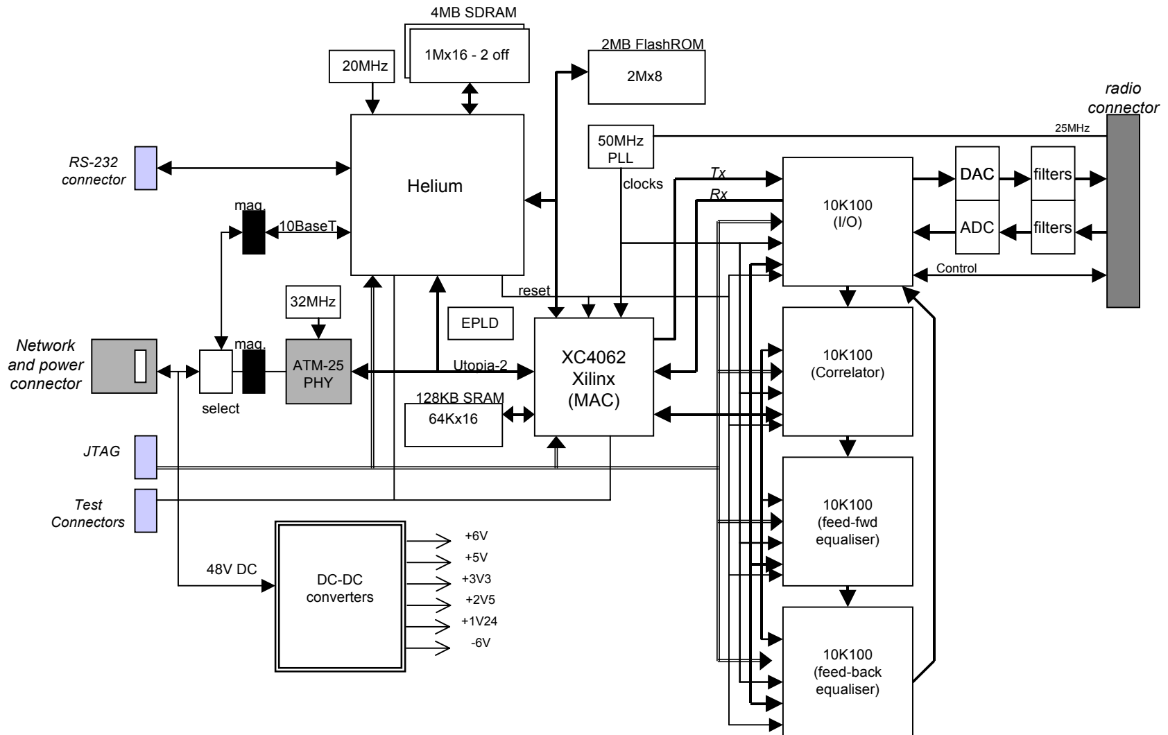
Figure 2 : System Motherboard
