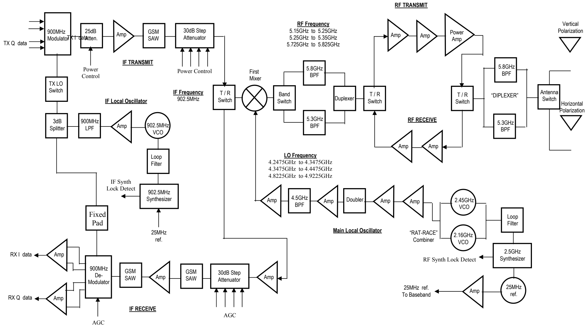
Figure 1 : Radio Transceiver Module.
