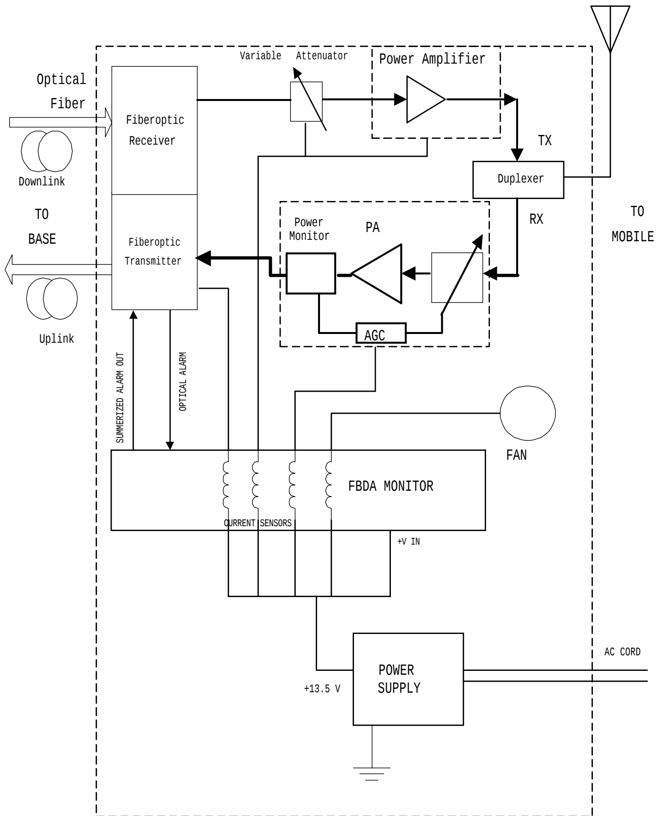
FBDA-PCS-A-10W ELELCTRICAL SCHEMATICS
