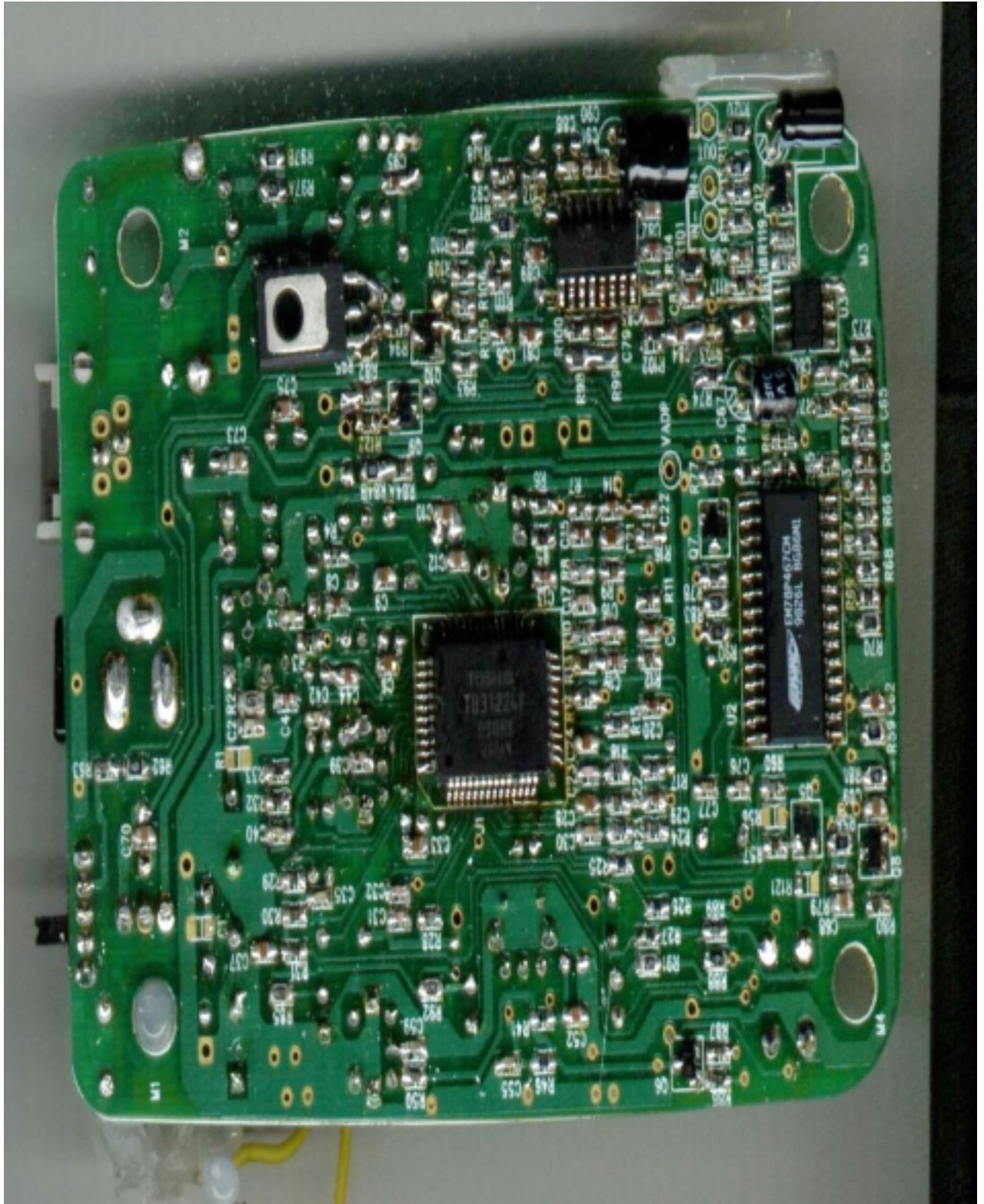
B. Base main board solder side
