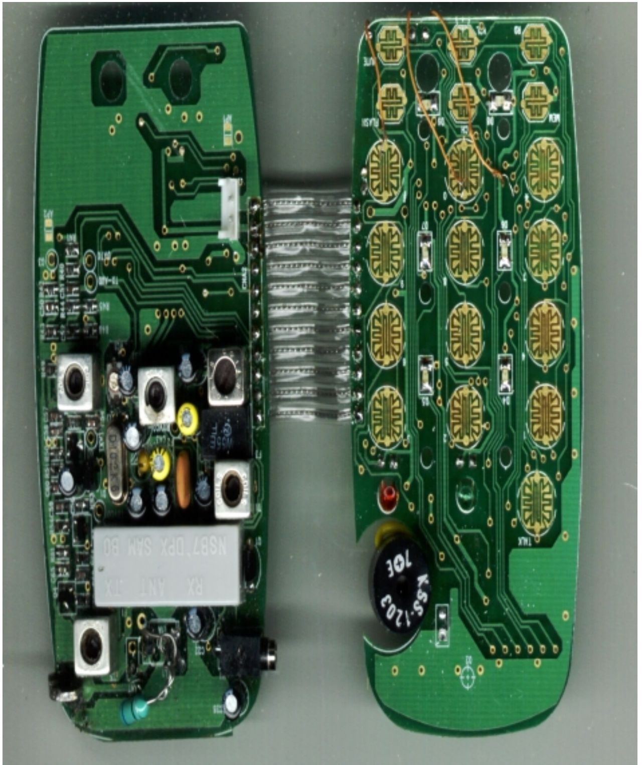
C. Handset main board component side
