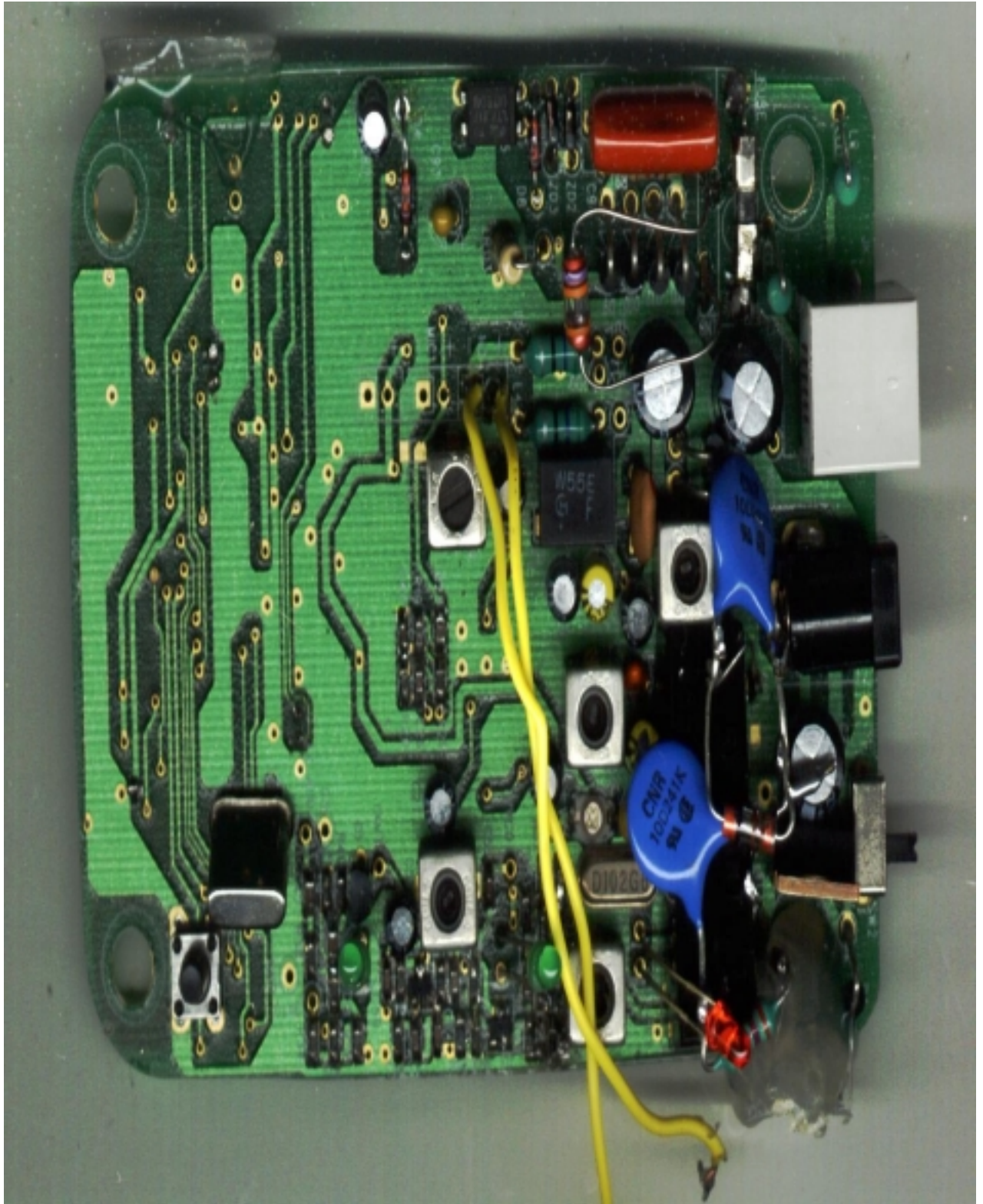
A. Base main board component side
