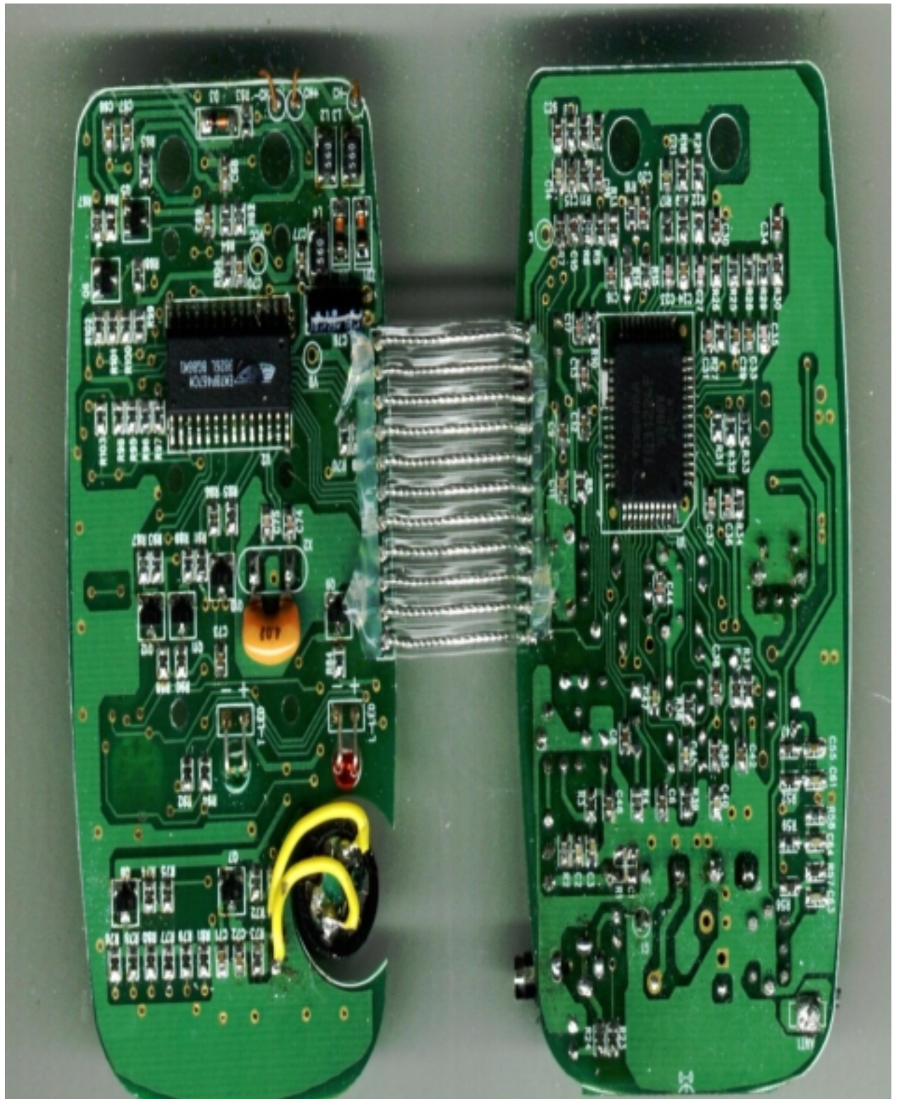
D. Handset main board solder side
