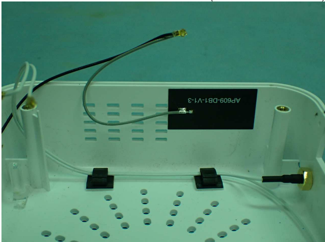
Figure 18 Internal View (WLAN / BT Antenna View)
