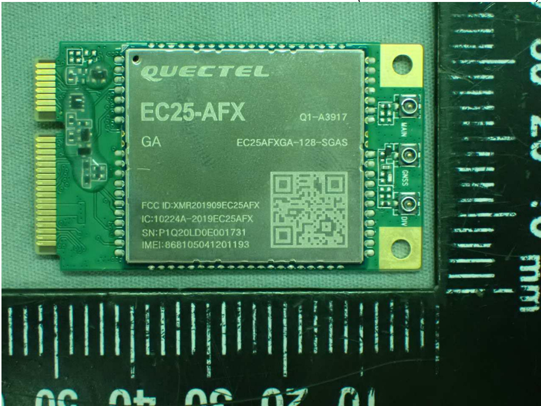
Figure 23 Internal View (LTE Module / Front View)
