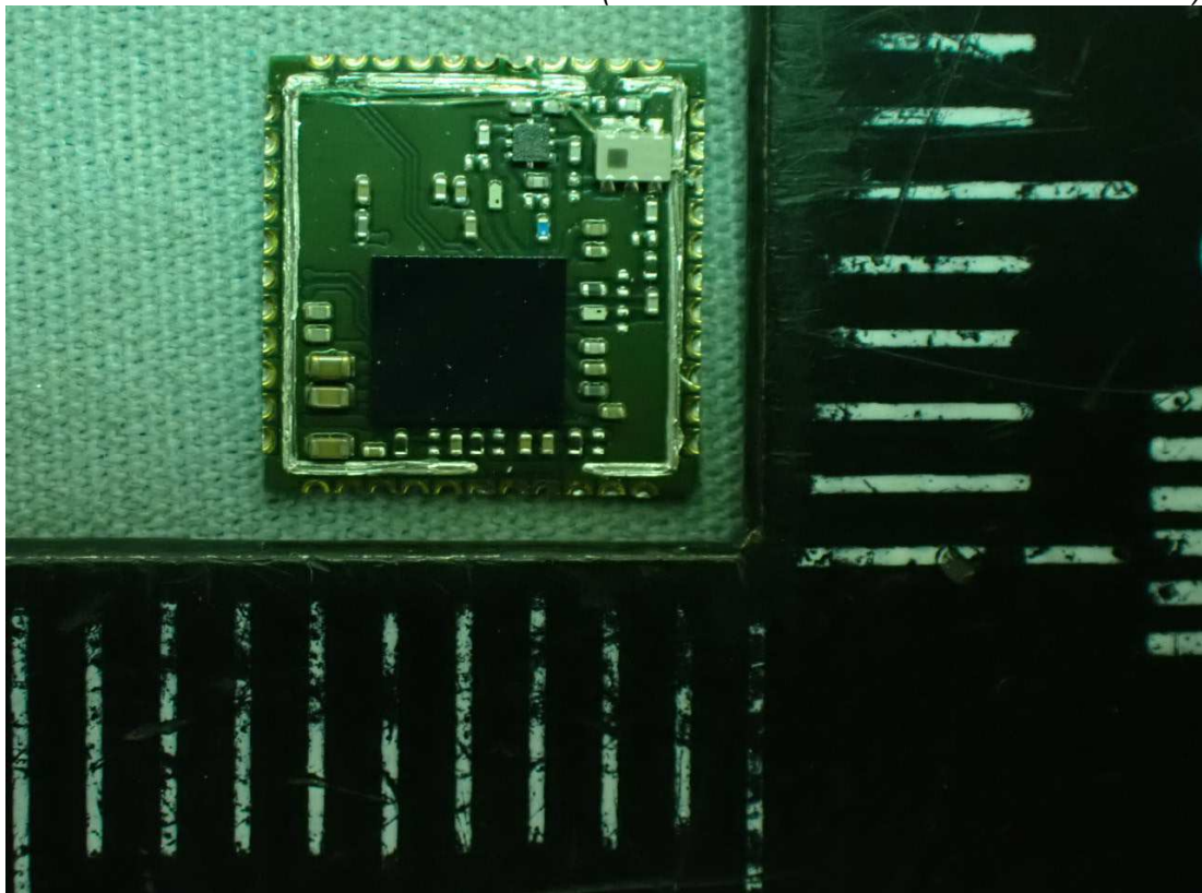
Figure 26 Internal View (WLAN / BT Combo Card / Front View)
