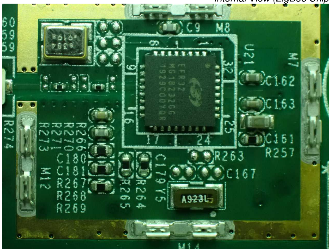
Figure 30 Internal View (ZigBee Chip)
