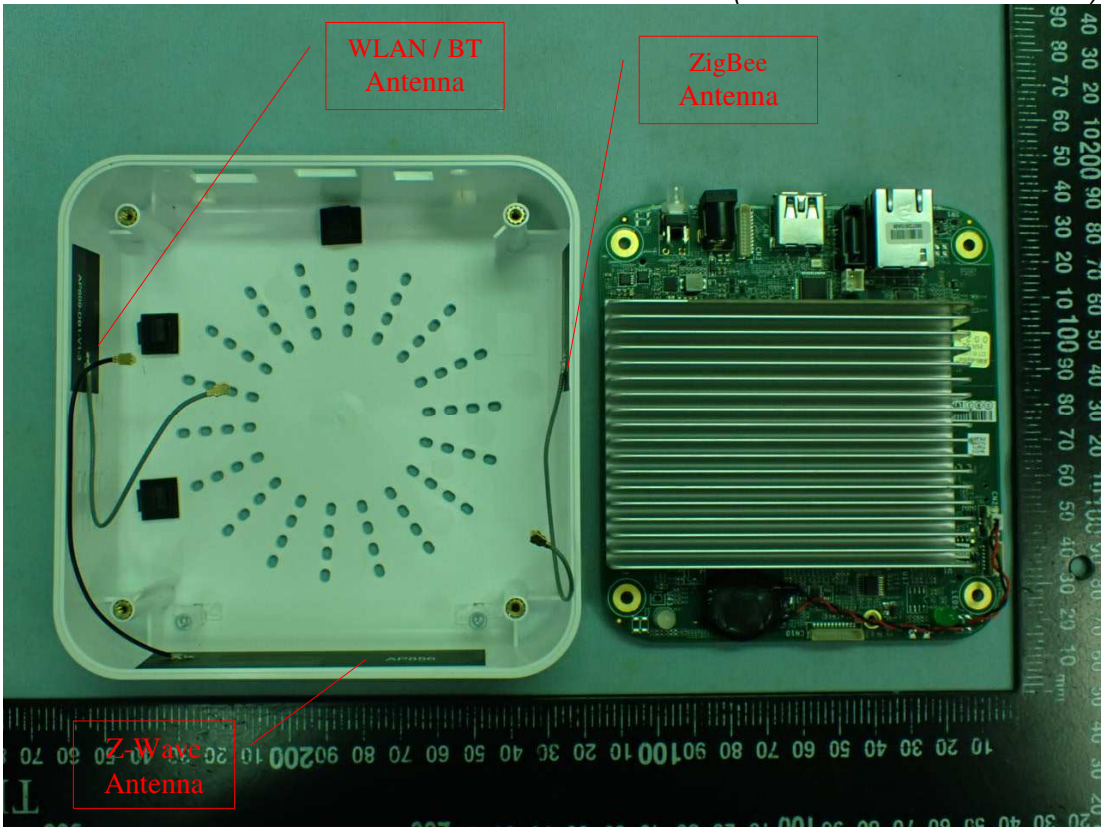
Figure 35 Internal View (Removed Internal Board)
