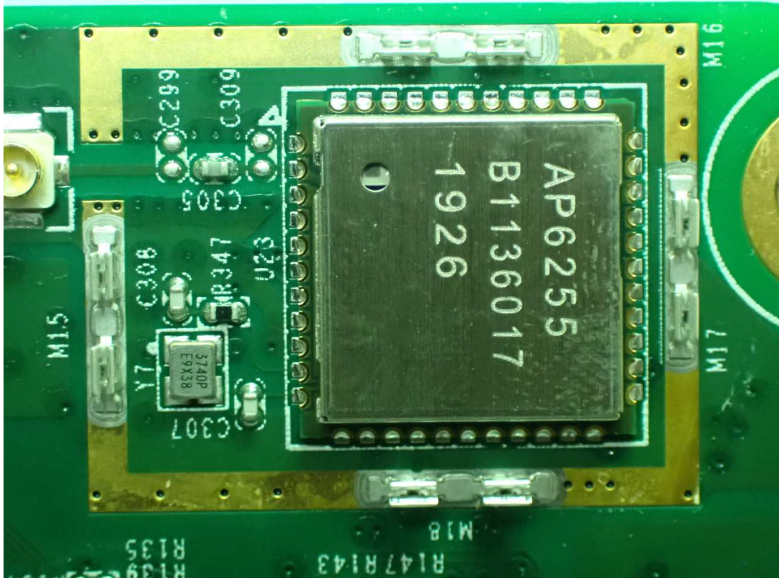
Figure 25 Internal View (WLAN / BT Combo Card)
