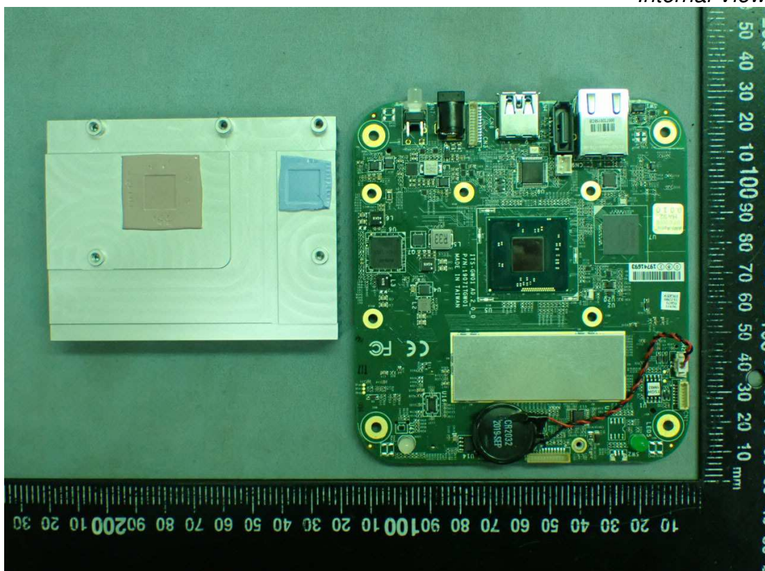
Figure 20 Internal View
