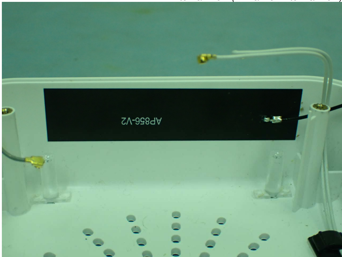
Figure 19 Internal View (Z-Wave Antenna View)
