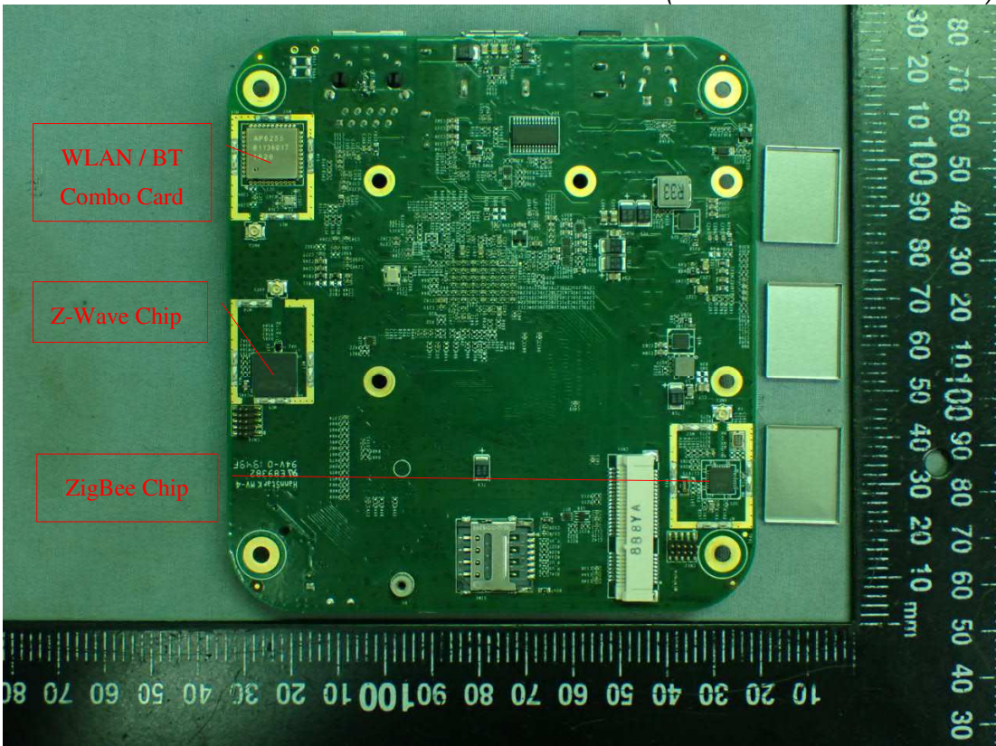
Figure 22 Internal View (Main Board / Front View)
