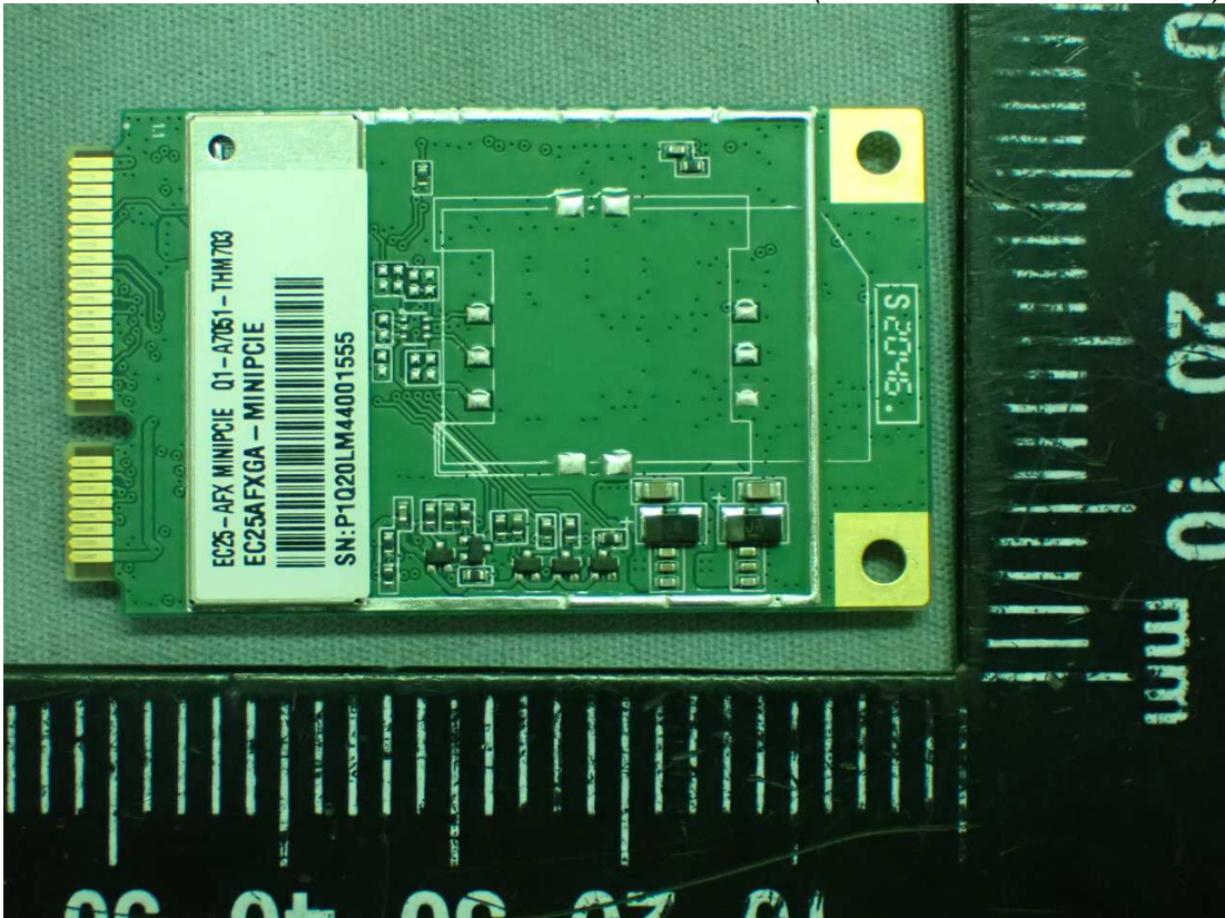
Figure 24 Internal View (LTE Module / Back View)
