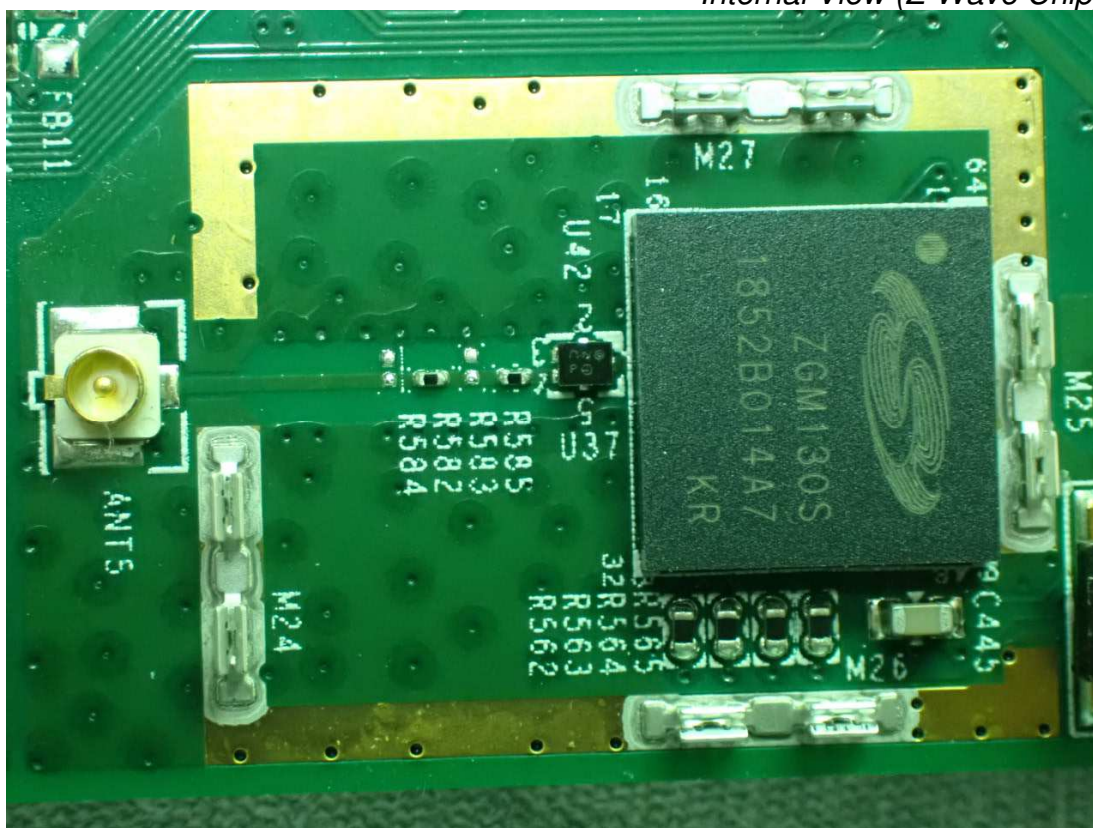
Figure 29 Internal View (Z-Wave Chip)
