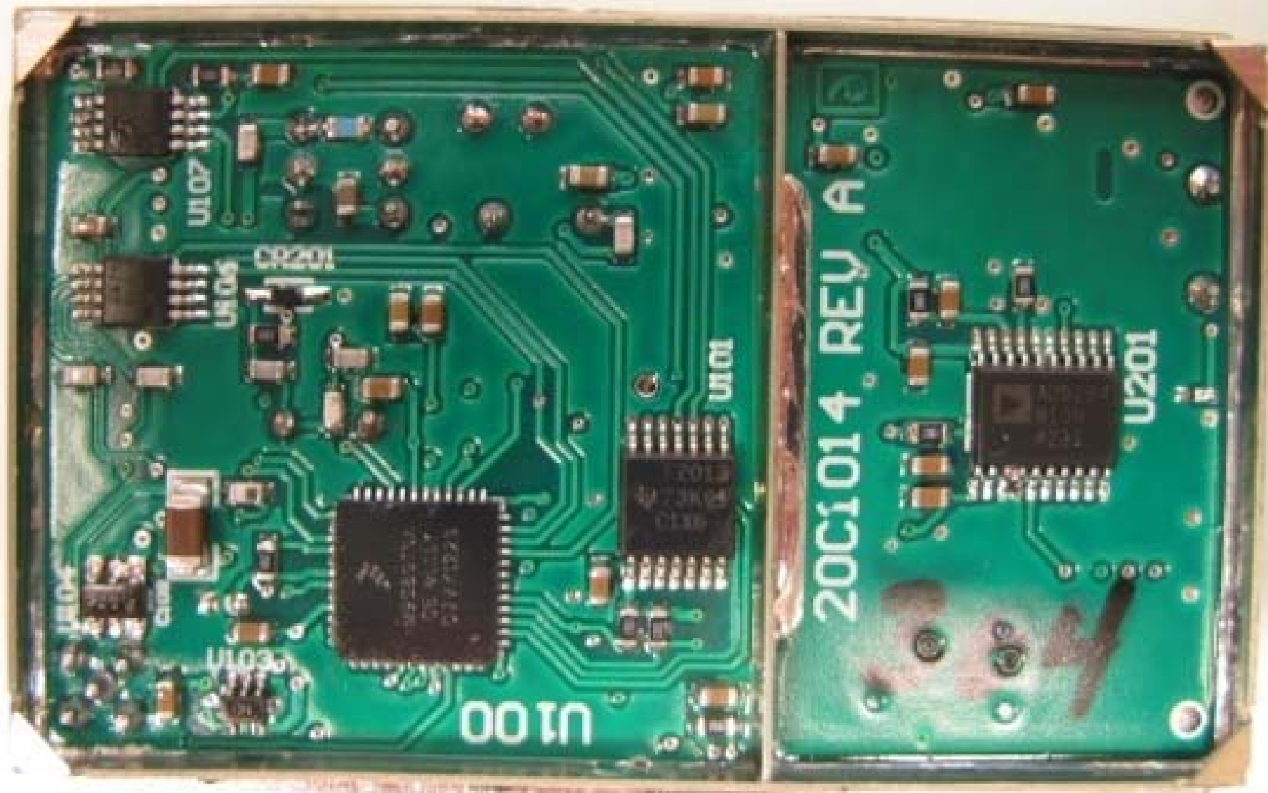
MCDR bottom pcb with shield
