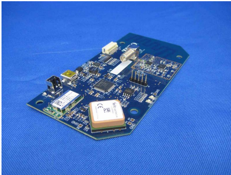
Component Side; View 1
