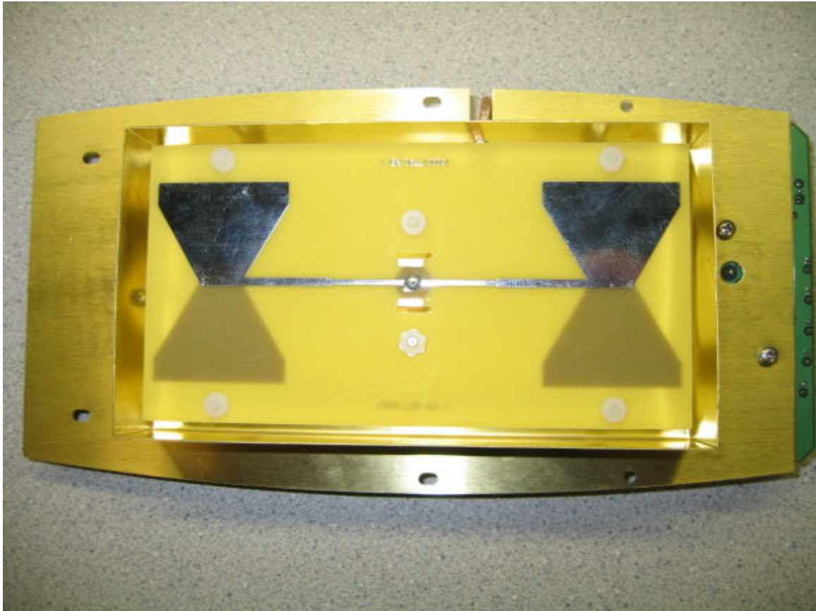
Re-Rad Antenna, Internal
