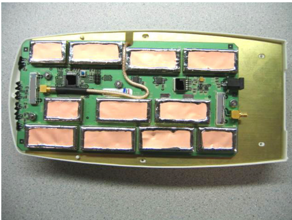
In-Home Repeater, Internal
