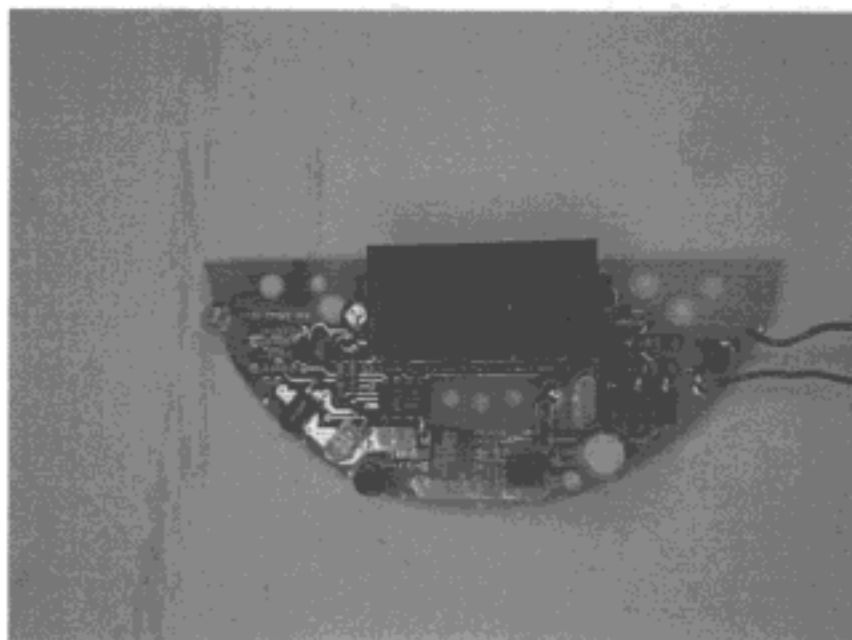
Figure 2 - Component Side of EUT
