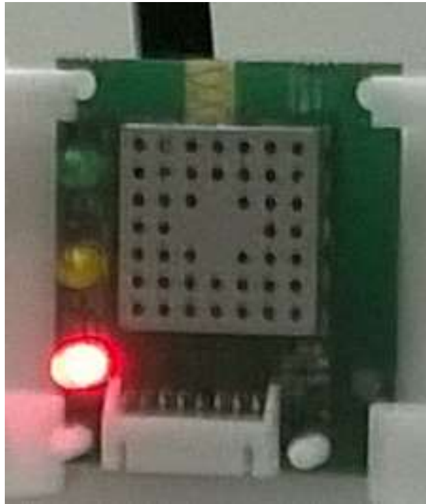
Figure 2 - RF module with shield
