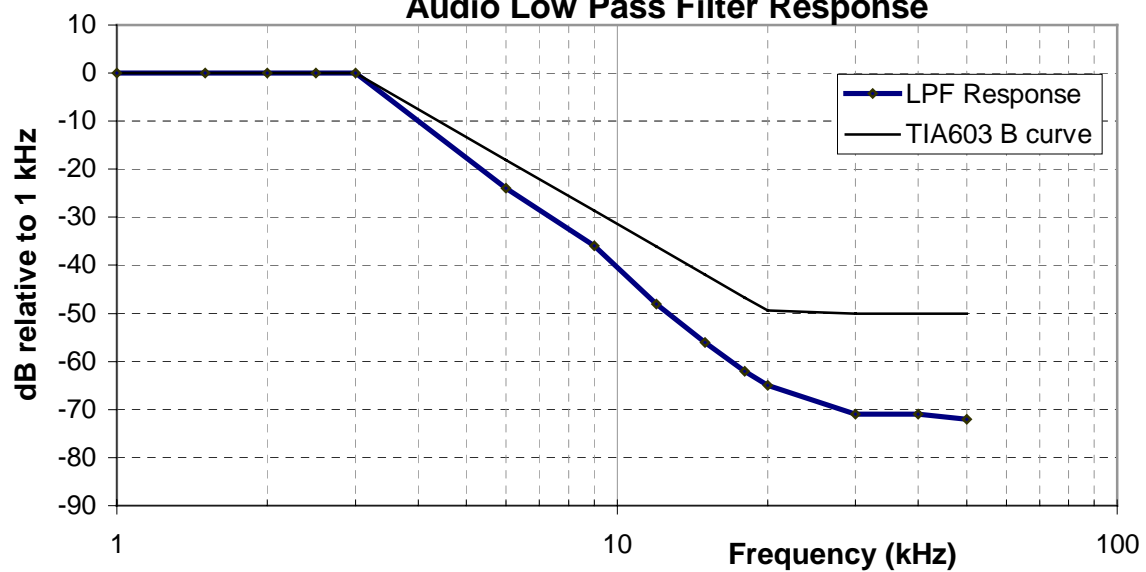
Audio Low Pass Filter Response
