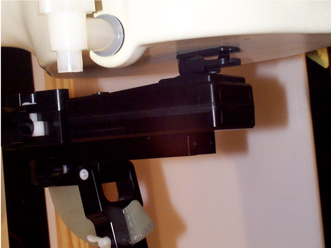
SAR Testing Against the Flat Phantom
