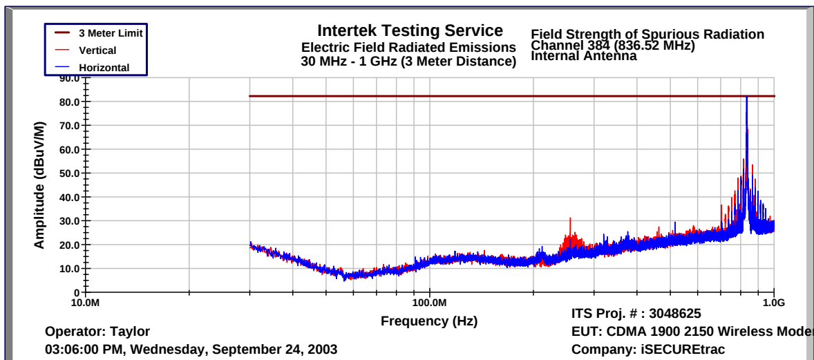
Figure 8-1: Field Strength of Spurious Radiation (30 MHz – 1 GHz), CDMA 800 Channel 384, 777, and 1013 (Internal Antenna)
