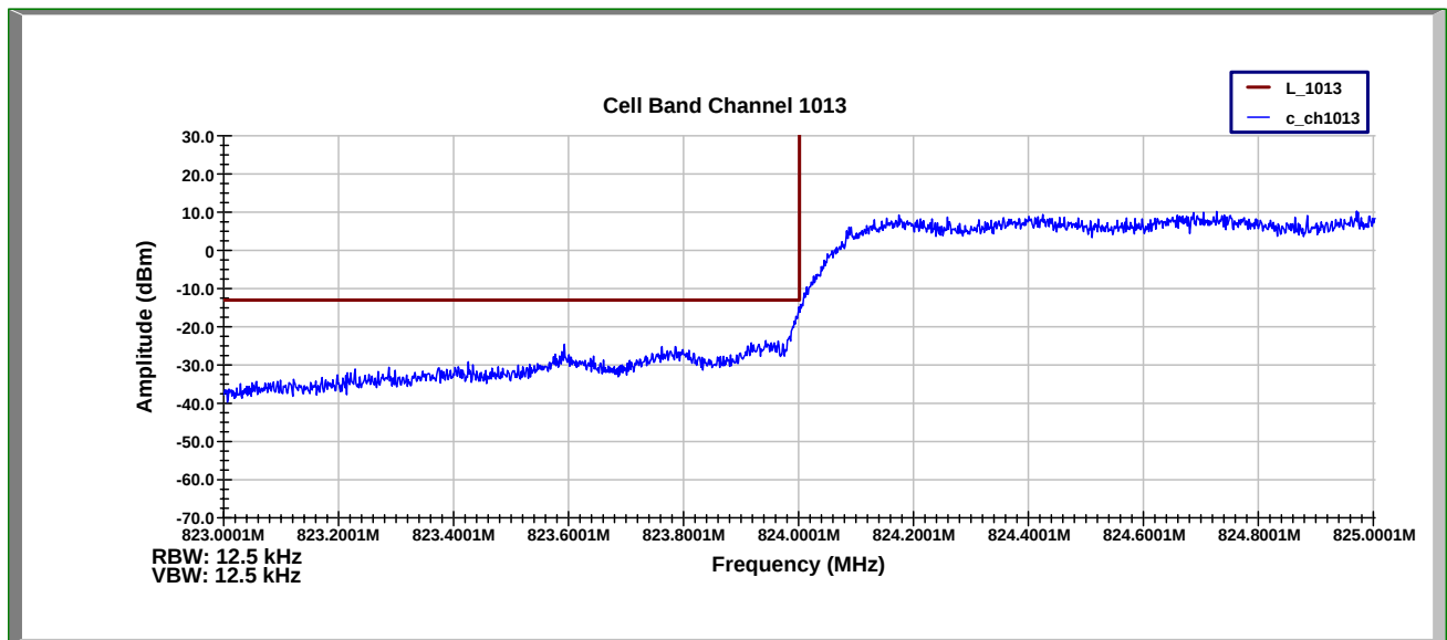
Figure 7-7: Emissions within 1 MHz of band edge, CDMA 800 Channel 1013
