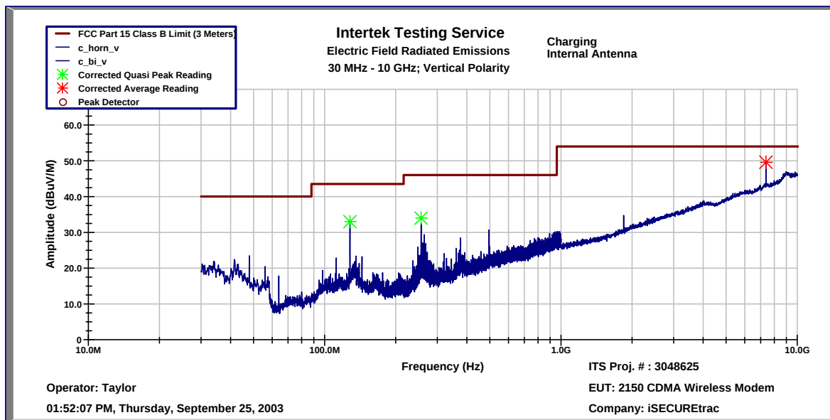
Figure 10-4 FCC §15.109Worse Case Receiver Spurious Emission (Vertical – Internal Antenna, Charging)
