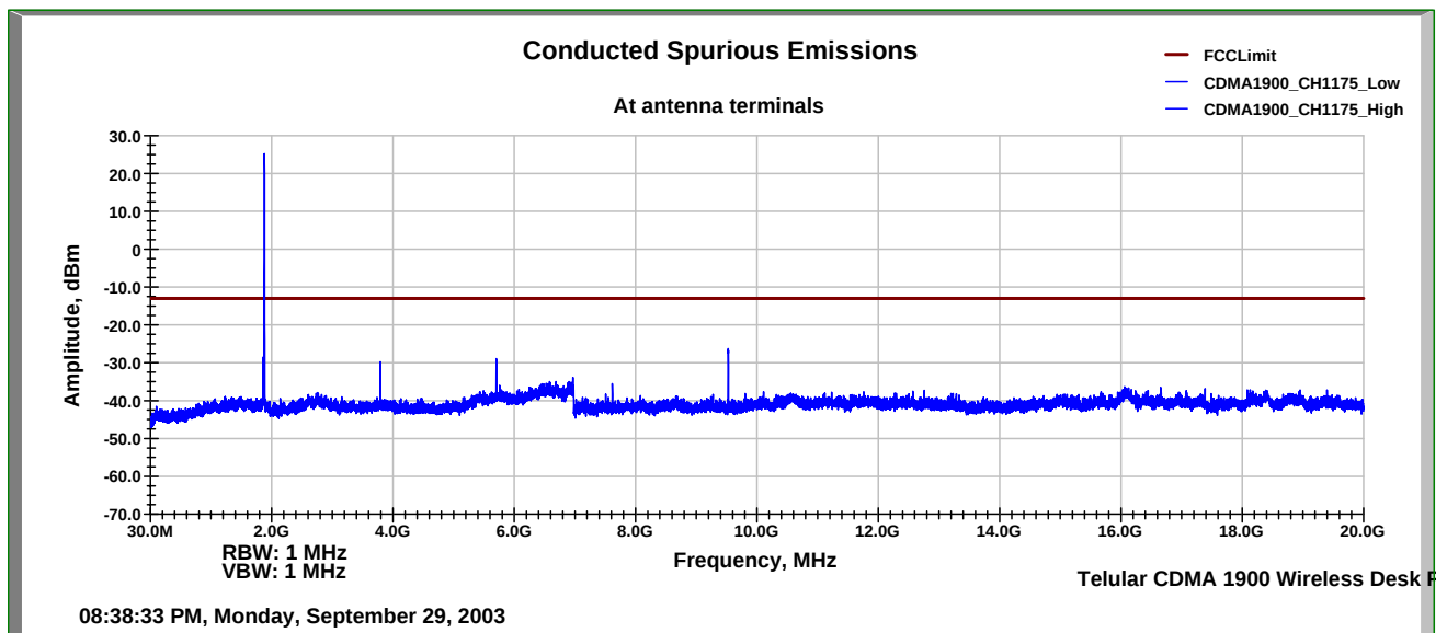
Figure 7-6: Out of band emissions at antenna terminals – CDMA1900 Channel 1175
