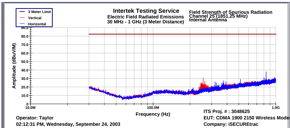
Figure 8-4: Field Strength of Spurious Radiation (30 MHz – 1 GHz), CDMA 1900 Channel 25, 600, and 1175 (Internal Antenna)
