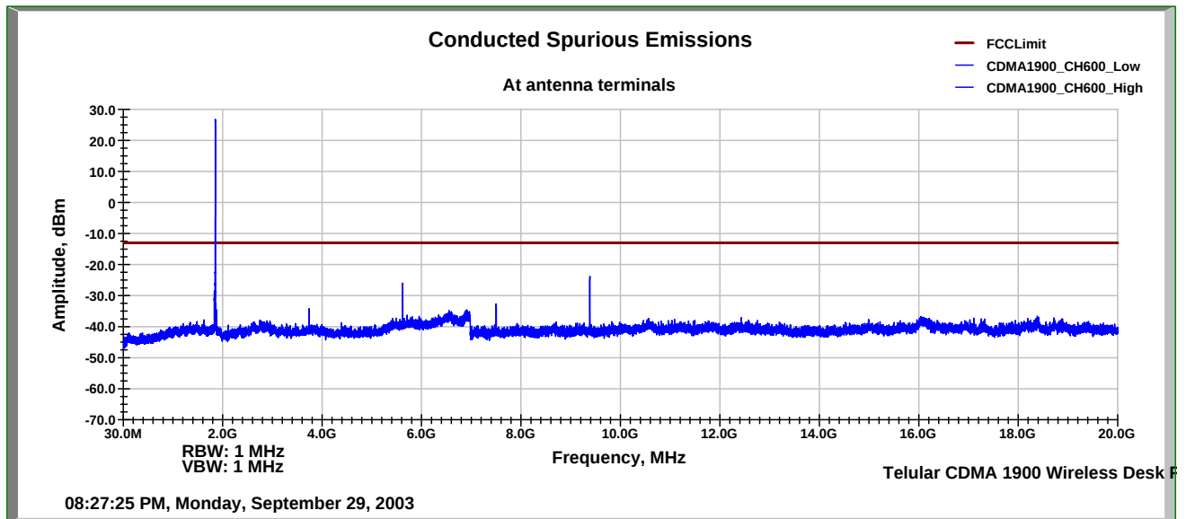
Figure 7-5: Out of band emissions at antenna terminals – CDMA1900 Channel 600
