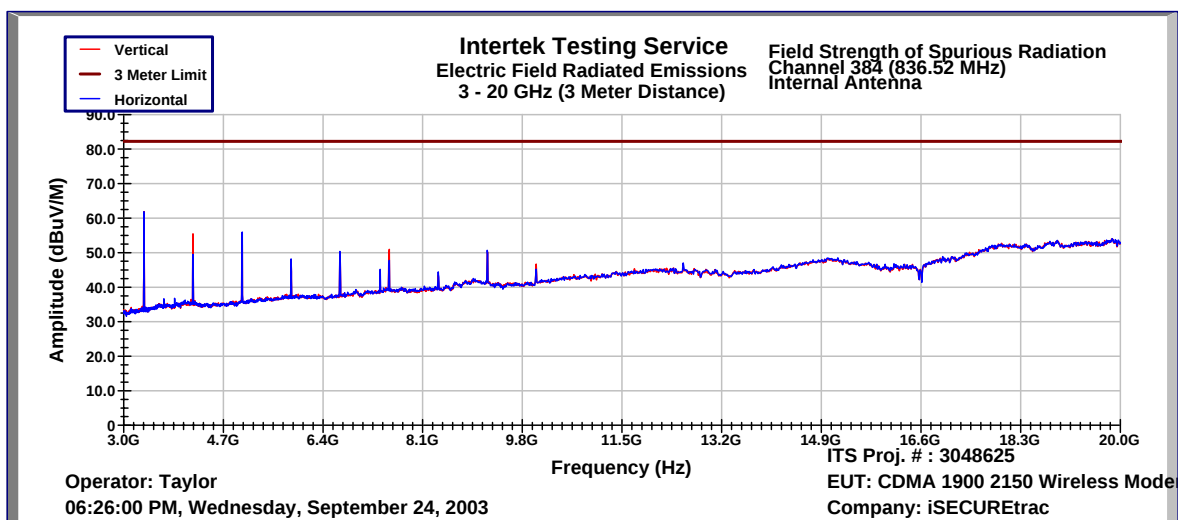
Figure 8-3: Field Strength of Spurious Radiation (3GHz – 20GHz), CDMA 800 Channel 384, 777, and 1013 (Internal Antenna)
