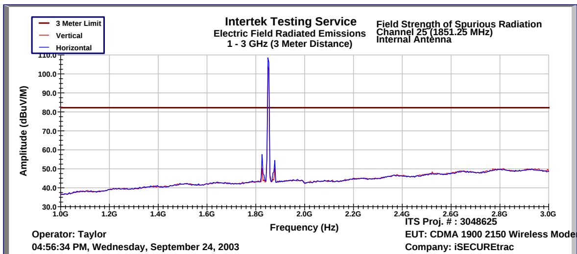
Figure 8-5: Field Strength of Spurious Radiation (1 GHz – 3 GHz), CDMA 1900 Channel 25, 600, and 1175 (Internal Antenna)
