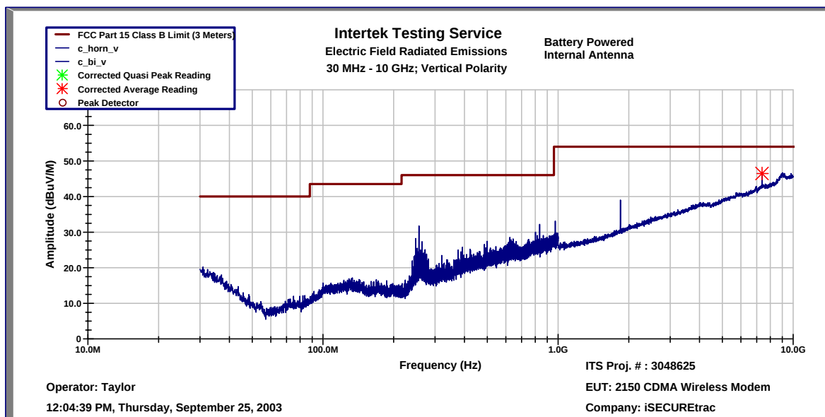
Figure 10-2 FCC §15.109Worse Case Receiver Spurious Emission (Vertical – Internal Antenna, Battery Powered)
