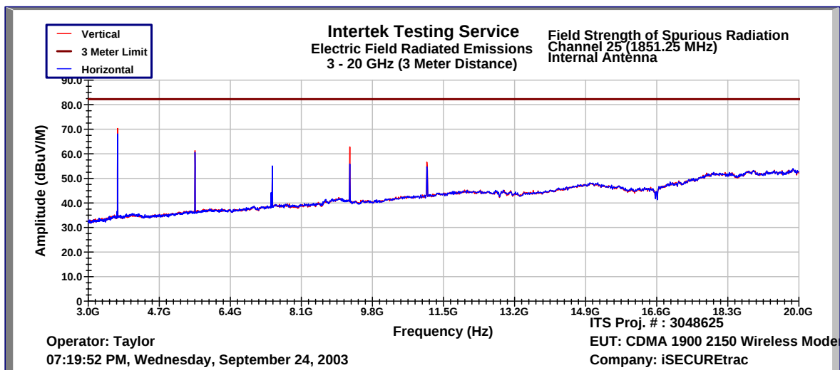
Figure 8-6: Field Strength of Spurious Radiation (3GHz – 20GHz), CDMA 1900 Channel 25, 600, and 1175 (Internal Antenna)
