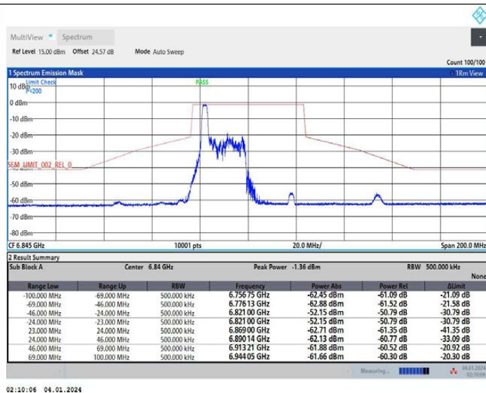
11AX40MIMO Ant2 6845 52Tone RU37
