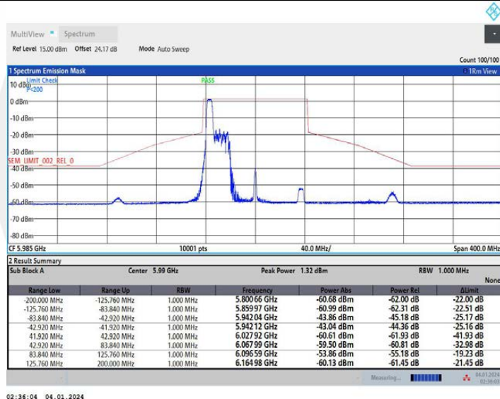
11AX80MIMO Ant2 5985 106Tone RU53
