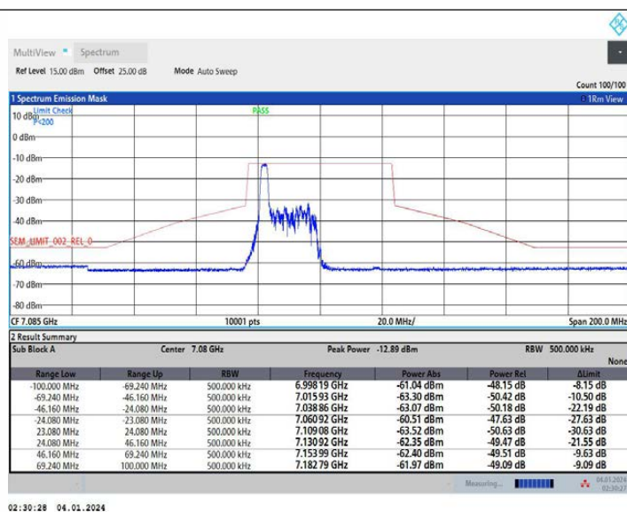
11AX40MIMO Ant2 7085 52Tone RU37
