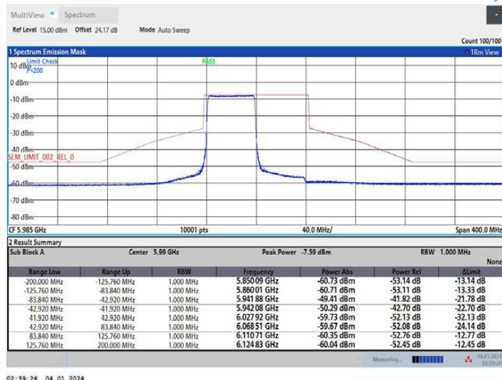
11AX80MIMO Ant1_5985_26Tone_RU0
