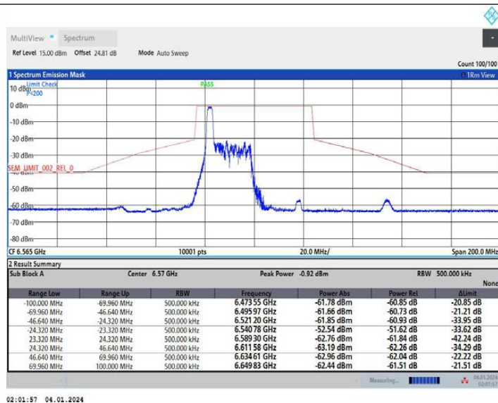
11AX40MIMO Ant2 6565 52Tone RU37
