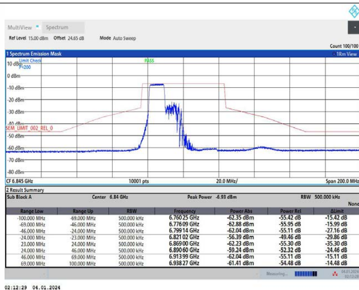
11AX40MIMO Ant1 6845_242Tone RU61
