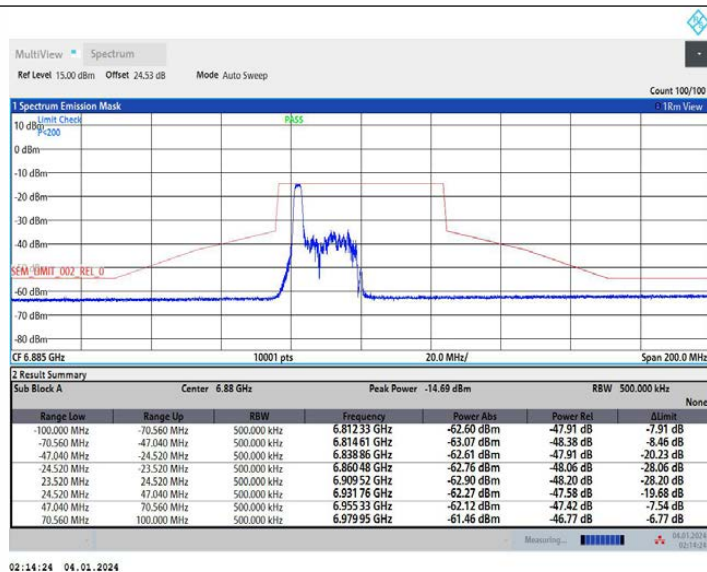
11AX40MIMO Ant2 6885 52Tone RU37
