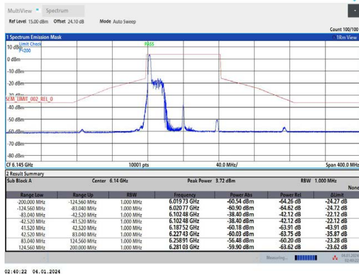
11AX80MIMO Ant2 6145 52Tone RU37
