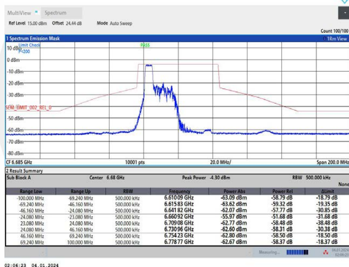
11AX40MIMO Ant2 6685 106Tone RU53
