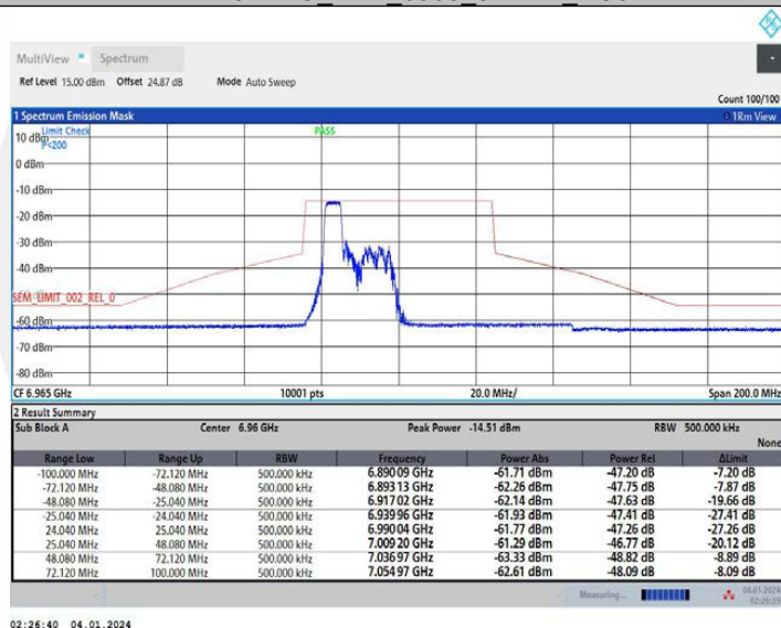
11AX40MIMO Ant2 6965 106Tone RU53
