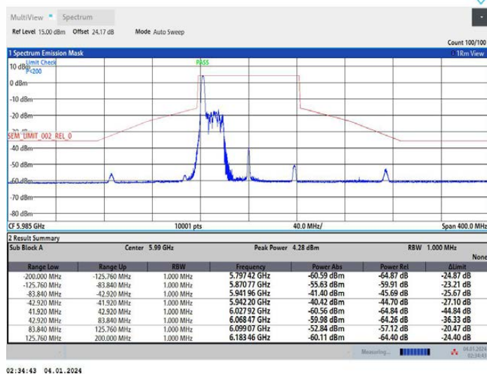
11AX80MIMO Ant2 5985 52Tone RU37
