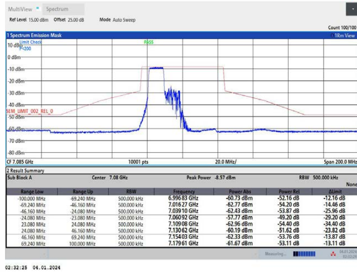
11AX40MIMO Ant2 7085_242Tone RU61
