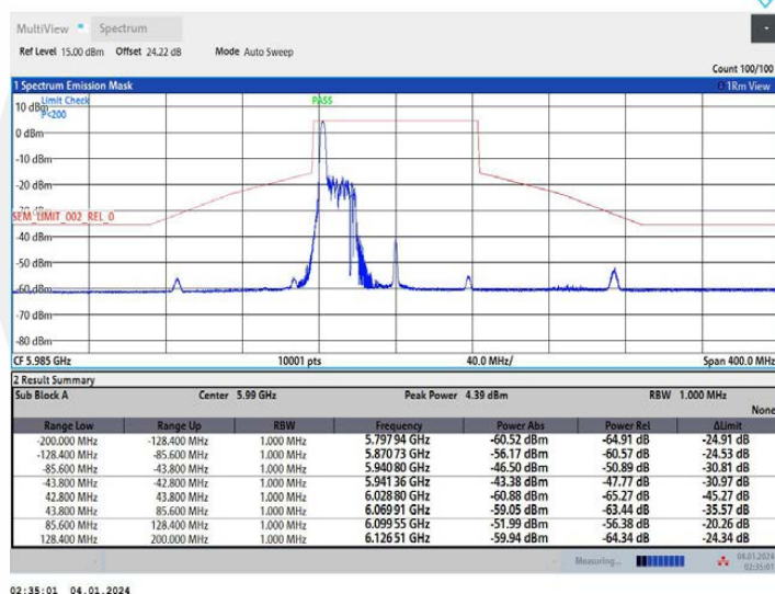
11AX80MIMO Ant1_5985_52Tone_RU37
