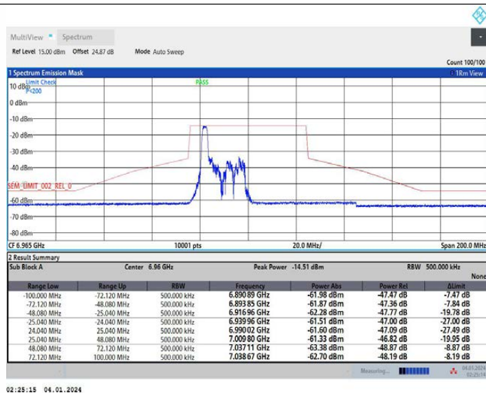
11AX40MIMO Ant2 6965 52Tone RU37
