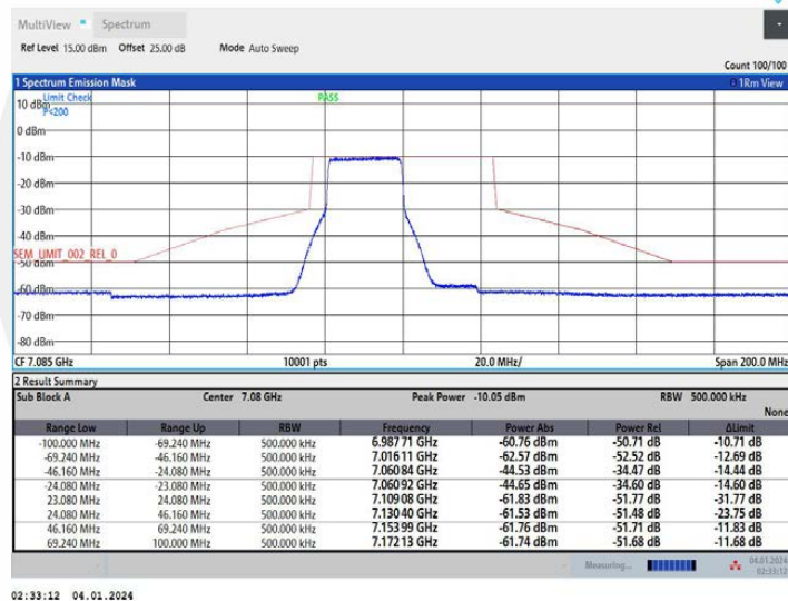
11AX40MIMO Ant1 7085_26Tone RU0
