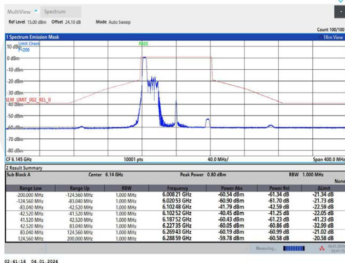
11AX80MIMO Ant2 6145 106Tone RU53
