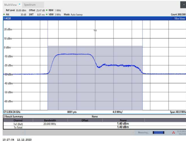
11AX20MIMO Ant1_6855_26Tone_RU0
