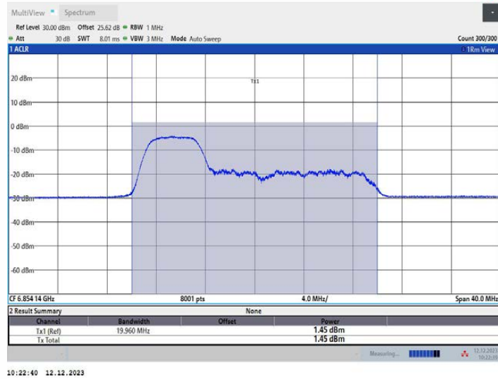
11AX20MIMO Ant1 6855_106Tone RU53
