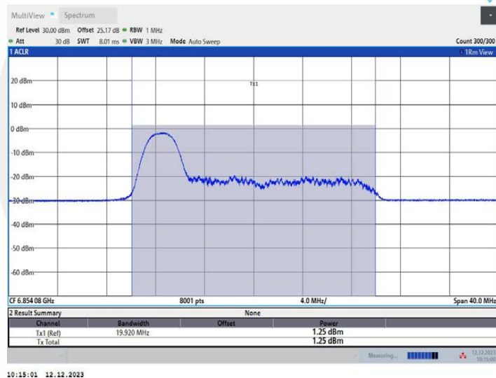
11AX20MIMO Ant1_6855_52Tone_RU37
