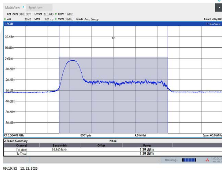
11AX20MIMO Ant1_6535_52Tone_RU37
