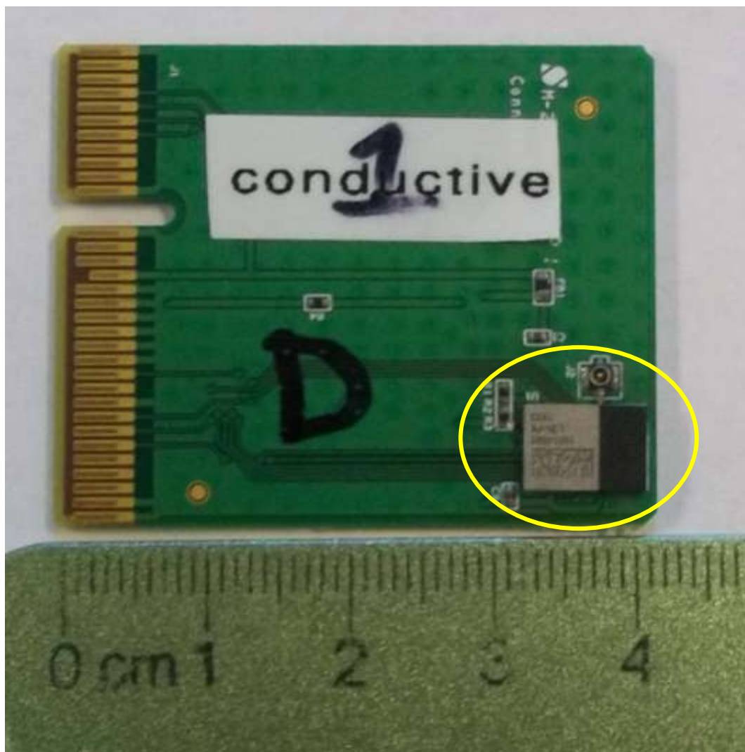
Figure 3. EUT, Close-up of Module and Antenna Area
