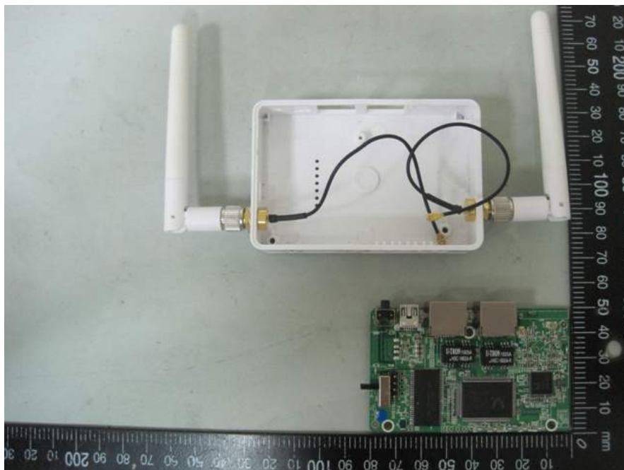
EUT 1. EUT with Dipole Antenna
