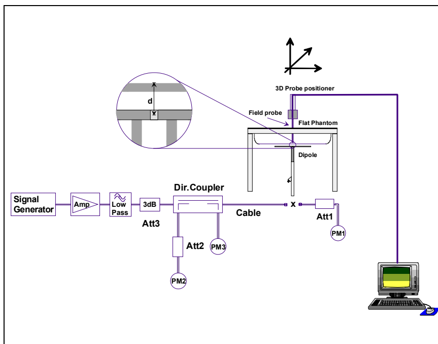
Figure 1. System Performance Check Setup Diagram
