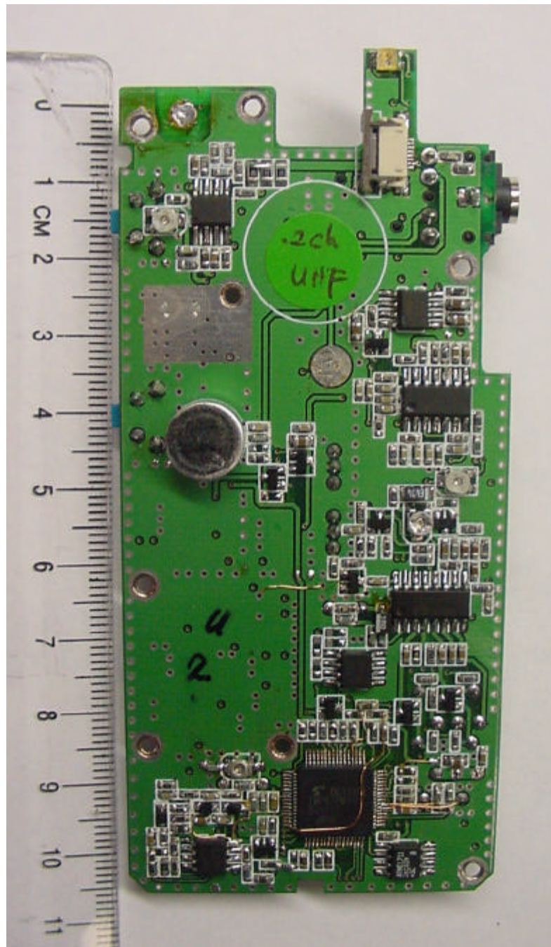
PHOTOGRAPH 5: FRONT VIEW OF PCB
