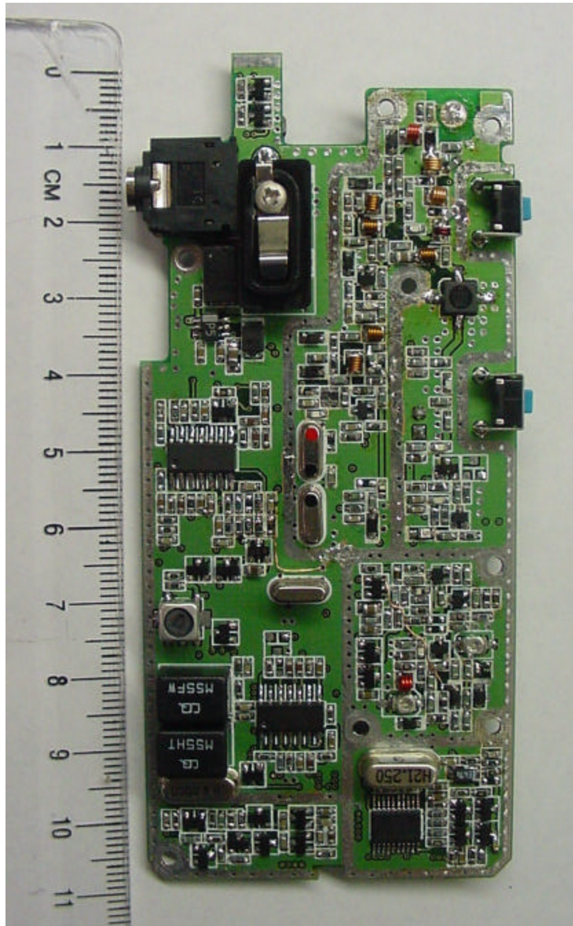
PHOTOGRAPH 6: BACK VIEW OF PCB
