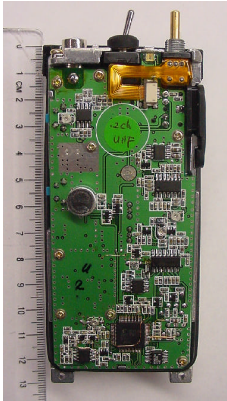
PHOTOGRAPH 7: FRONT VIEW OF PCB INSIDE CHASSIS
